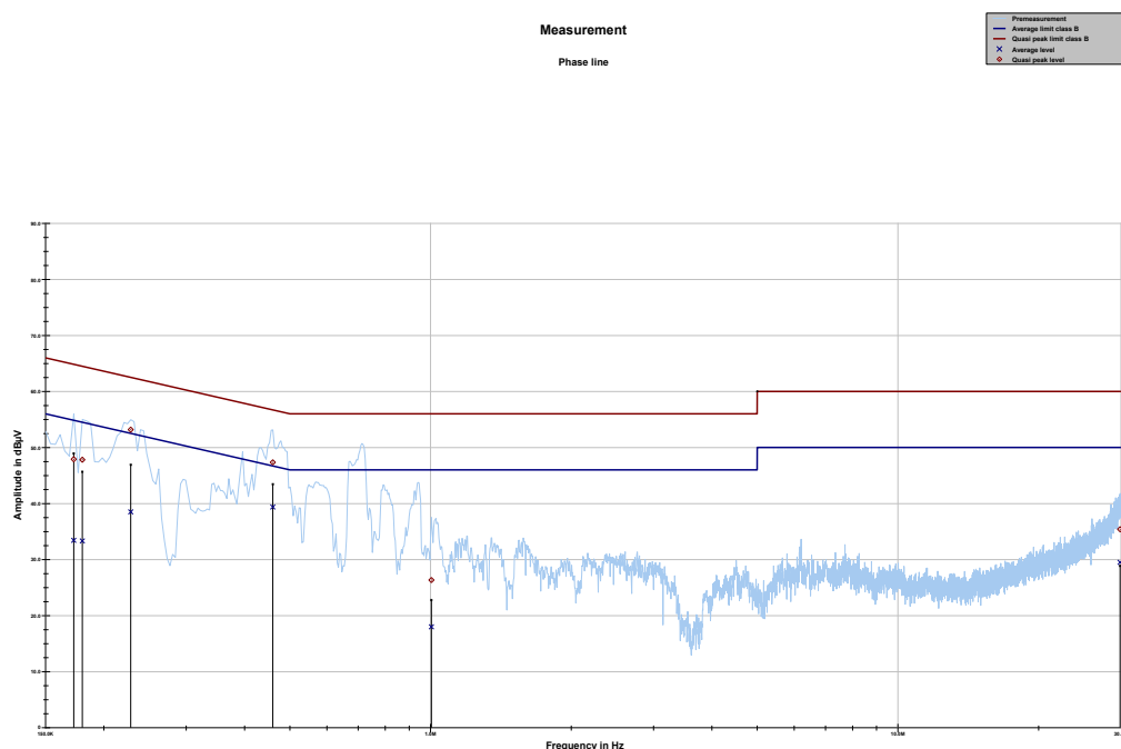
Plot 3: 150 kHz to 30 MHz, phase line (120 VAC)
