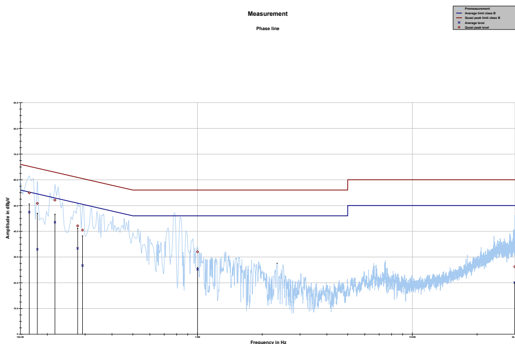
Plot 1: 150 kHz to 30 MHz, phase line (240 VAC)
