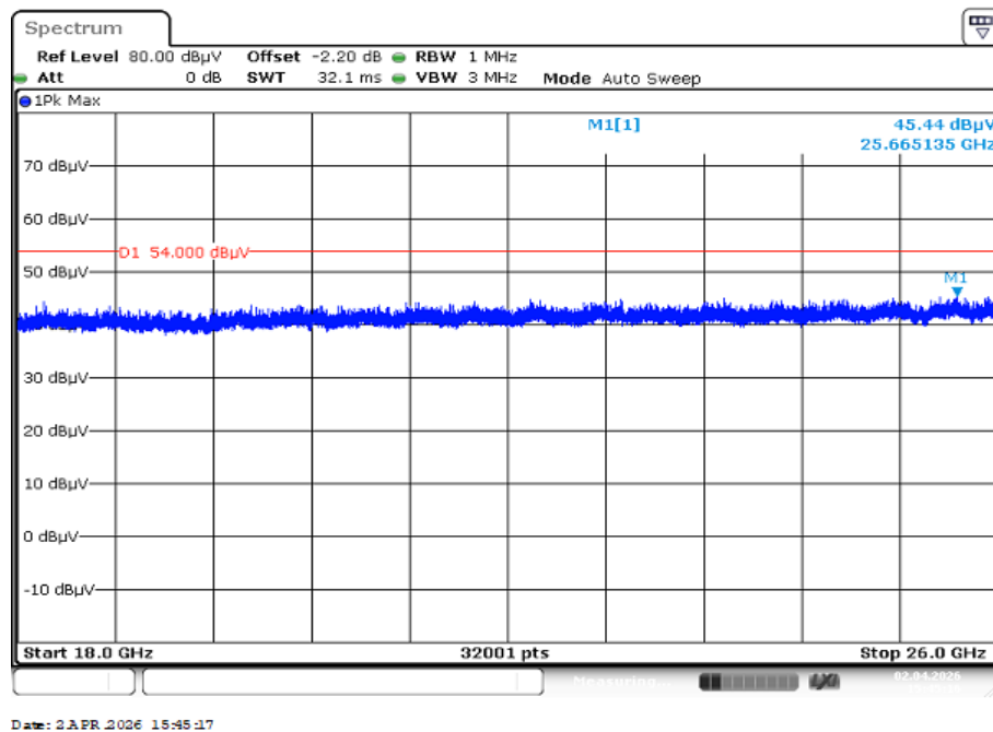
Plot 4: 18 GHz to 26 GHz, TX mode, vertical & horizontal polarization, valid for all modes
