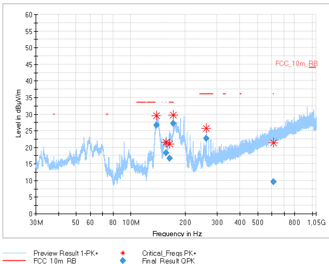
Plot 1: 30 MHz to 1 GHz, TX mode, vertical & horizontal polarization (valid for all channels)
