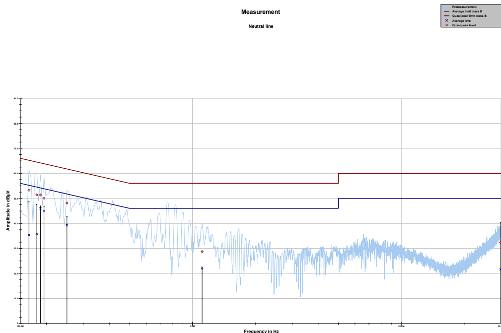
Plot 2: 150 kHz to 30 MHz, neutral line (240 VAC)
