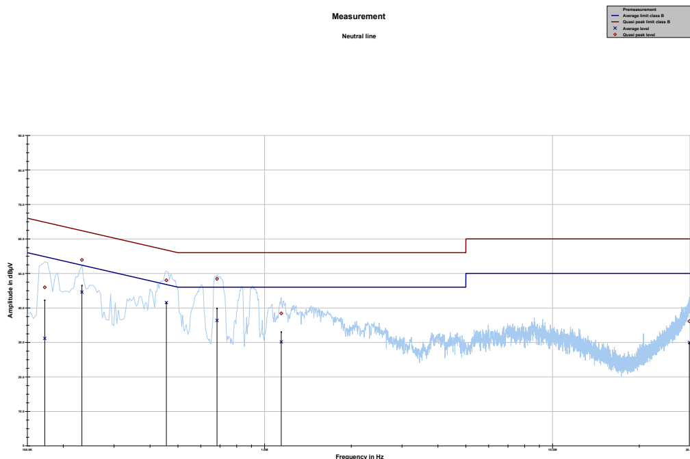
Plot 4: 150 kHz to 30 MHz, neutral line (120 VAC)
