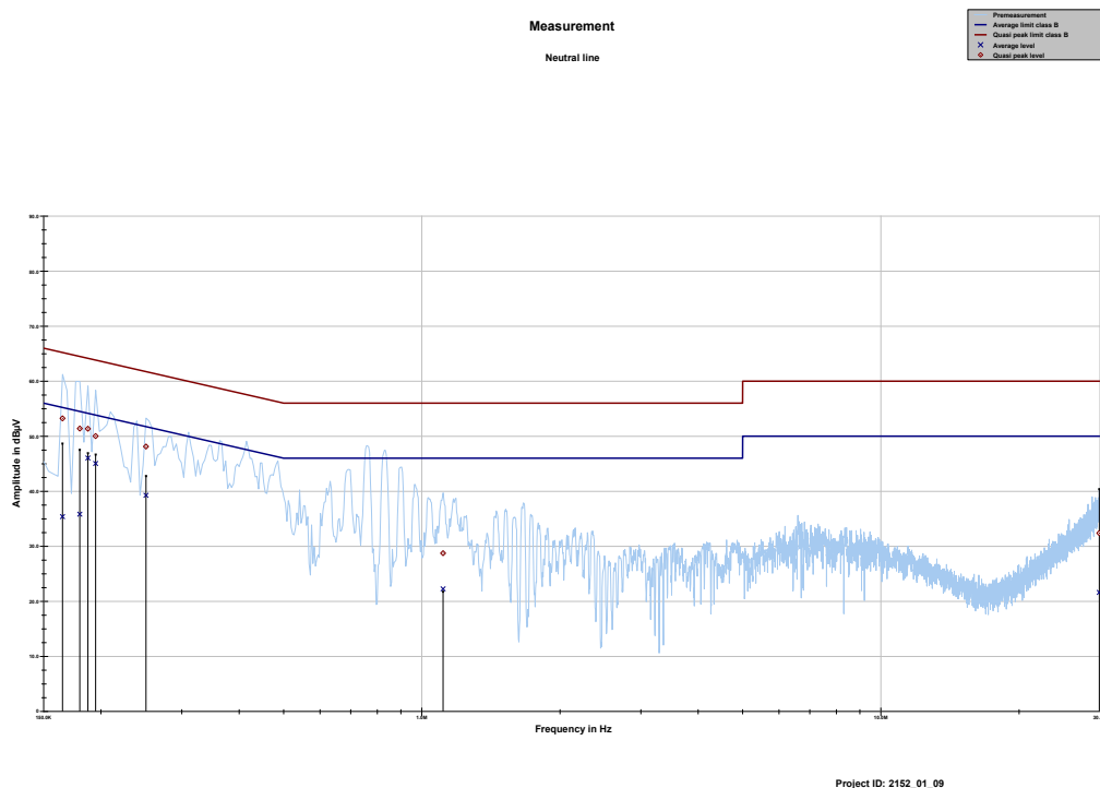
Plot 2: 150 kHz to 30 MHz, neutral line (240 VAC)
