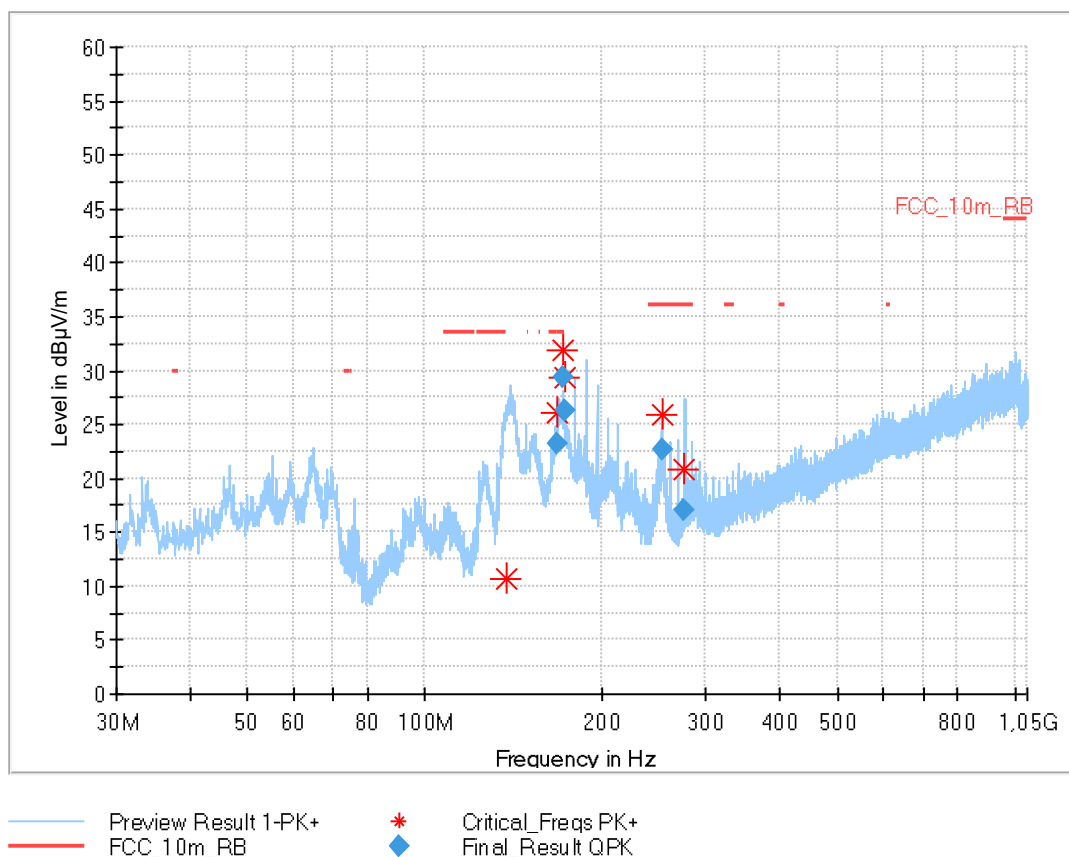
Plot 2: 30 MHz to 1 GHz, TX mode, vertical & horizontal polarization, 2 Msps, valid for all channels
