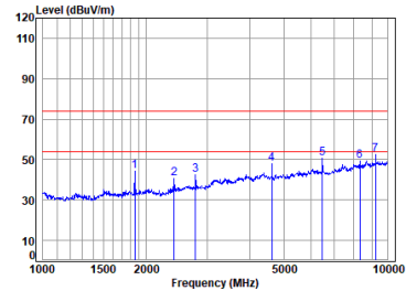
Sub_TX_CH_H_Vertical
