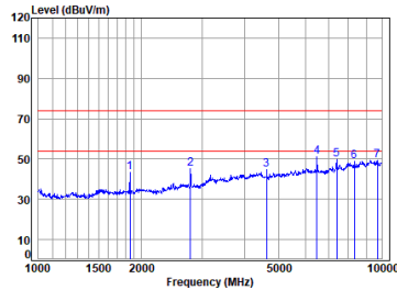
Sub_TX_CH_H_Horizontal
