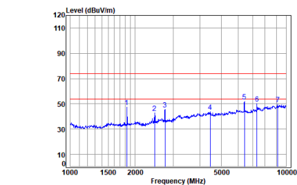
Sub_TX_CH_M_Horizontal
