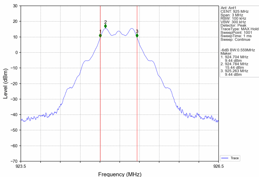
Sub_HCH_925MHz_Ant1_NTNV
