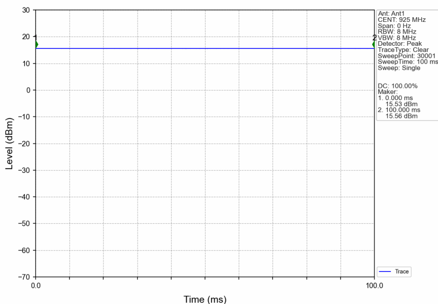
Sub_HCH_925MHz_Ant1_NTNV
