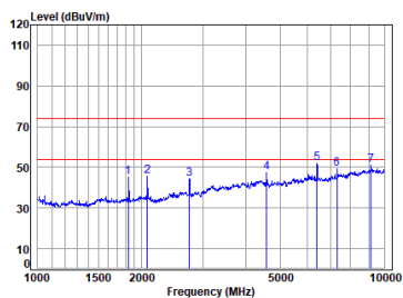
Sub_TX_CH_M_Vertical
