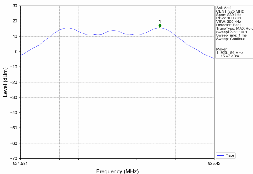
Sub_HCH_925MHz_Ant1_NTNV
