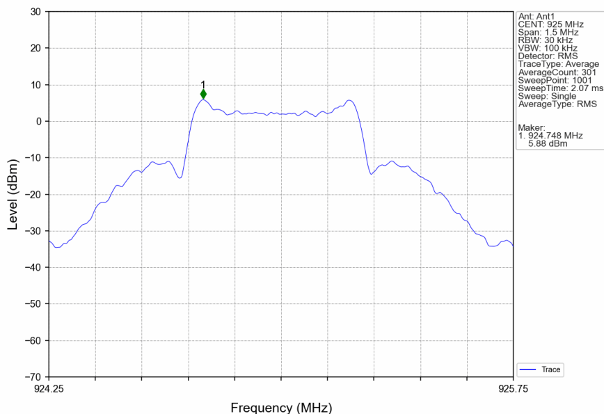
Sub_HCH_925MHz_Ant1_NTNV
