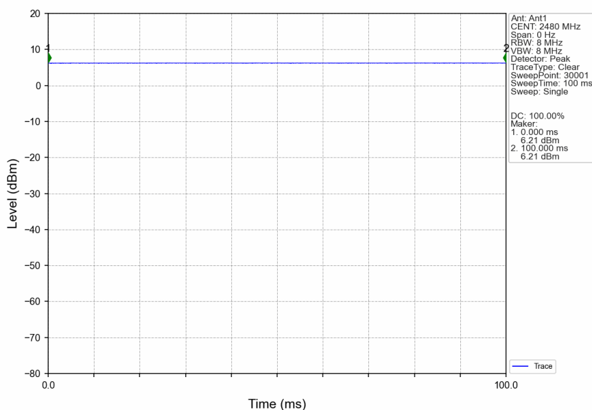
1M_HCH_2480MHz_Ant1_NTNV
