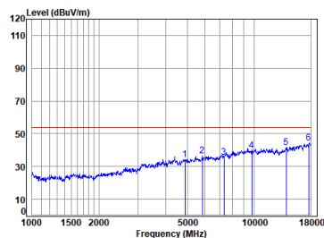
BLE_1M_TX_CH_19_Vertical-Avg
