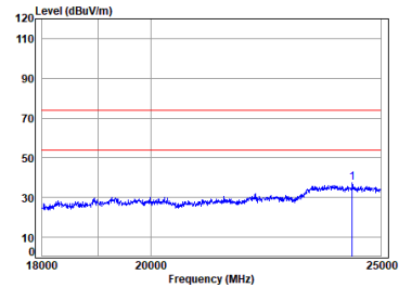
BLE_TX_CH_M_Vertical
