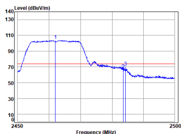
11g_TX_CH_11_Horizontal-Peak
