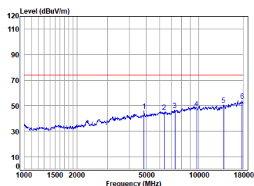
11b_TX_CH_06_Horizontal-Peak
