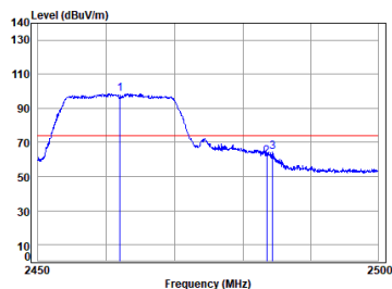
11g_TX_CH_11_Vertical-Peak
