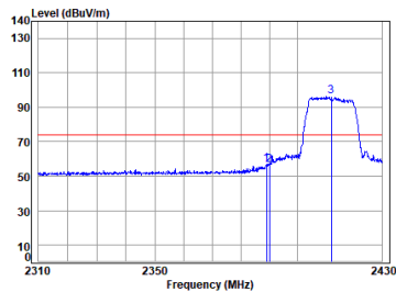
11g_TX_CH_01_Vertical-Peak
