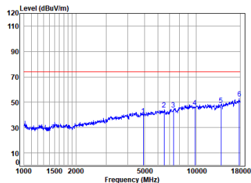
11g_TX_CH_11_Vertical-Peak
