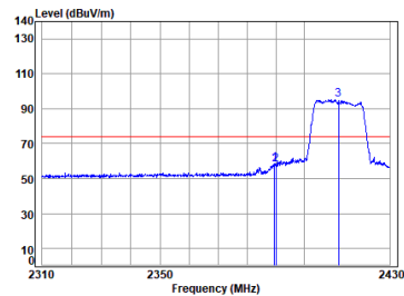
11n_HT(20M)_TX_CH_01_Vertical-Peak
