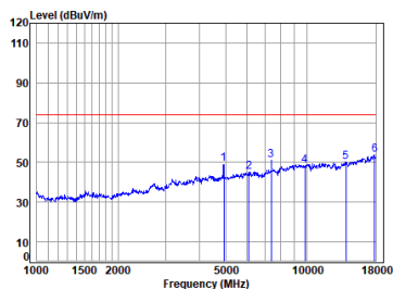
11b_TX_CH_11_Vertical-Peak
