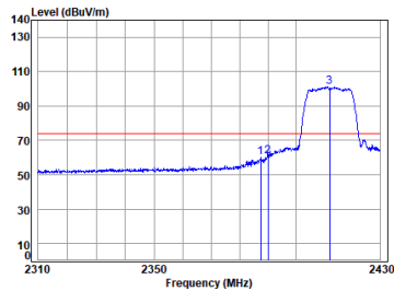
11g_TX_CH_01_Horizontal-Peak
