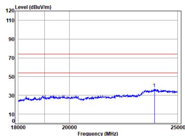
2.4G WIFI_TX_CH_M_Vertical
