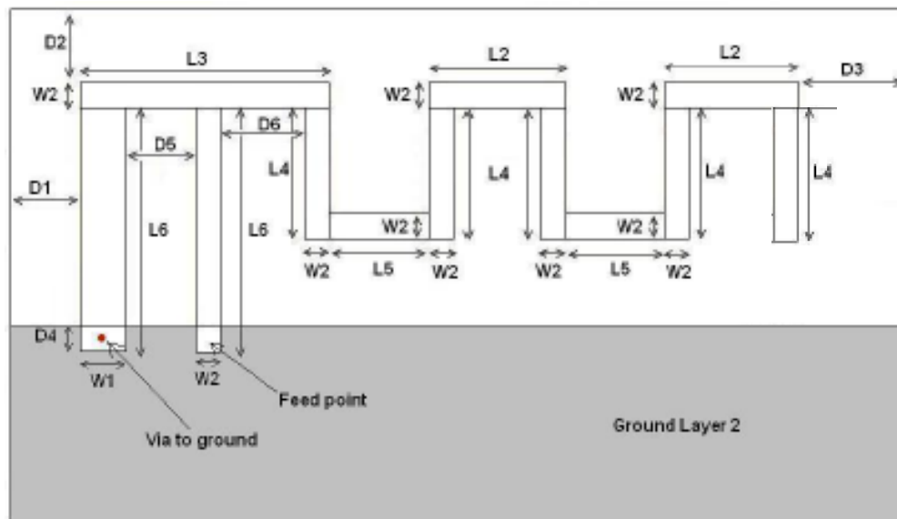
Figure 3: Antenna Dimensions
