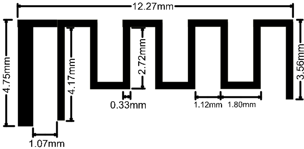
Figure 3: Antenna Dimensions
