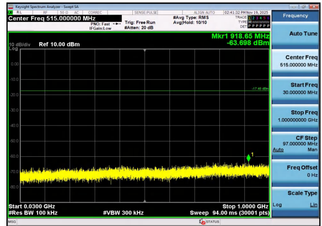
30MHz-1G
