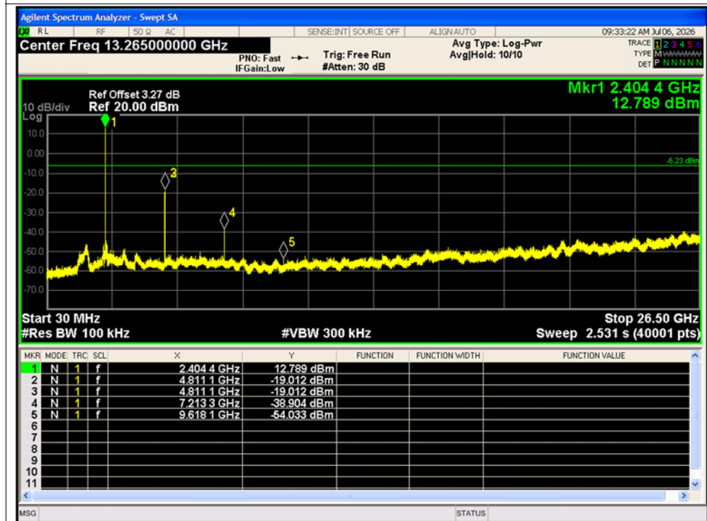
Tx. Spurious NVNT Zigbee 2405MHz Ant1 Emission
