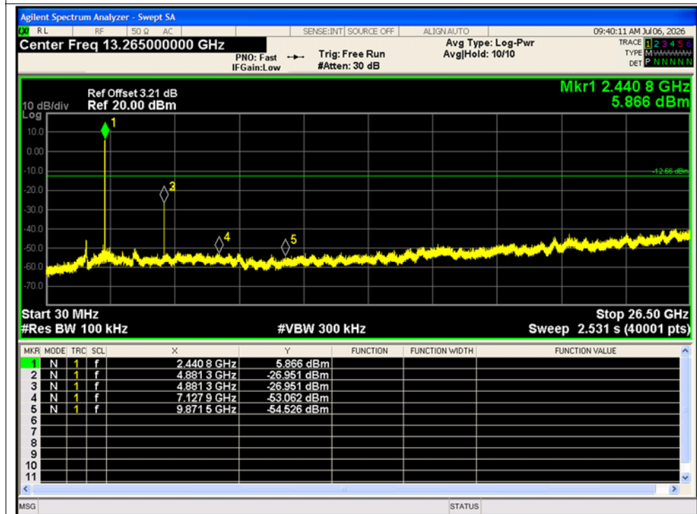
Tx. Spurious NVNT Zigbee 2440MHz Ant1 Emission
