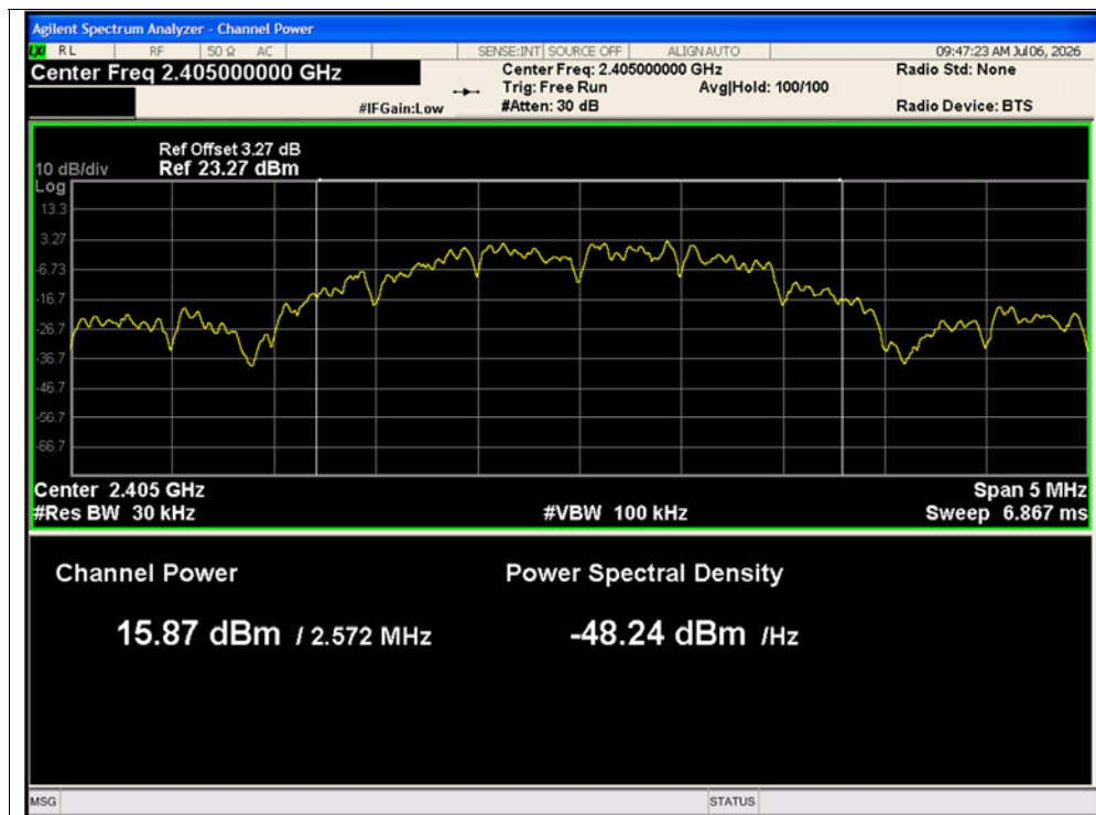
Average Power NVNT Zigbee 2405MHz Ant1
