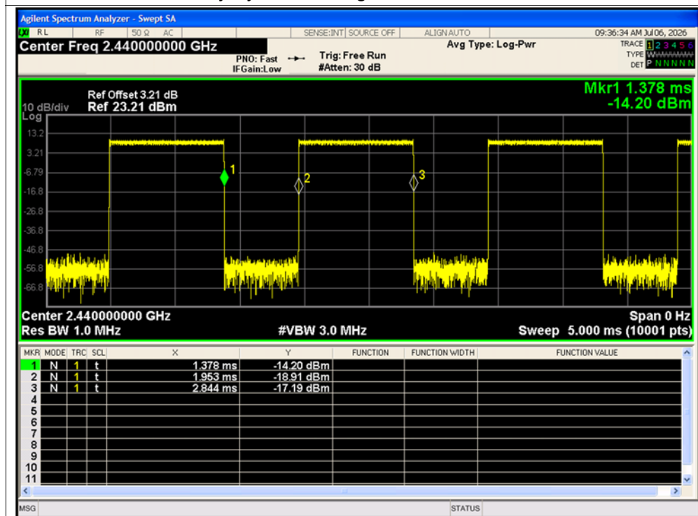
Duty Cycle NVNT Zigbee 2440MHz Ant1
