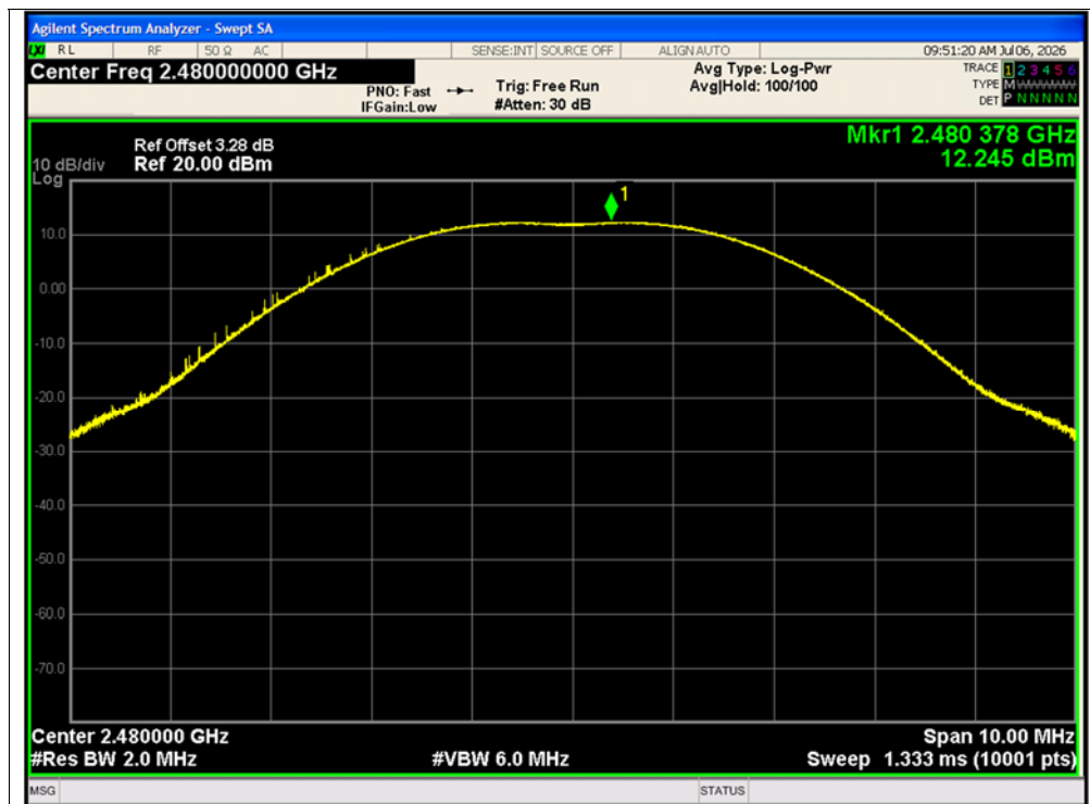
Peak Power NVNT Zigbee 2480MHz Ant1
