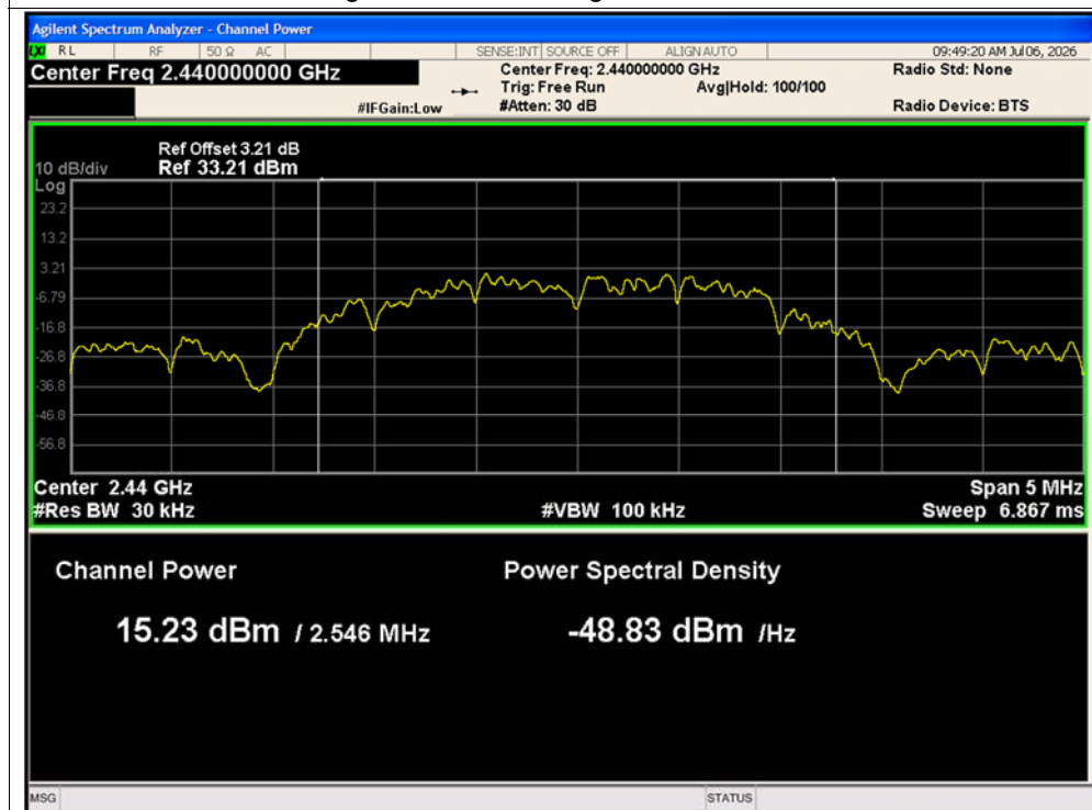
Average Power NVNT Zigbee 2440MHz Ant1
