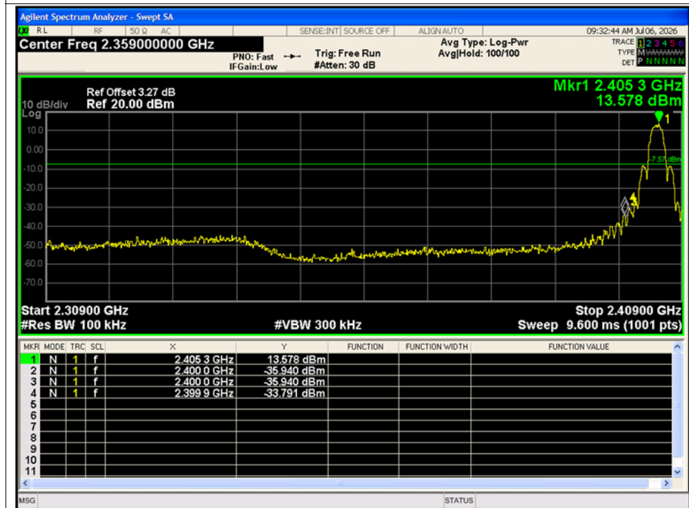
Band Edge NVNT Zigbee 2405MHz Ant1 Emission
