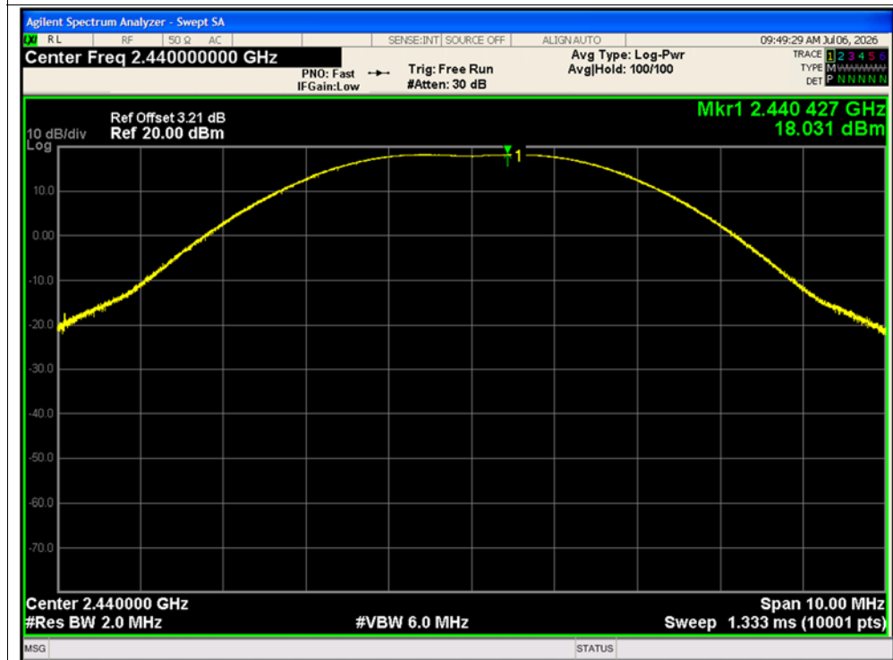
Peak Power NVNT Zigbee 2440MHz Ant1
