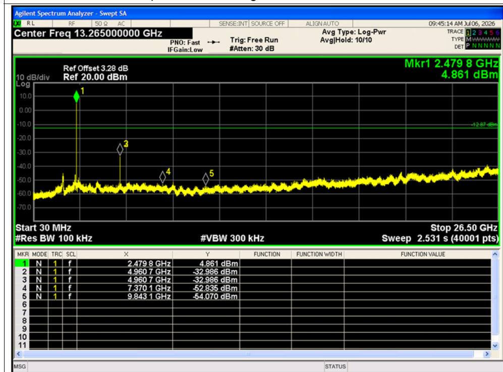
Tx. Spurious NVNT Zigbee 2480MHz Ant1 Emission
