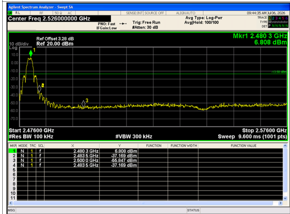
Band Edge NVNT Zigbee 2480MHz Ant1 Emission
