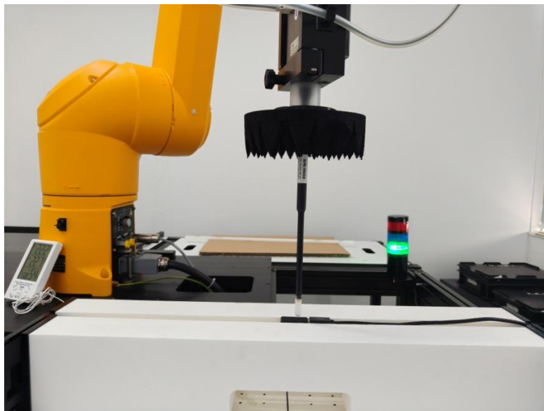
Horizontal Down (Test distance: 2mm)
