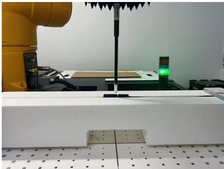
Vertical Back (Test distance: 2mm)
