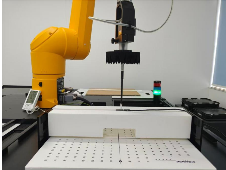
Horizontal Up (Test distance: 2mm)
