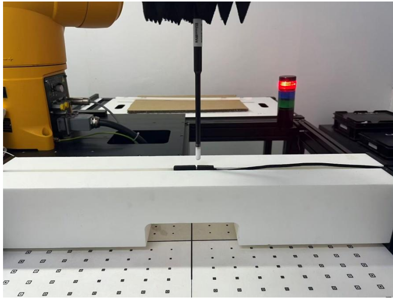
Vertical Front (Test distance: 2mm)
