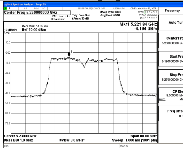
11AC40MIMO Ant3 5230
