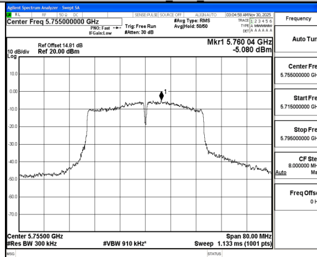
11N40MIMO Ant3 5755
