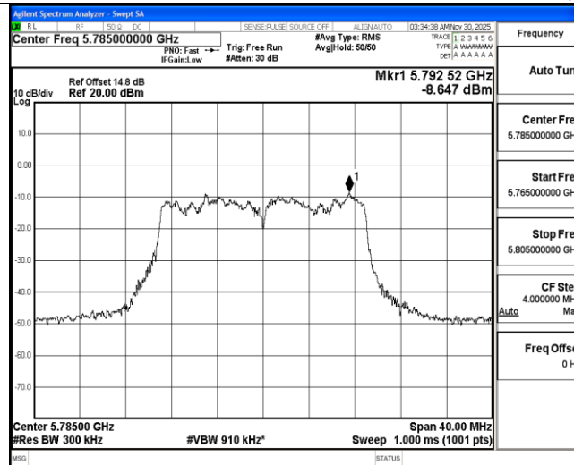
11AC20MIMO Ant2 5785
