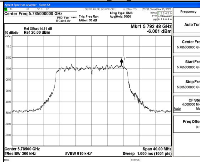
11AC20MIMO Ant3 5785
