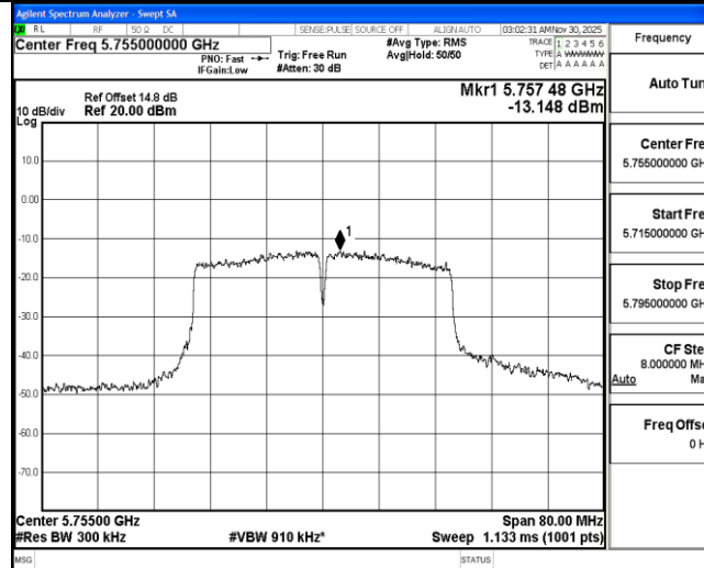
11N40MIMO Ant2 5755
