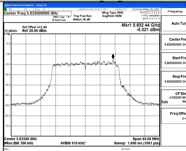
11AC20MIMO Ant3 5825
