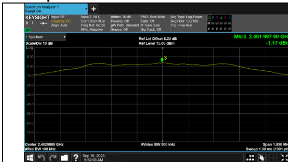
In-Band Reference Level BLE 1M_Channel 0
