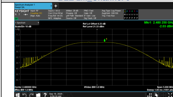
Peak Output Power BLE 1M_Channel 39
