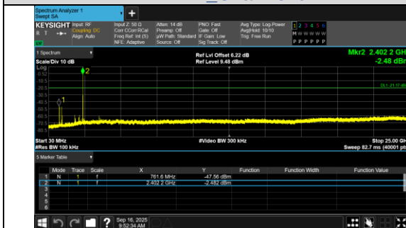
30.0 MHz - 25000.0 MHz BLE 1M_Channel 0
