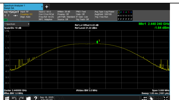
Peak Output Power BLE 1M_Channel 19
