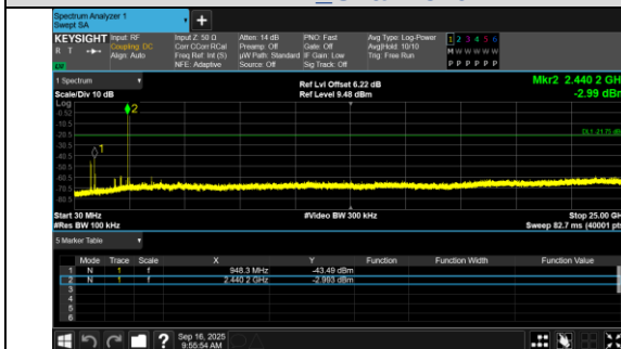
30.0 MHz - 25000.0 MHz BLE 1M_Channel 19
