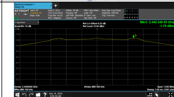
In-Band Reference Level BLE 1M_Channel 19
