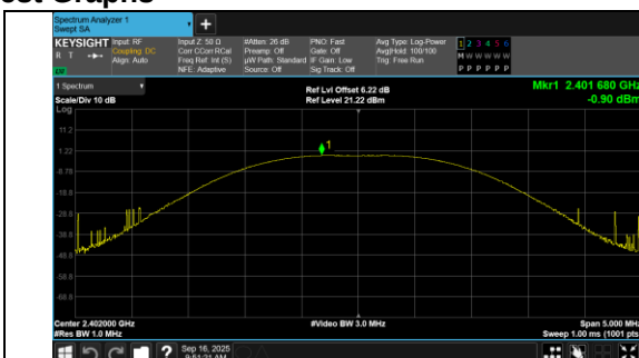
Peak Output Power BLE 1M_Channel 0
