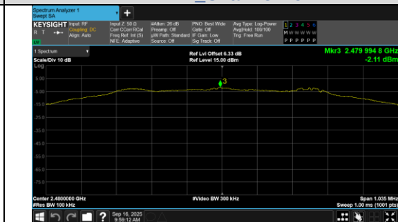
In-Band Reference Level BLE 1M_Channel 39
