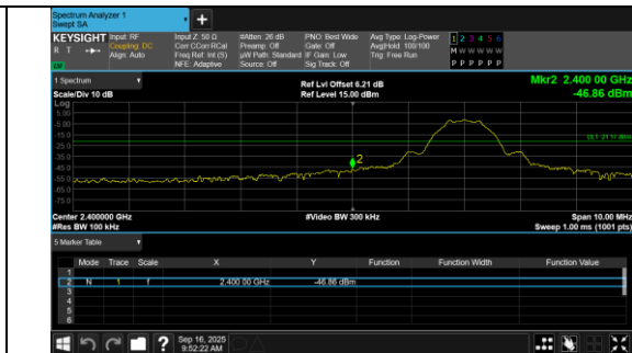
Out Of Band Emission BLE 1M_Channel 0
