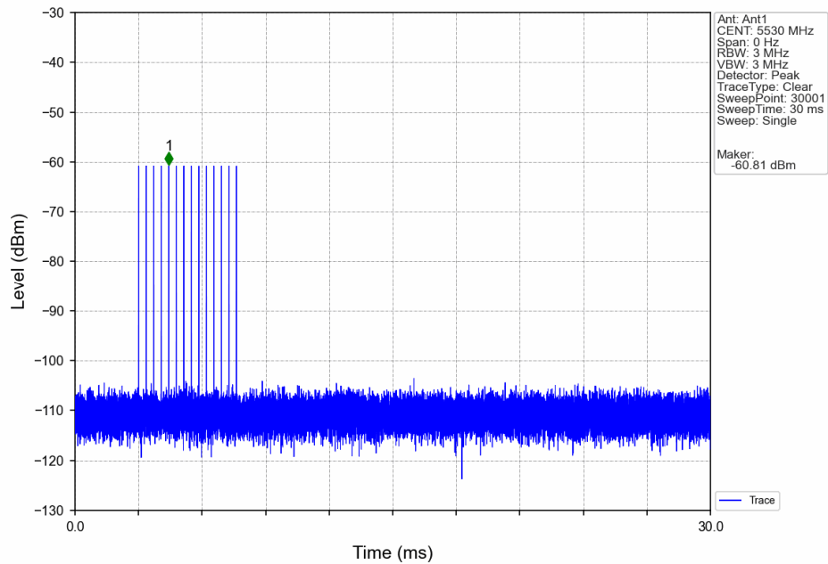
Signal Calibration_802.11ax(HEW80)_2C_5530MHz_RadarType5_Trial0
