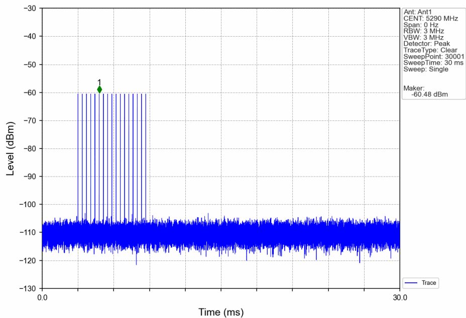
Signal Calibration_802.11ax(HEW80)_2A_5290MHz_RadarType3_Trial0
