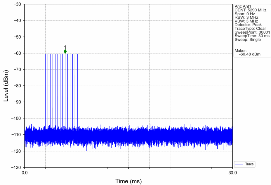
Signal Calibration_802.11ax(HEW80)_2A_5290MHz_RadarType5_Trial0
