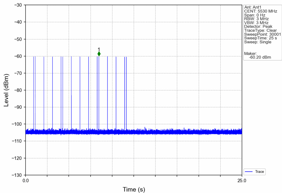
Signal Calibration_802.11ax(HEW80)_2C_5530MHz_RadarType5_Trial0
