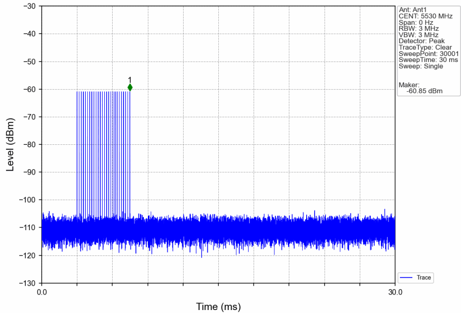
Signal Calibration_802.11ax(HEW80)_2C_5530MHz_RadarType3_Trial0
