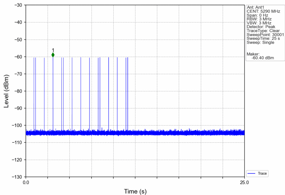
Signal Calibration_802.11ax(HEW80)_2A_5290MHz_RadarType5_Trial0
