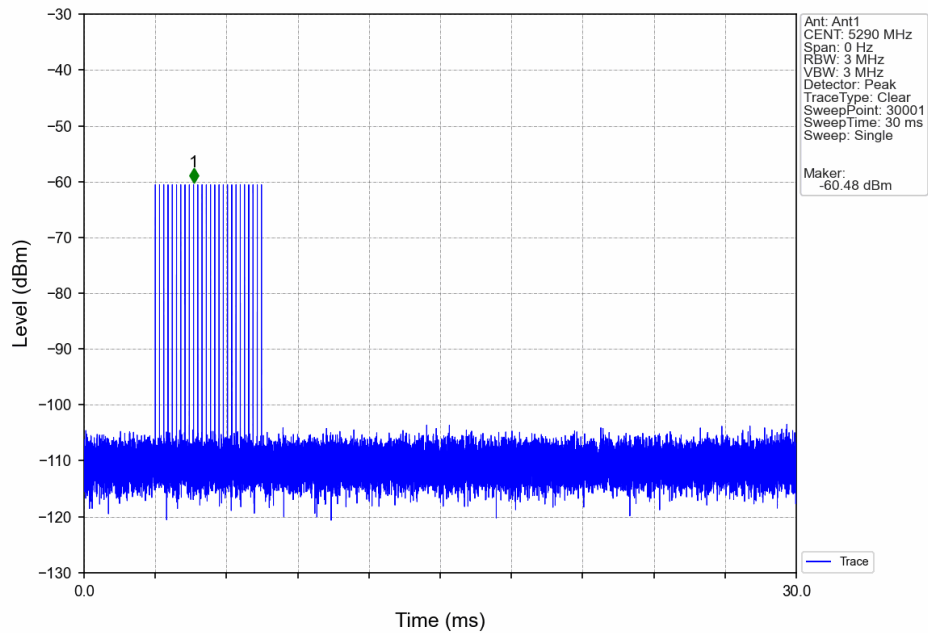
Signal Calibration_802.11ax(HEW80)_2A_5290MHz_RadarType3_Trial0
