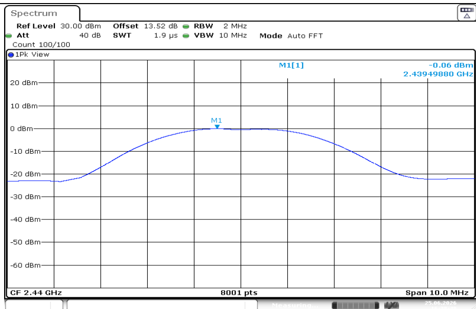
BLE_2M-Ant1-2440-PASS
