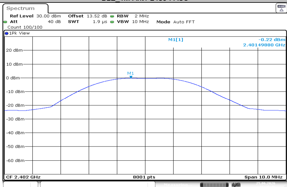
BLE_2M-Ant1-2402-PASS
