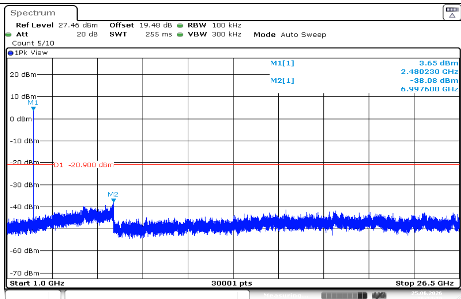
BLE_1M-Ant1-2480-1000~26500-PASS
