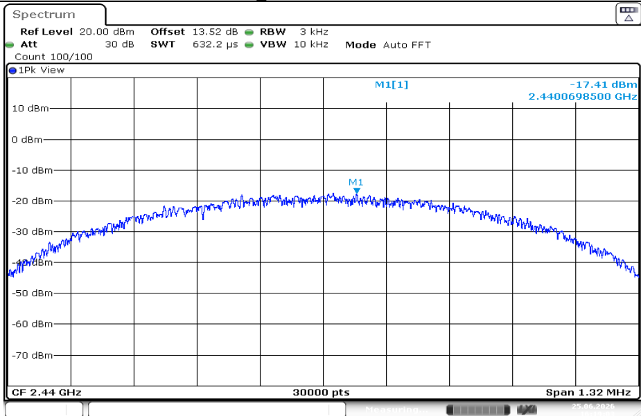
BLE_1M-Ant1-2440-PASS
