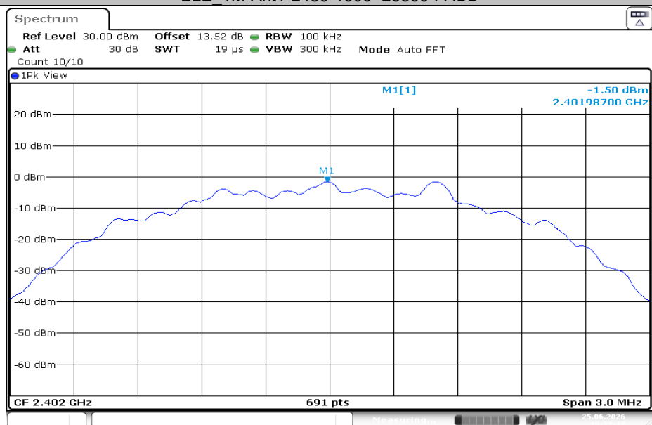
BLE_2M-Ant1-2402-0~Reference-PASS
