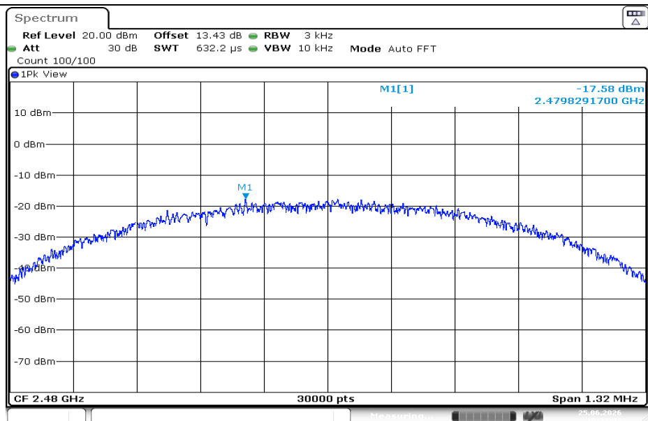
BLE_1M-Ant1-2480-PASS
