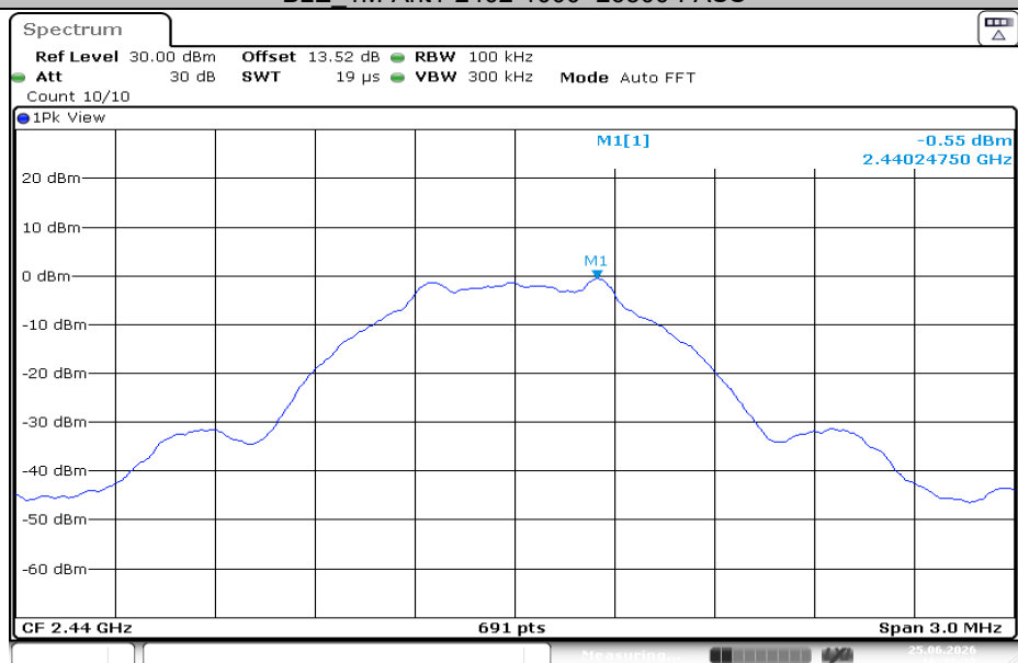
BLE_1M-Ant1-2440-0~Reference-PASS
