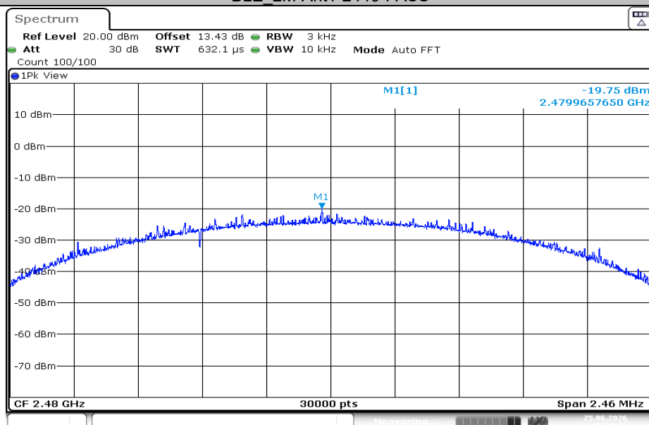
BLE_2M-Ant1-2480-PASS
