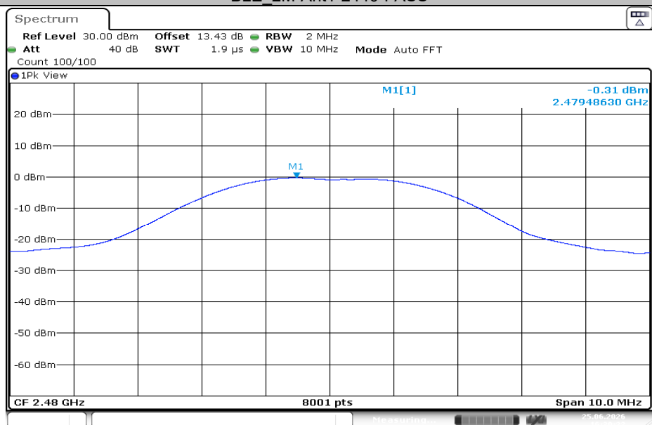
BLE_2M-Ant1-2480-PASS
