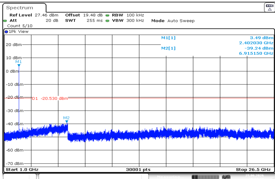
BLE_1M-Ant1-2402-1000~26500-PASS
