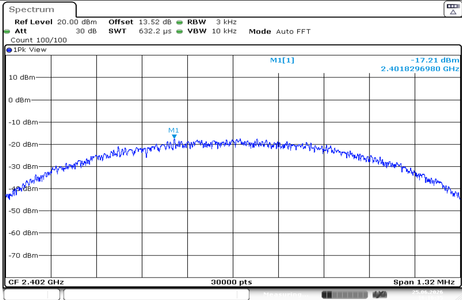
BLE_1M-Ant1-2402-PASS
