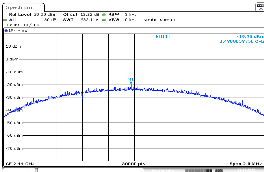
BLE_2M-Ant1-2440-PASS
