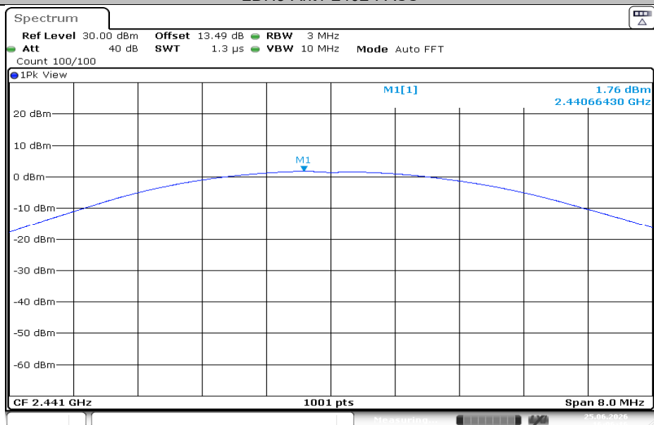
2DH5-Ant1-2441-PASS
