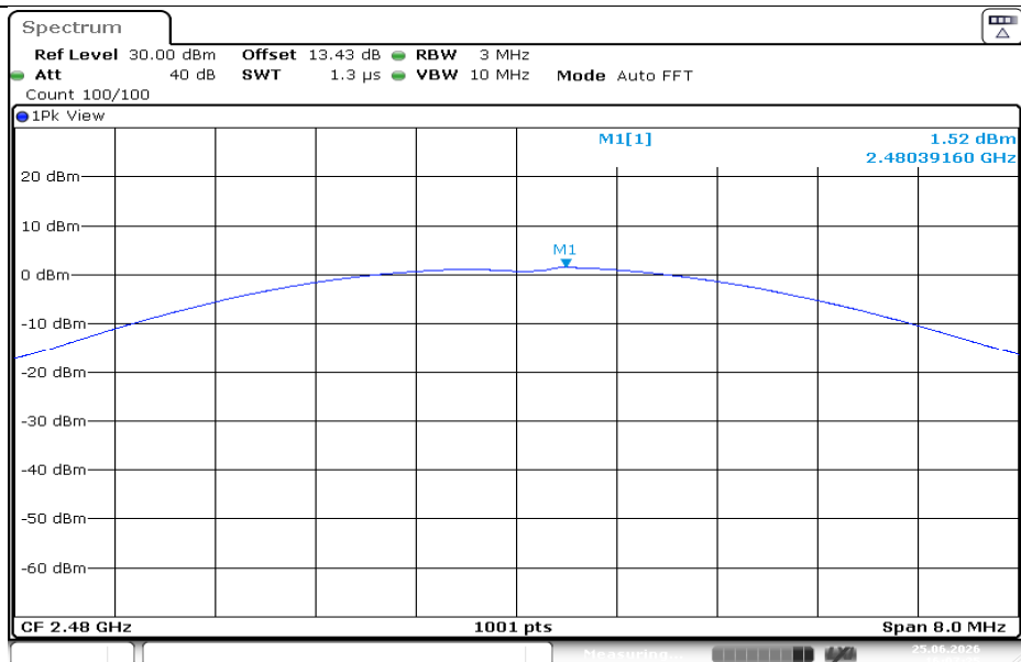
2DH5-Ant1-2480-PASS
