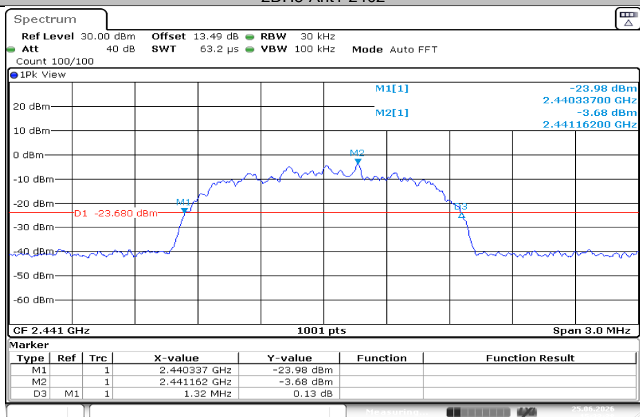
2DH5-Ant1-2441
