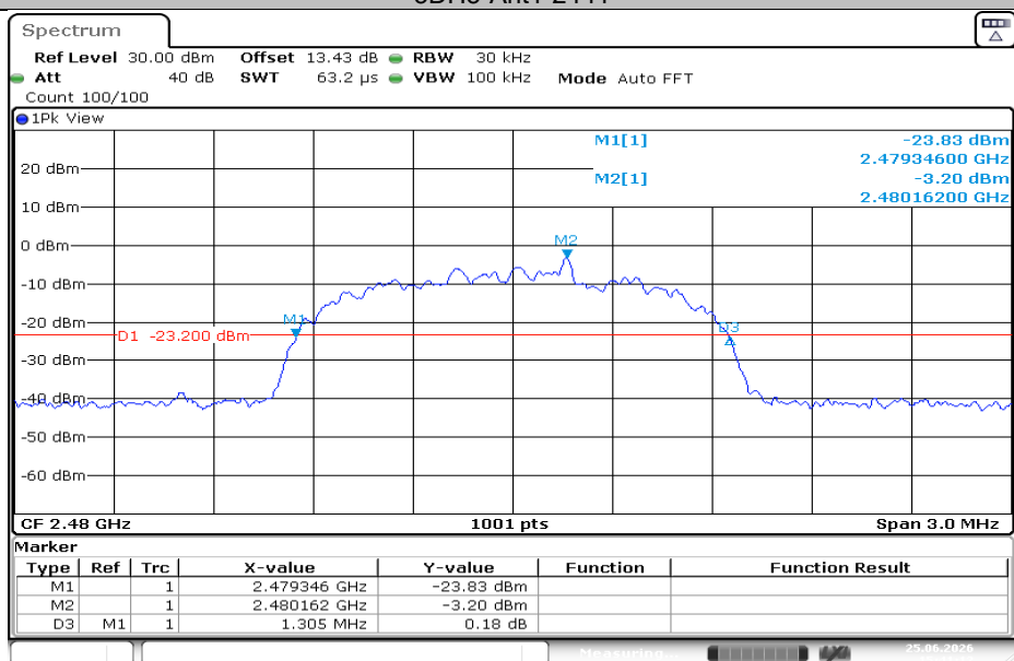
3DH5-Ant1-2480
