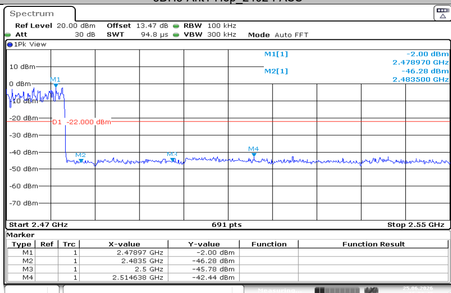
3DH5-Ant1-Hop_2480-PASS
