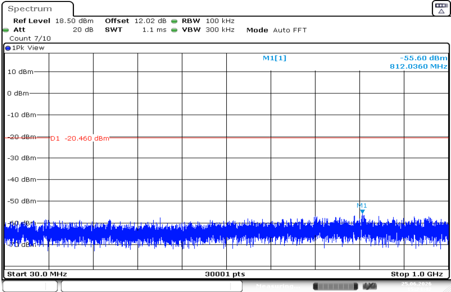
DH5-Ant1-2402-30~1000-PASS
