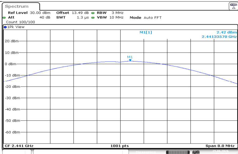
3DH5-Ant1-2441-PASS
