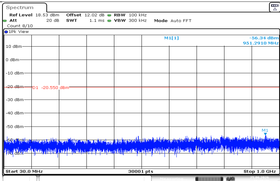
3DH5-Ant1-2441-30~1000-PASS
