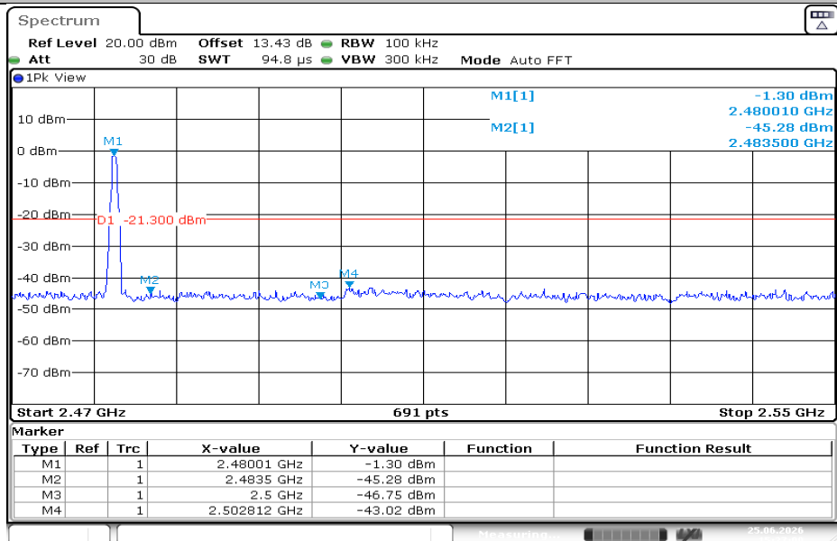
DH5-Ant1-2480-PASS
