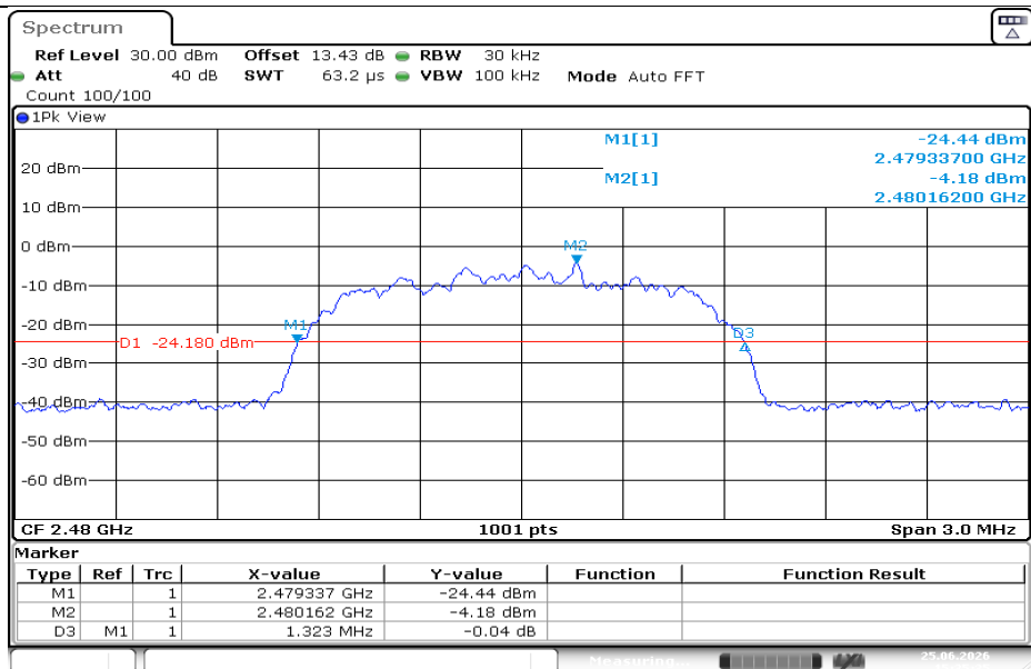
2DH5-Ant1-2480
