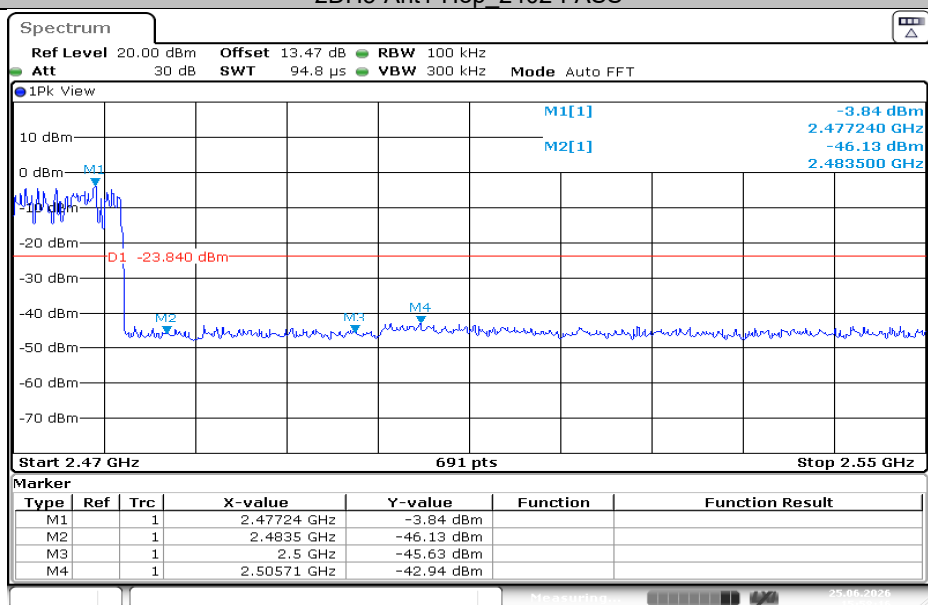
2DH5-Ant1-Hop_2480-PASS
