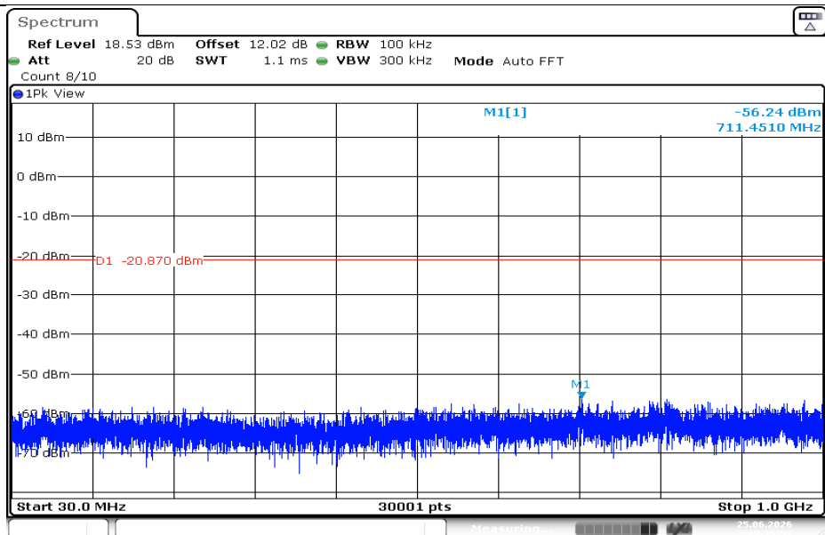
DH5-Ant1-2441-30~1000-PASS
