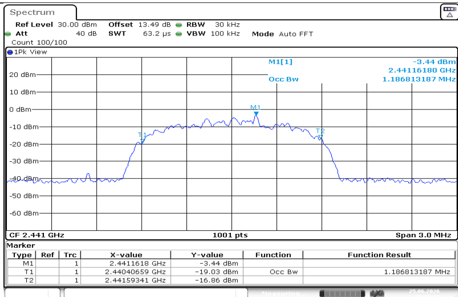
3DH5-Ant1-2441
