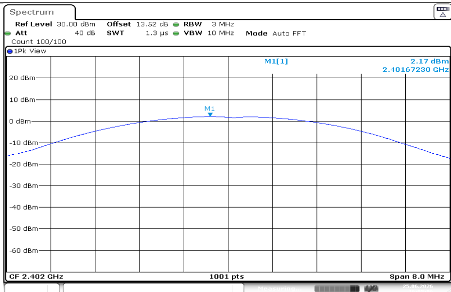
2DH5-Ant1-2402-PASS
