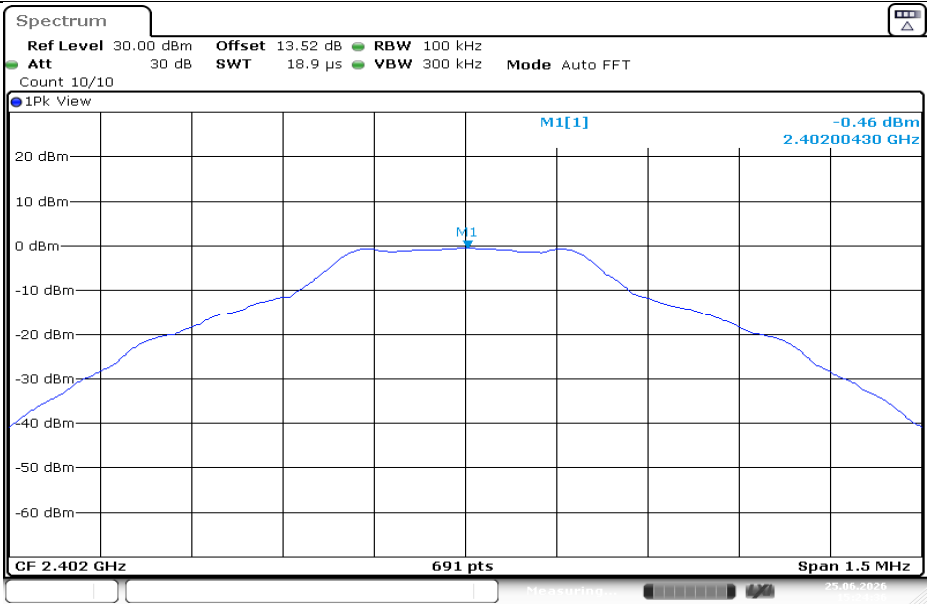
DH5-Ant1-2402-0~Reference-PASS
