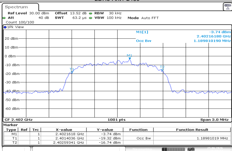
3DH5-Ant1-2402
