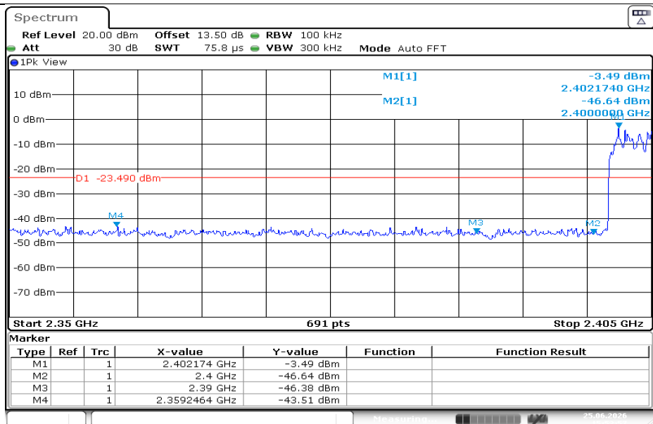
2DH5-Ant1-Hop_2402-PASS
