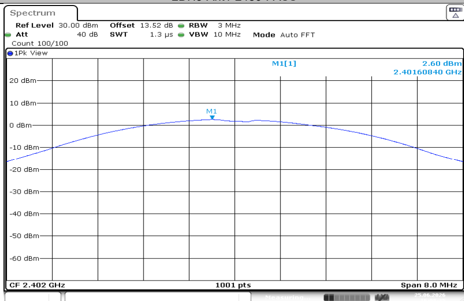
3DH5-Ant1-2402-PASS
