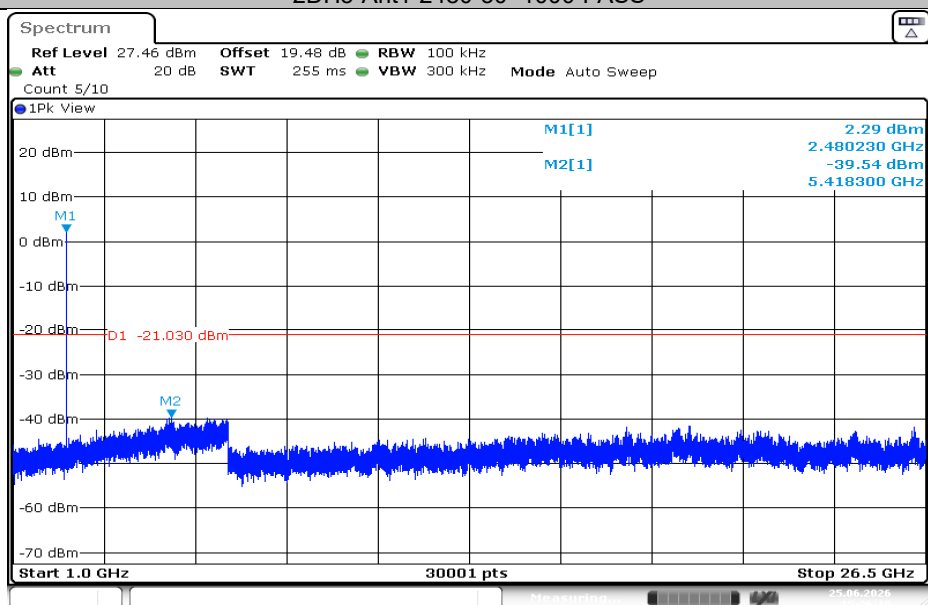
2DH5-Ant1-2480-1000~26500-PASS
