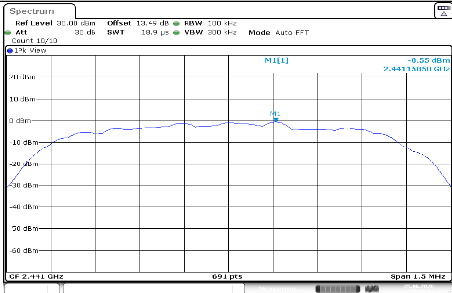
3DH5-Ant1-2441-0~Reference-PASS
