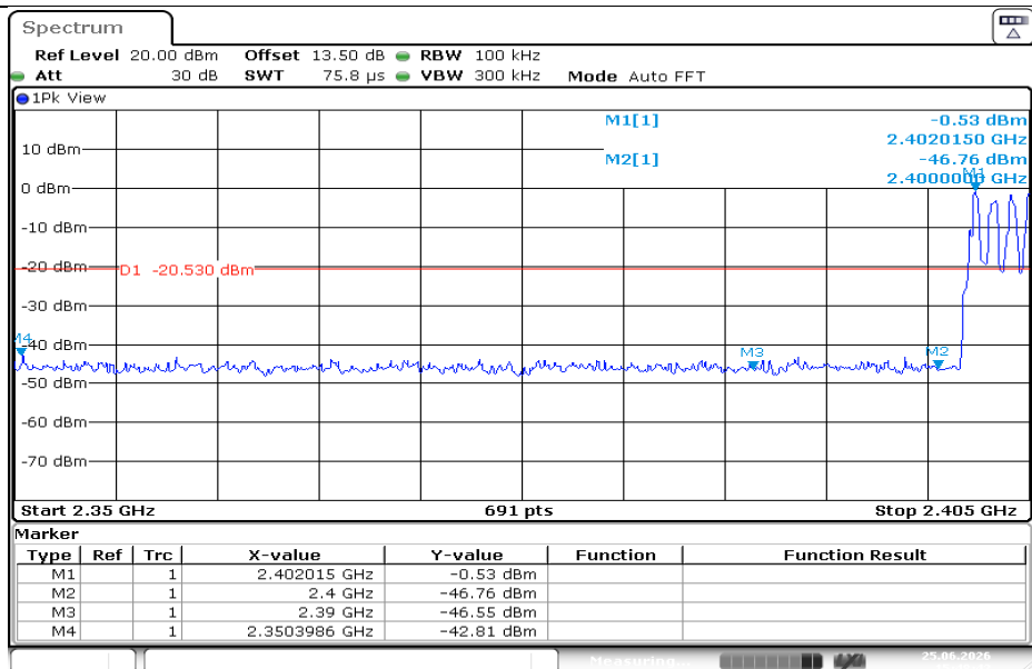
DH5-Ant1-Hop_2402-PASS
