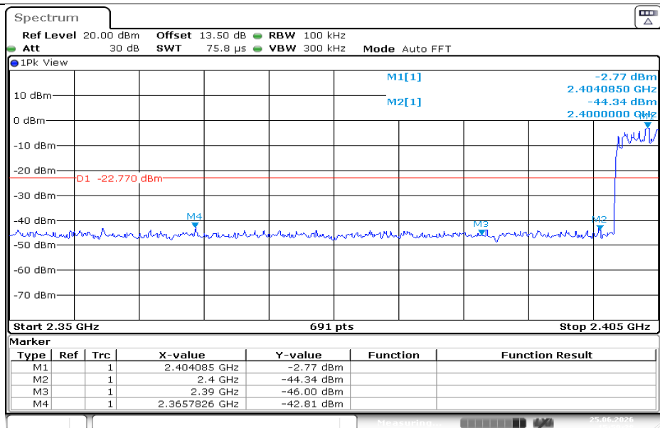
3DH5-Ant1-Hop_2402-PASS
