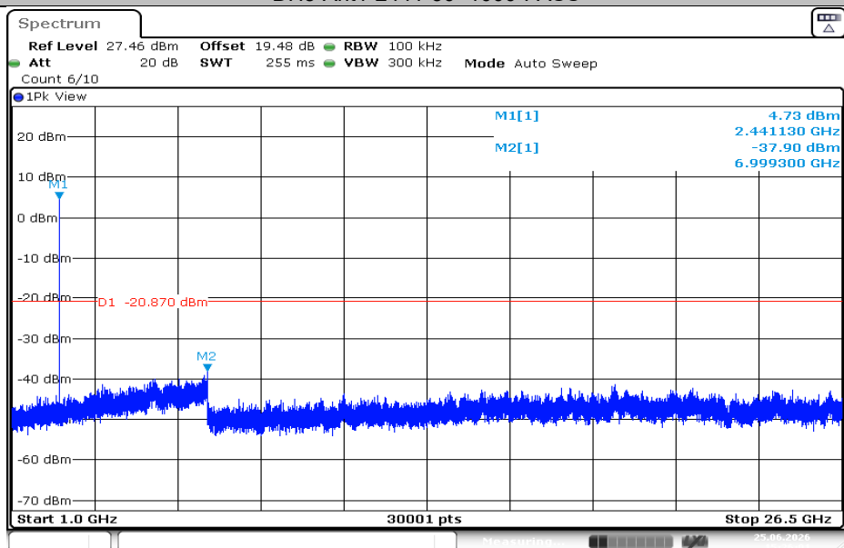
DH5-Ant1-2441-1000~26500-PASS
