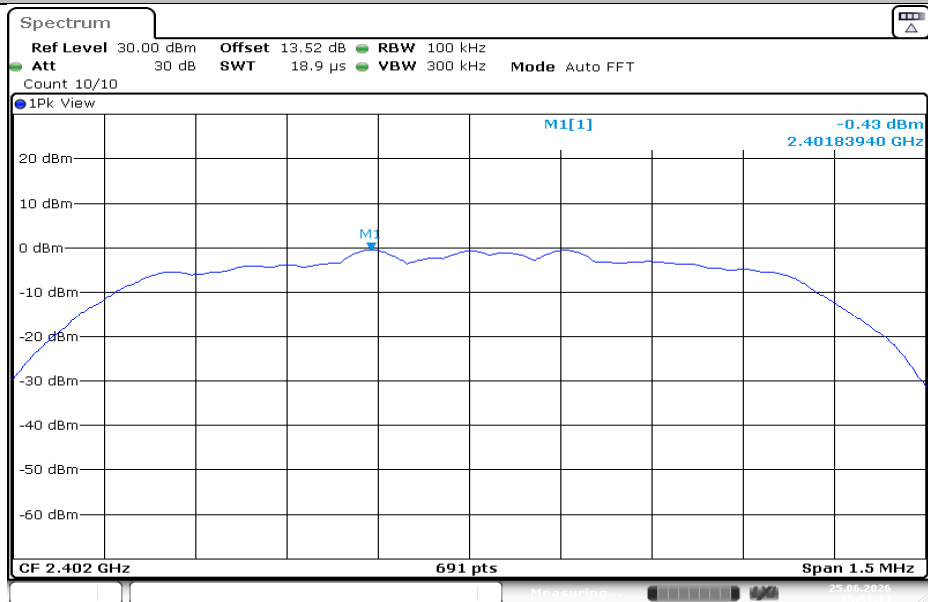
2DH5-Ant1-2402-0~Reference-PASS
