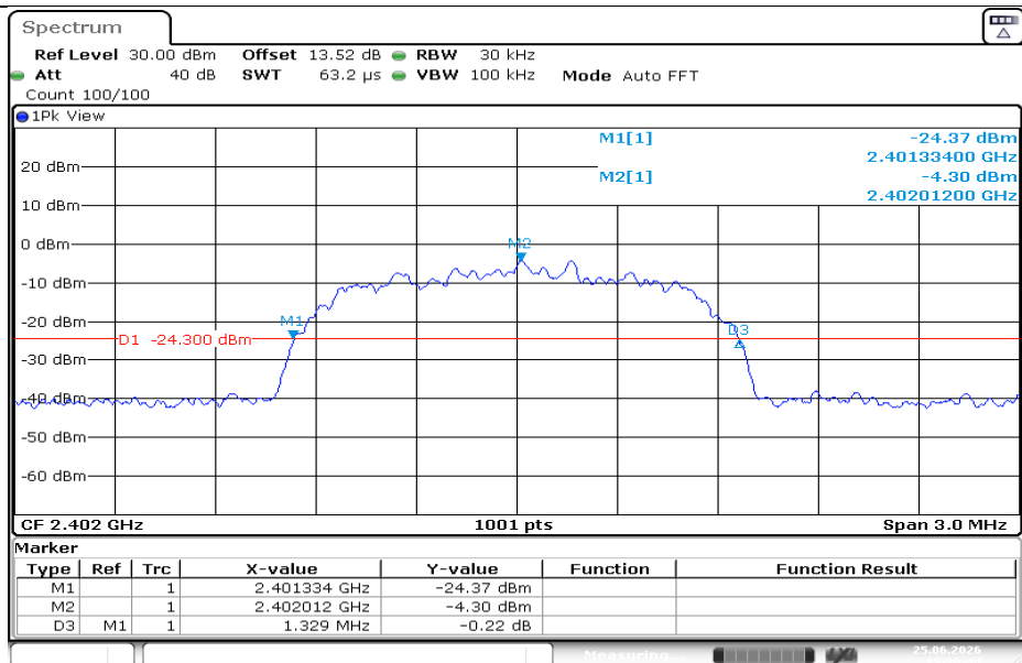
2DH5-Ant1-2402
