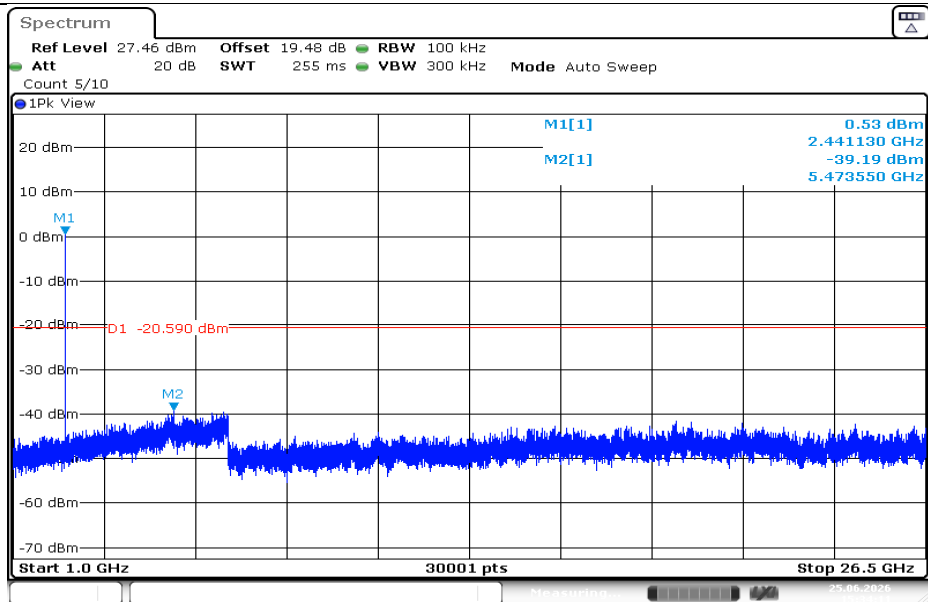
2DH5-Ant1-2441-1000~26500-PASS
