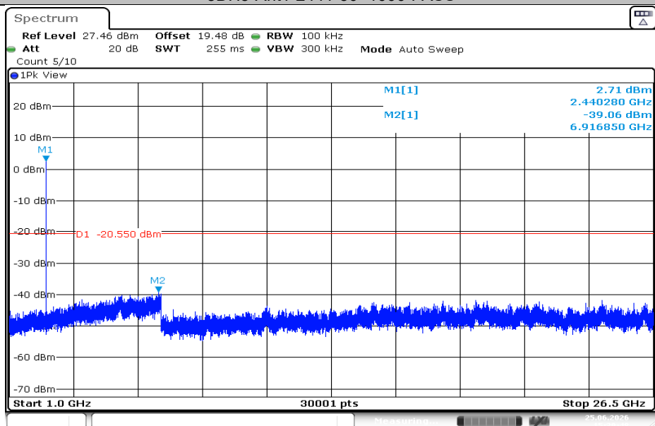
3DH5-Ant1-2441-1000~26500-PASS
