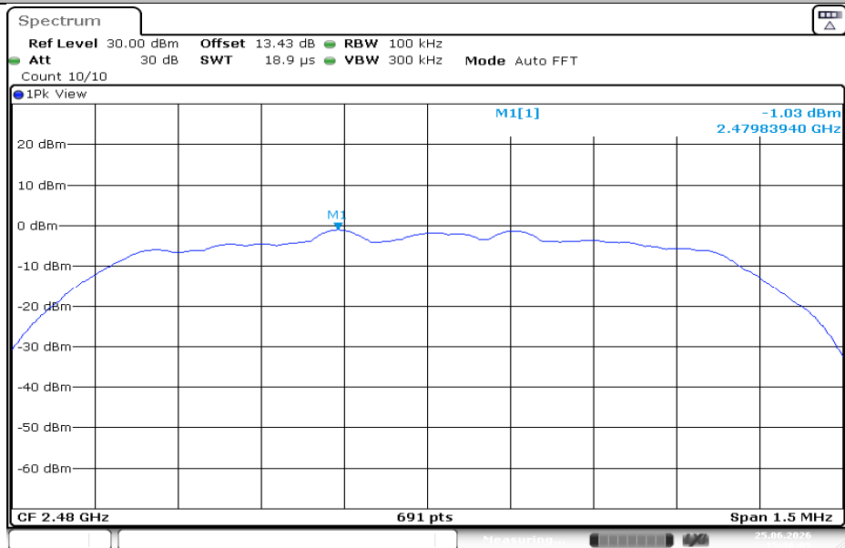
2DH5-Ant1-2480-0~Reference-PASS
