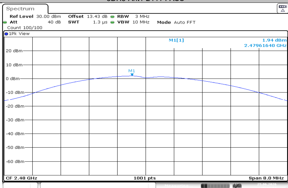
3DH5-Ant1-2480-PASS
