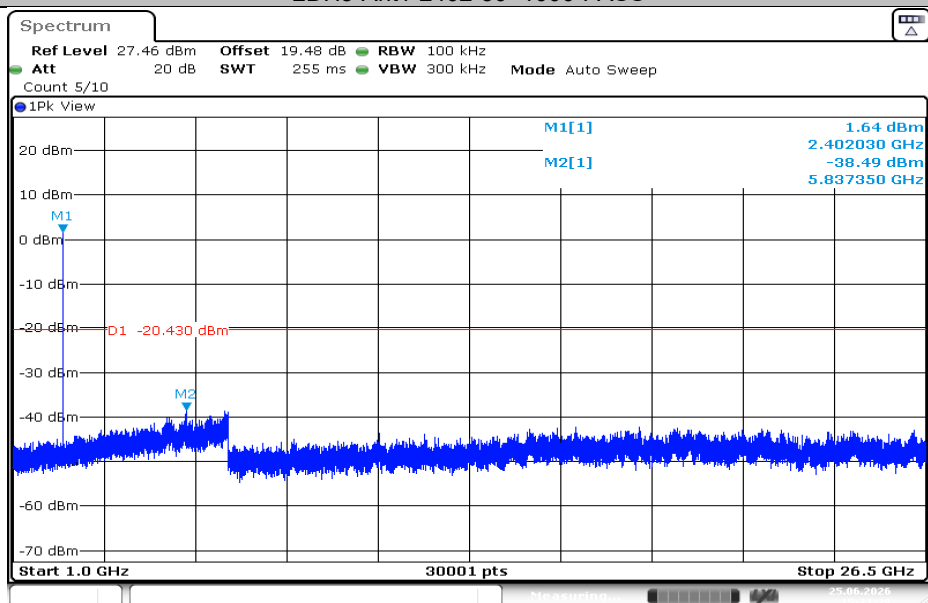
2DH5-Ant1-2402-1000~26500-PASS
