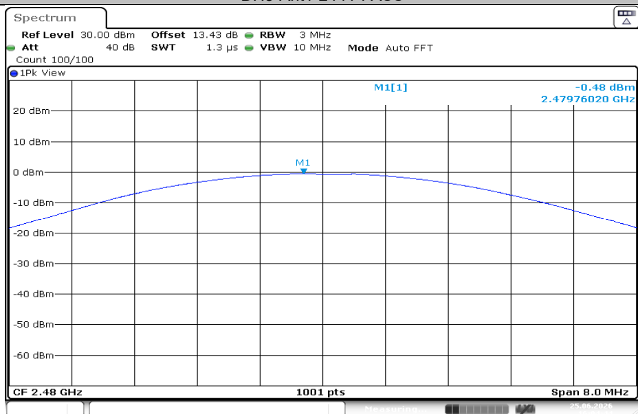
DH5-Ant1-2480-PASS
