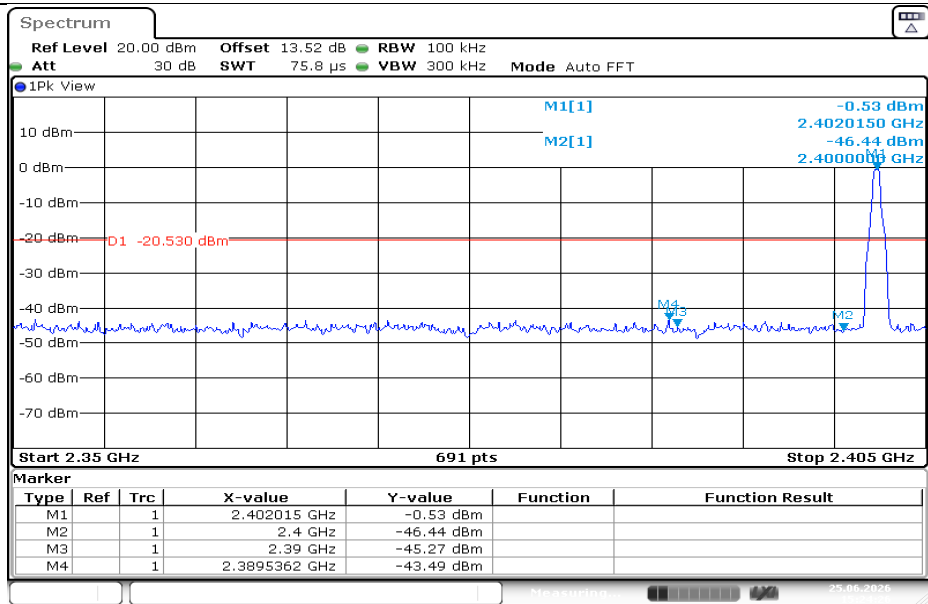
DH5-Ant1-2402-PASS
