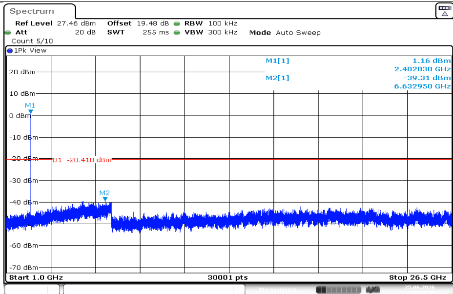
3DH5-Ant1-2402-1000~26500-PASS
