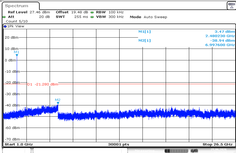
DH5-Ant1-2480-1000~26500-PASS
