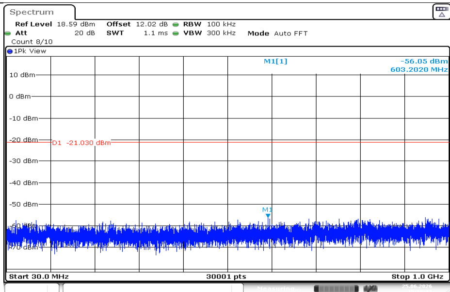
2DH5-Ant1-2480-30~1000-PASS
