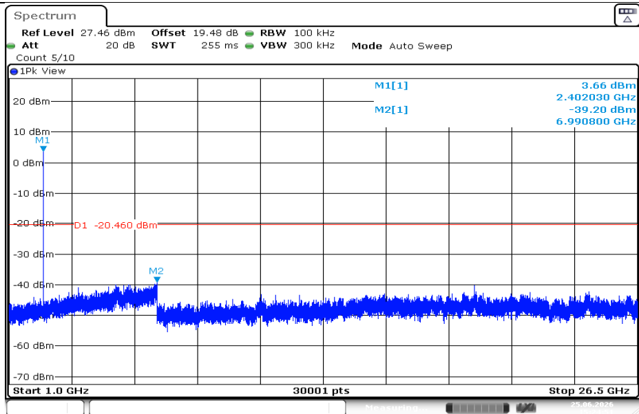
DH5-Ant1-2402-1000~26500-PASS
