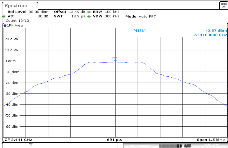
DH5-Ant1-2441-0~Reference-PASS
