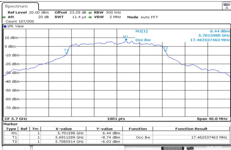
11A-CDD-Ant1-5700
