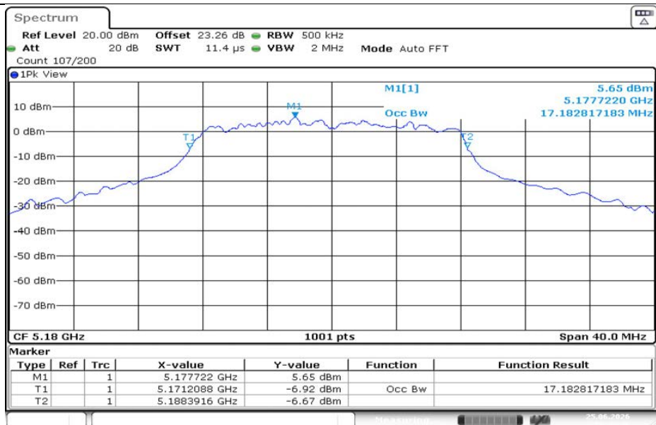
11A-CDD-Ant1-5180
