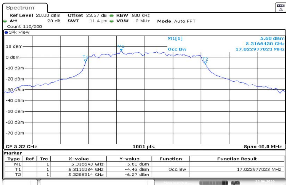
11A-CDD-Ant1-5320
