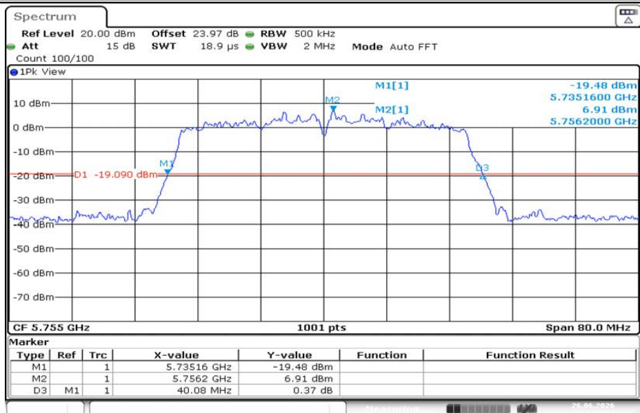
11AC40MIMO-Ant2-5755
