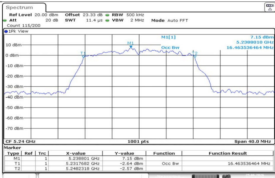
11A-CDD-Ant1-5240
