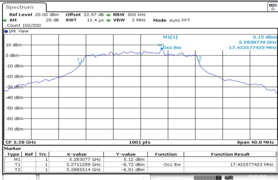
11A-CDD-Ant2-5280
