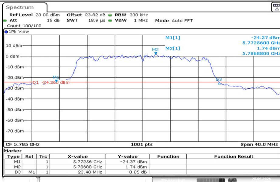
11AX20MIMO-Ant2-5785
