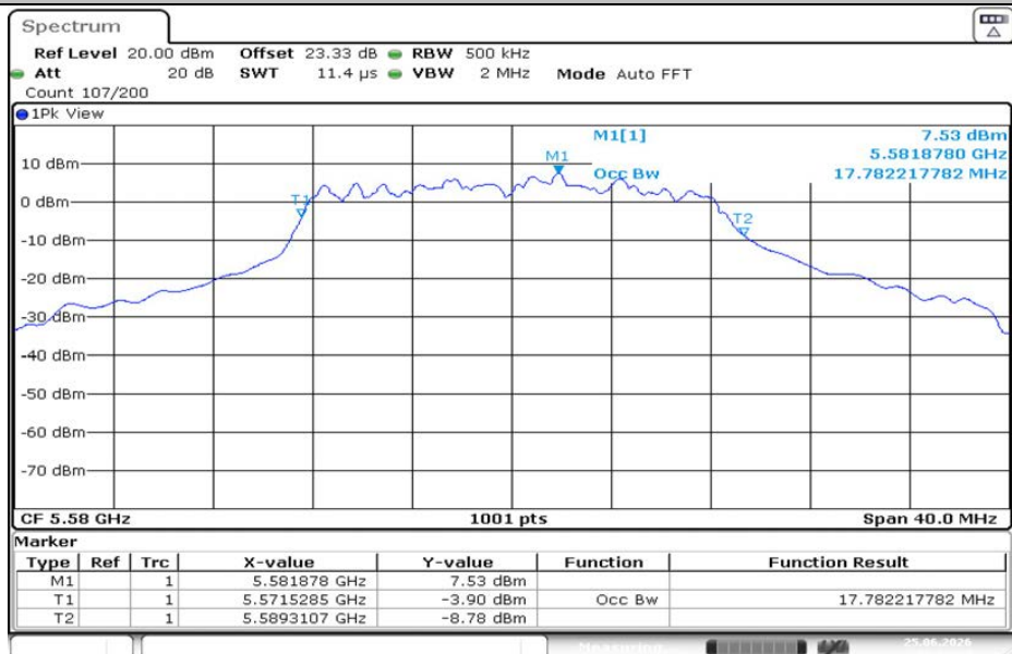
11A-CDD-Ant2-5580
