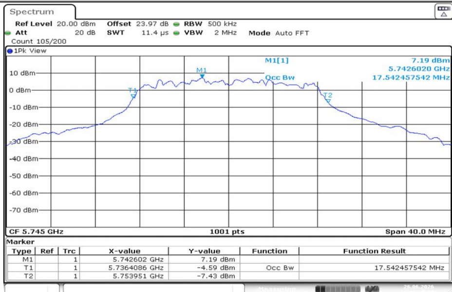
11A-CDD-Ant2-5745
