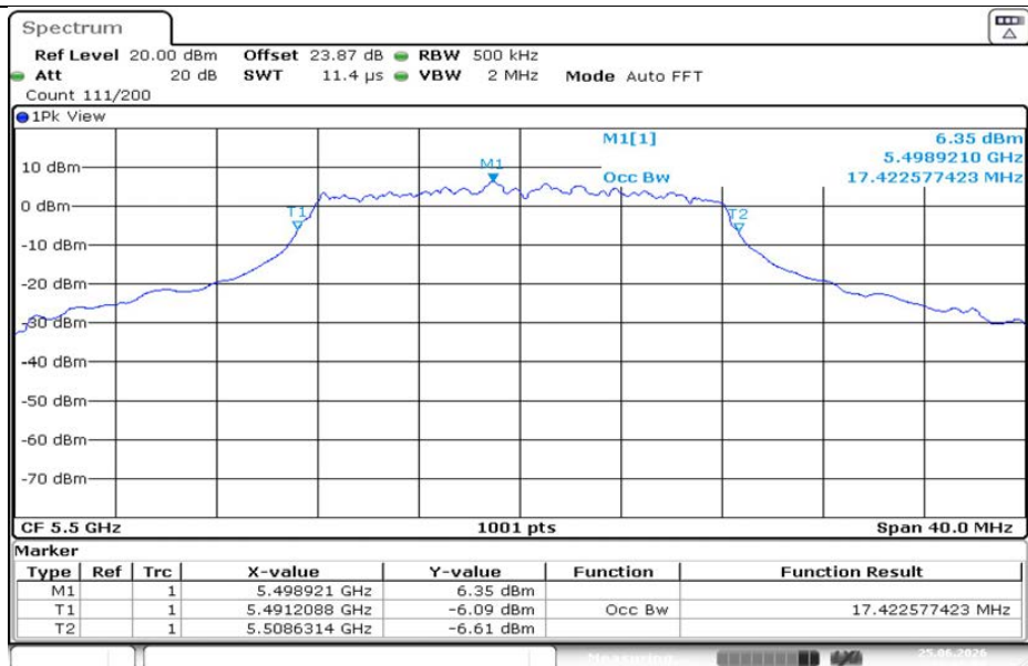
11A-CDD-Ant1-5500
