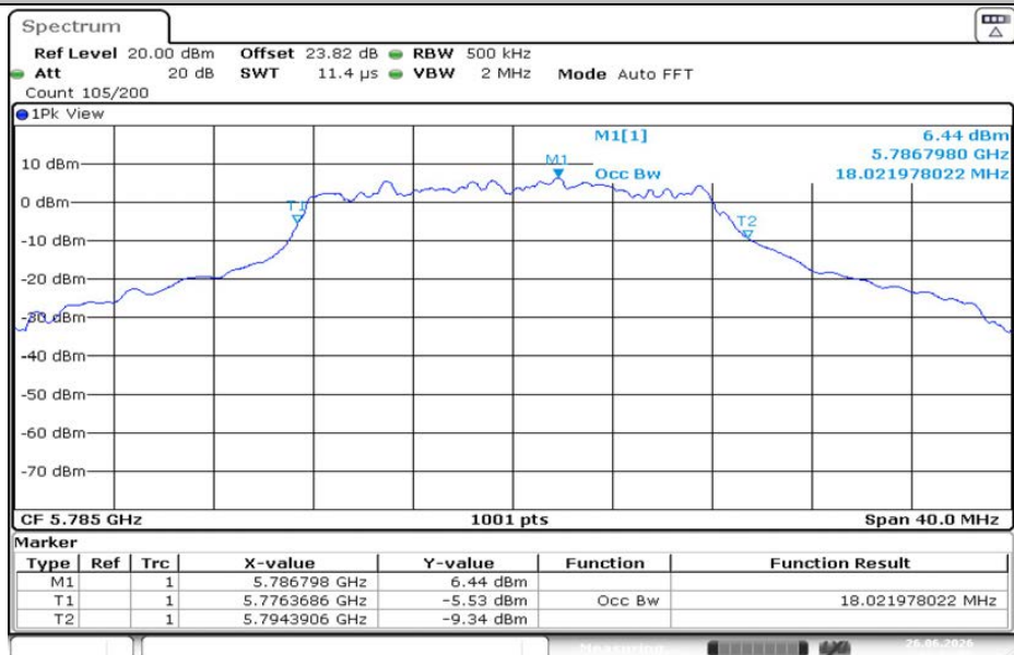
11A-CDD-Ant2-5785
