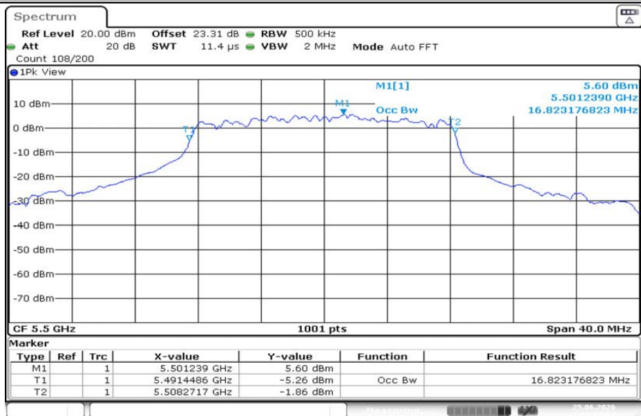
11A-CDD-Ant2-5500
