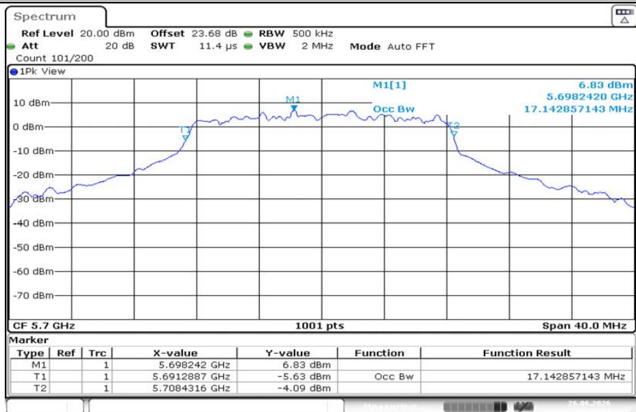
11A-CDD-Ant2-5700
