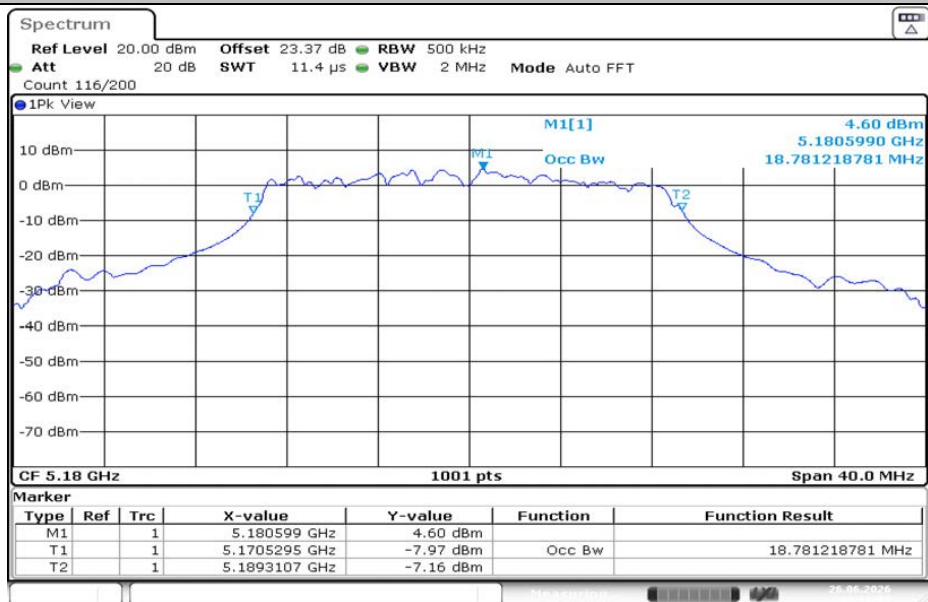
11N20MIMO-Ant2-5180
