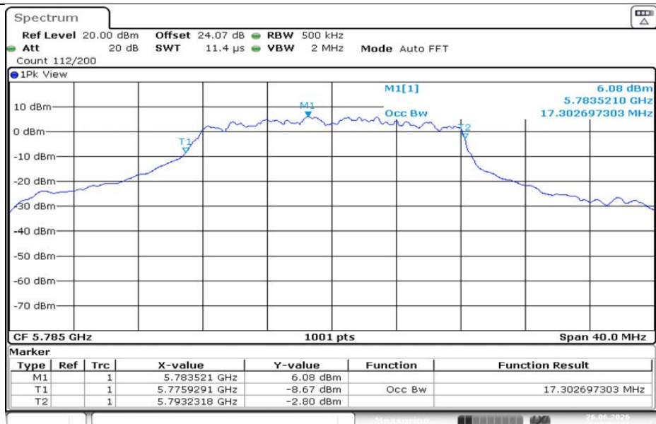
11A-CDD-Ant1-5785
