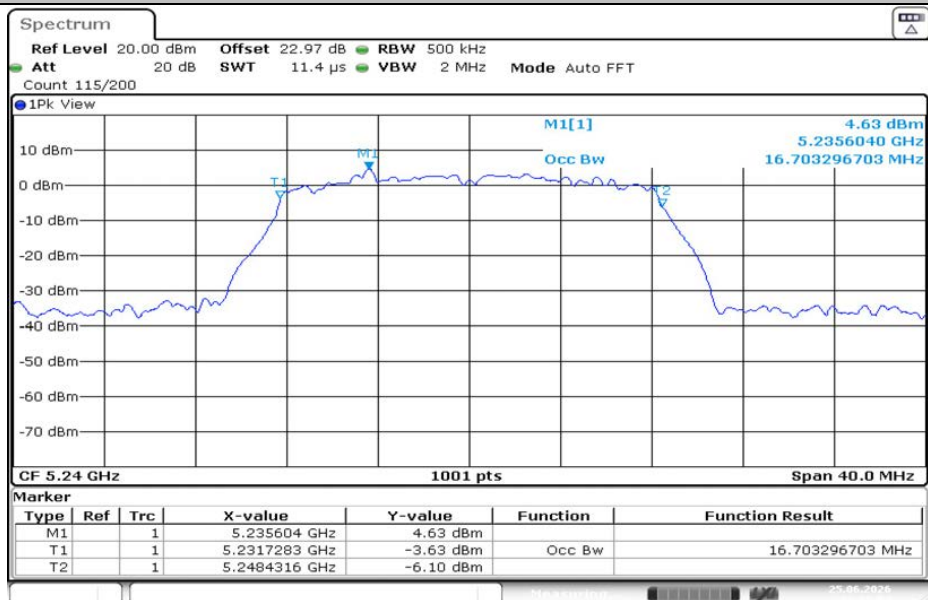
11A-CDD-Ant2-5240
