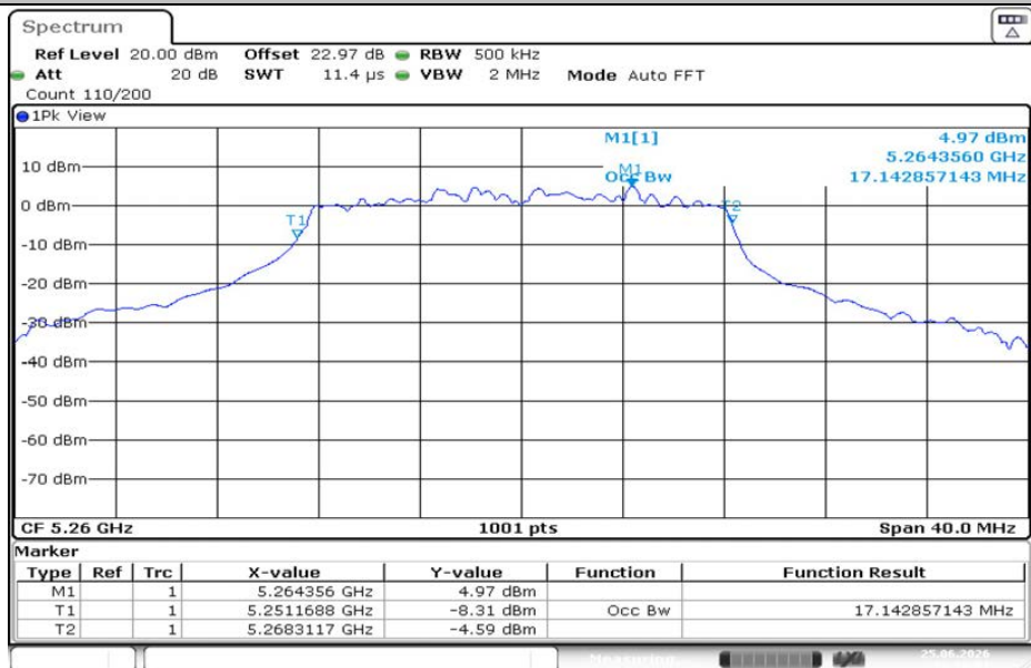
11A-CDD-Ant2-5260
