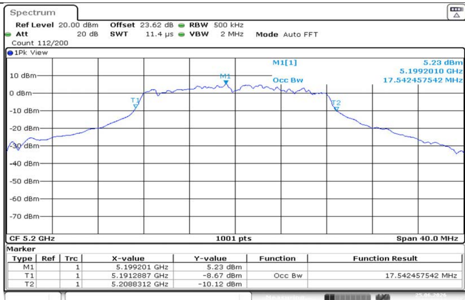
11A-CDD-Ant1-5200
