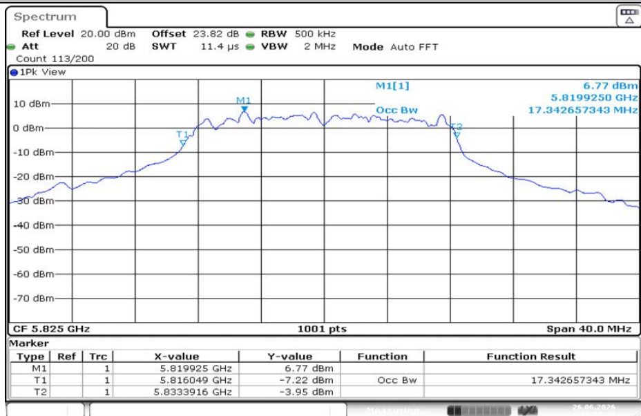
11A-CDD-Ant2-5825
