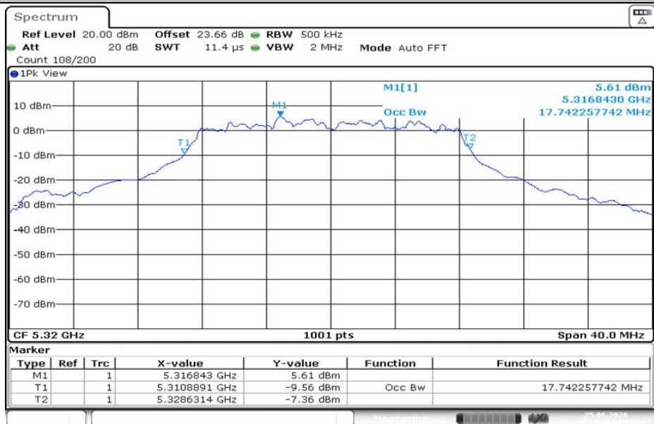
11A-CDD-Ant2-5320
