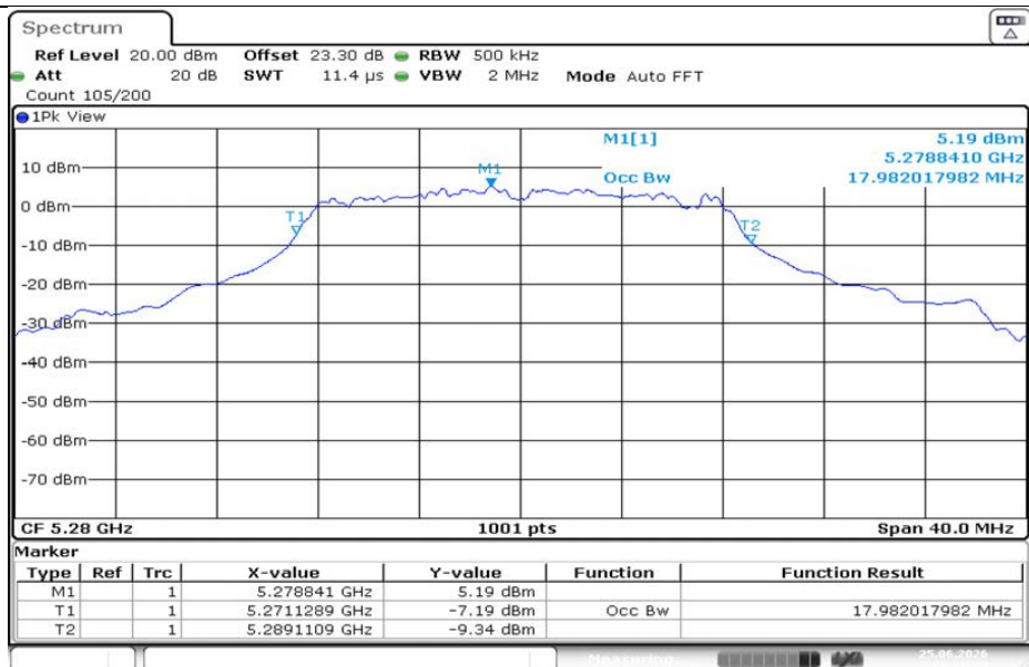
11A-CDD-Ant1-5280
