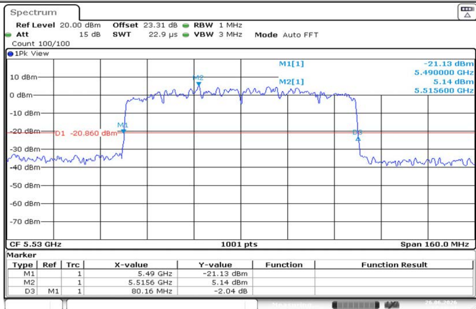
11AX80MIMO-Ant2-5530
