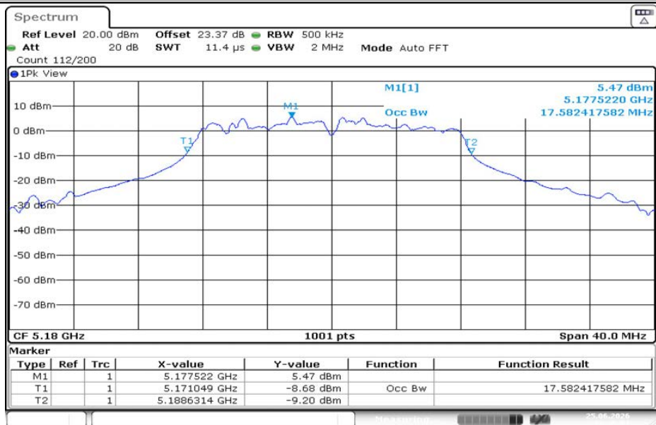
11A-CDD-Ant2-5180
