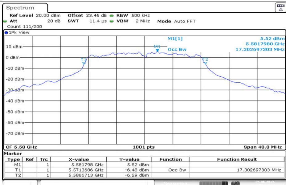
11A-CDD-Ant1-5580
