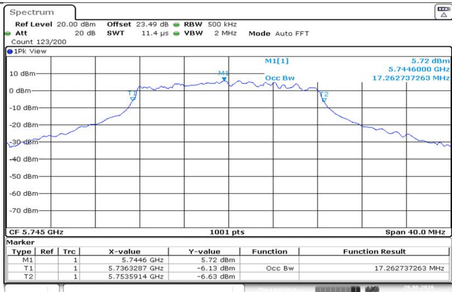
11A-CDD-Ant1-5745
