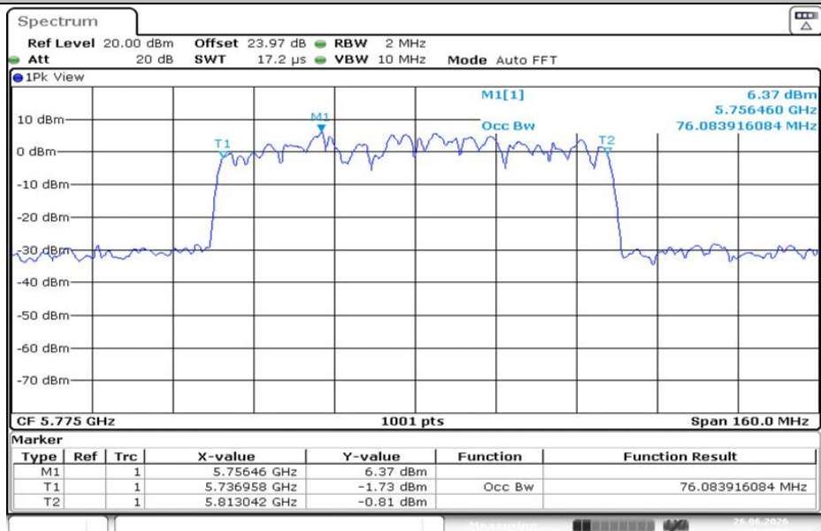
11AC80MIMO-Ant2-5775
