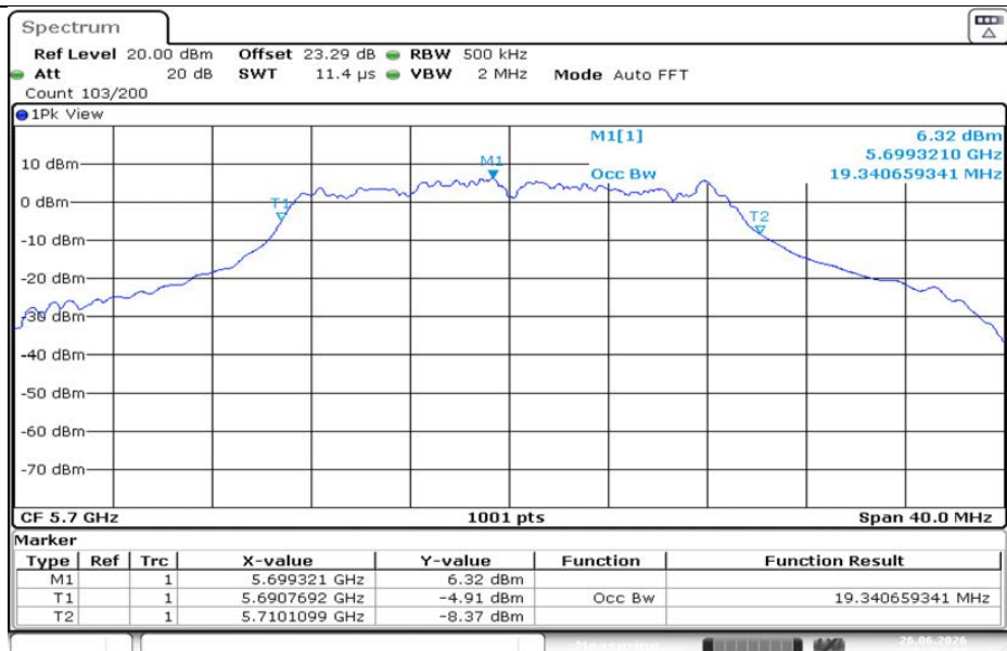
11AC20MIMO-Ant1-5700
