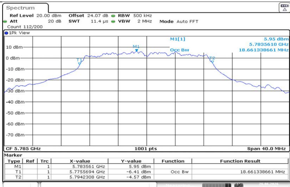
11N20MIMO-Ant1-5785
