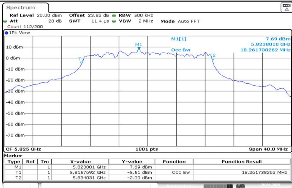
11AC20MIMO-Ant2-5825
