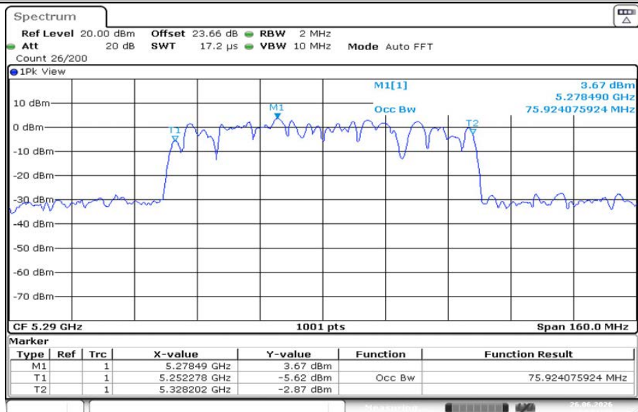
11AC80MIMO-Ant2-5290
