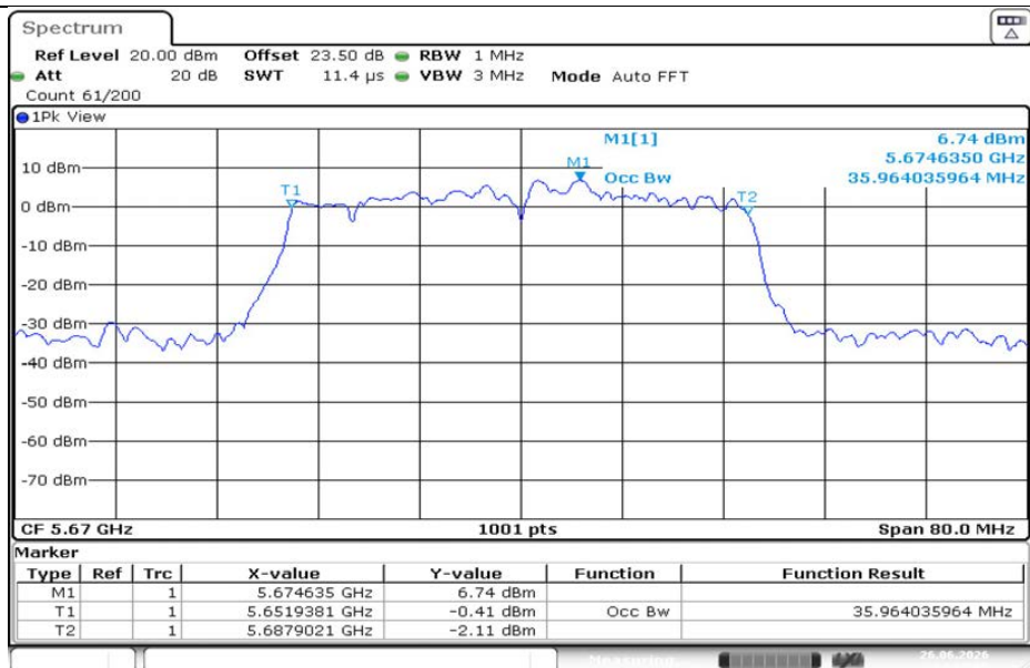
11AC40MIMO-Ant1-5670
