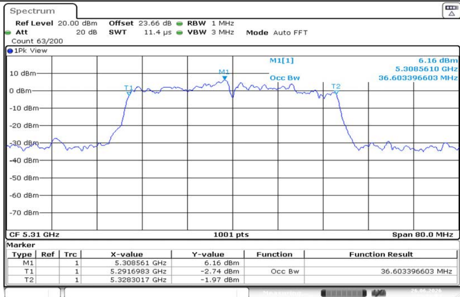
11AC40MIMO-Ant2-5310
