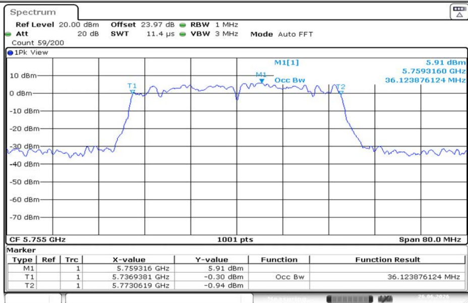
11AC40MIMO-Ant2-5755
