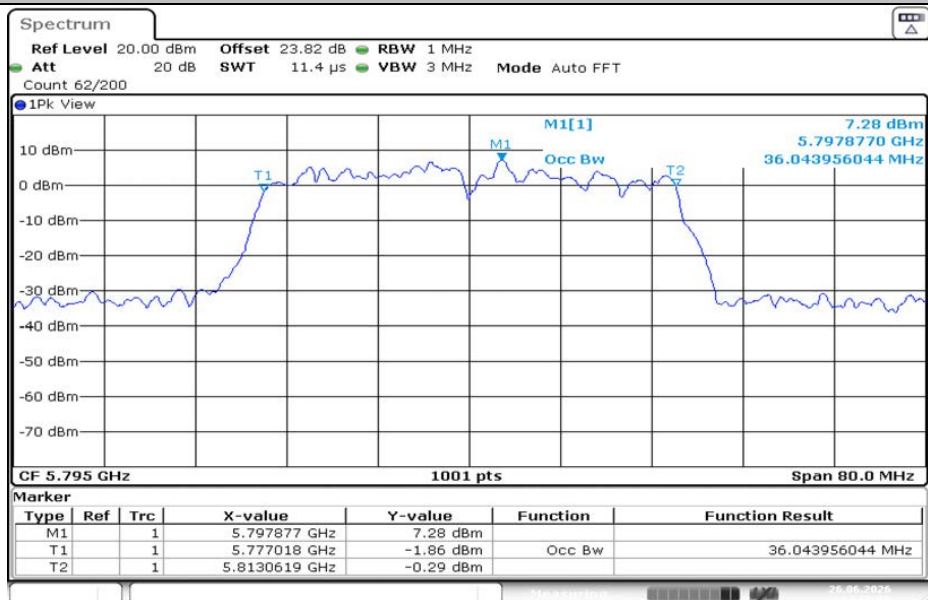
11AC40MIMO-Ant2-5795
