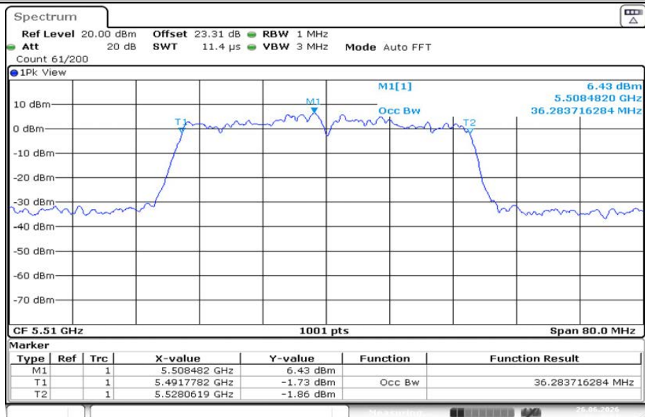
11N40MIMO-Ant2-5510
