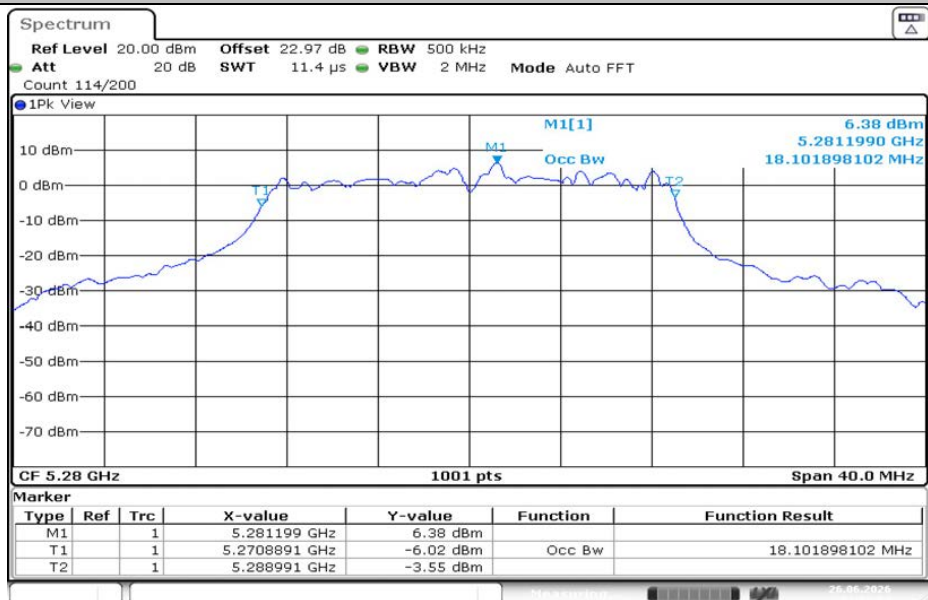
11AC20MIMO-Ant2-5280
