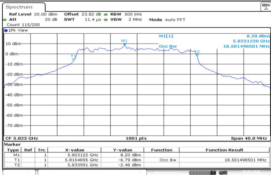
11N20MIMO-Ant2-5825
