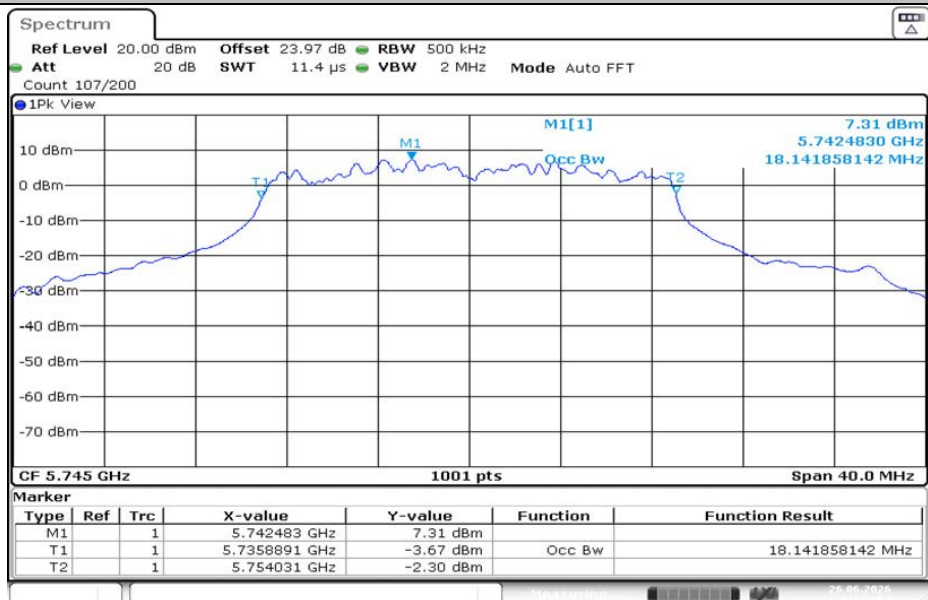
11AC20MIMO-Ant2-5745
