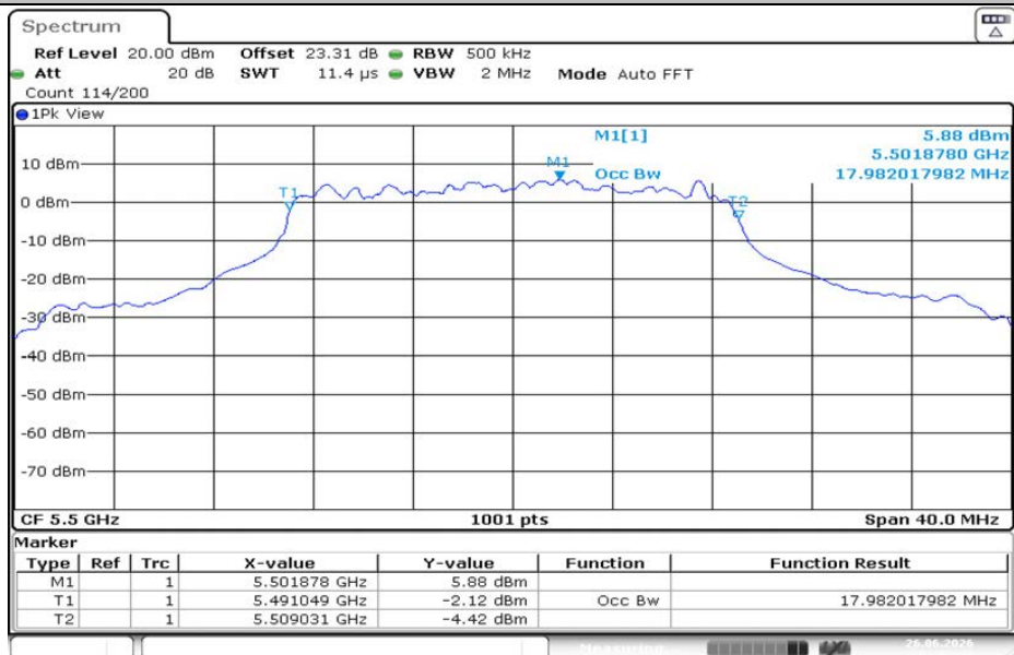
11AC20MIMO-Ant2-5500
