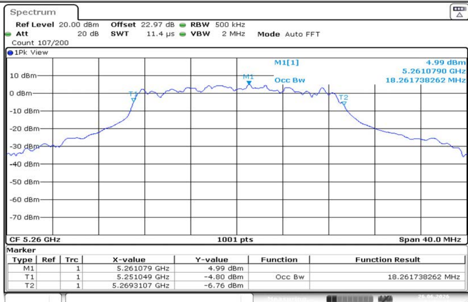
11AC20MIMO-Ant2-5260
