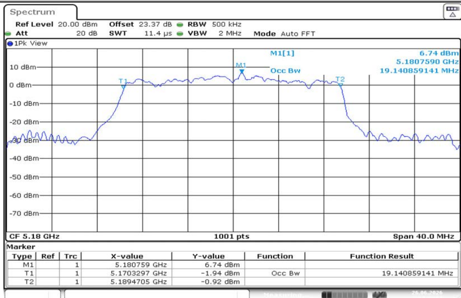
11AX20MIMO-Ant2-5180
