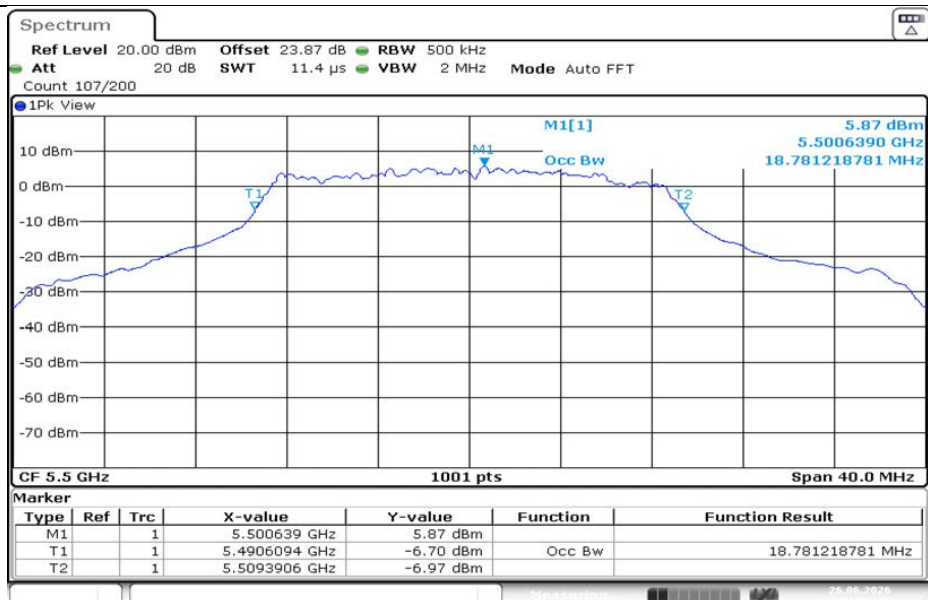
11AC20MIMO-Ant1-5500
