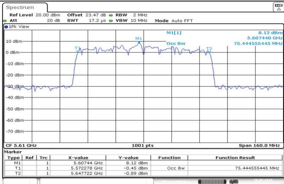
11AC80MIMO-Ant2-5610
