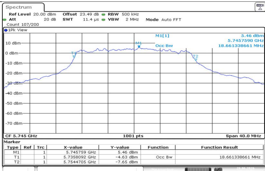
11AC20MIMO-Ant1-5745
