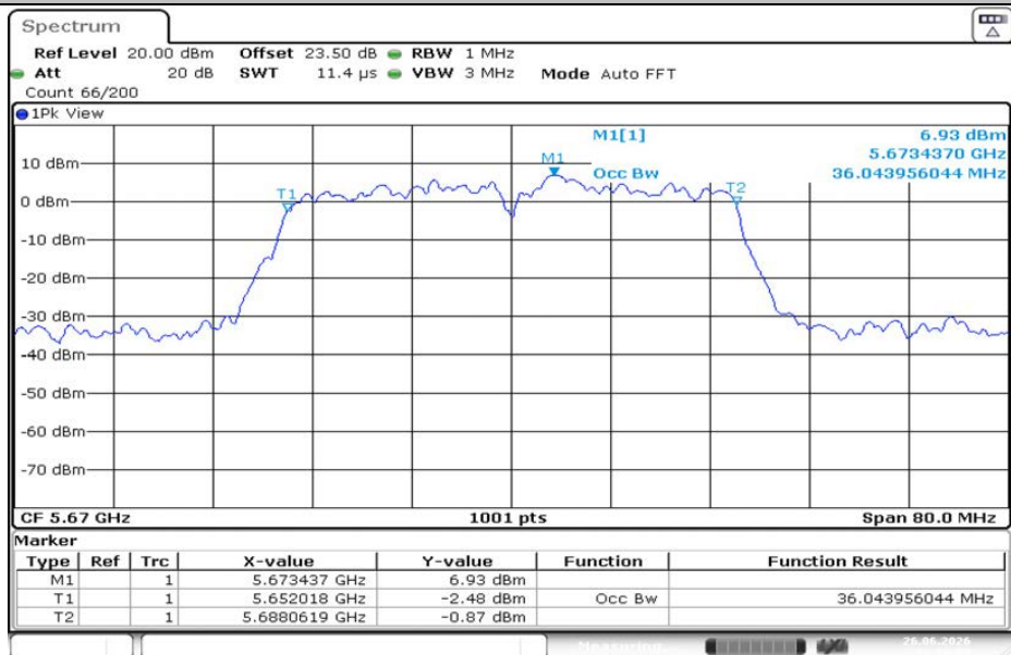
11N40MIMO-Ant2-5670
