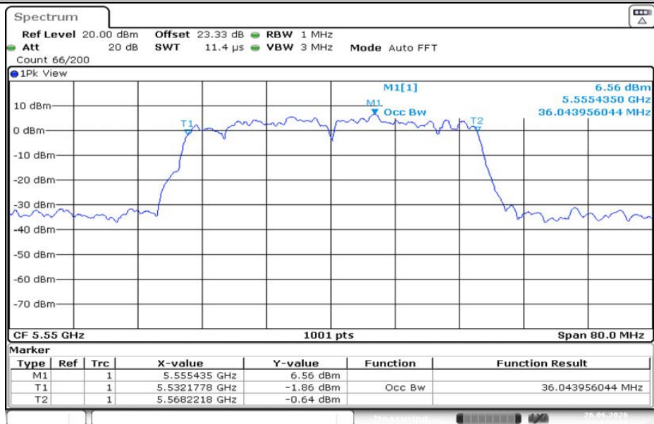
11AC40MIMO-Ant2-5550
