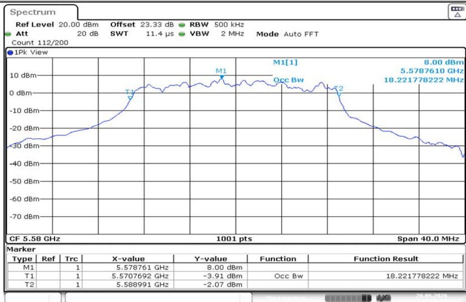
11N20MIMO-Ant2-5580
