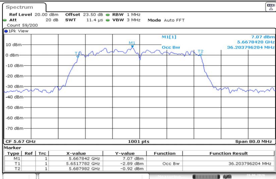
11AC40MIMO-Ant2-5670
