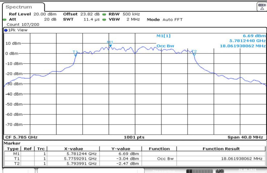
11AC20MIMO-Ant2-5785
