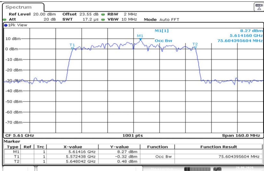
11AC80MIMO-Ant1-5610
