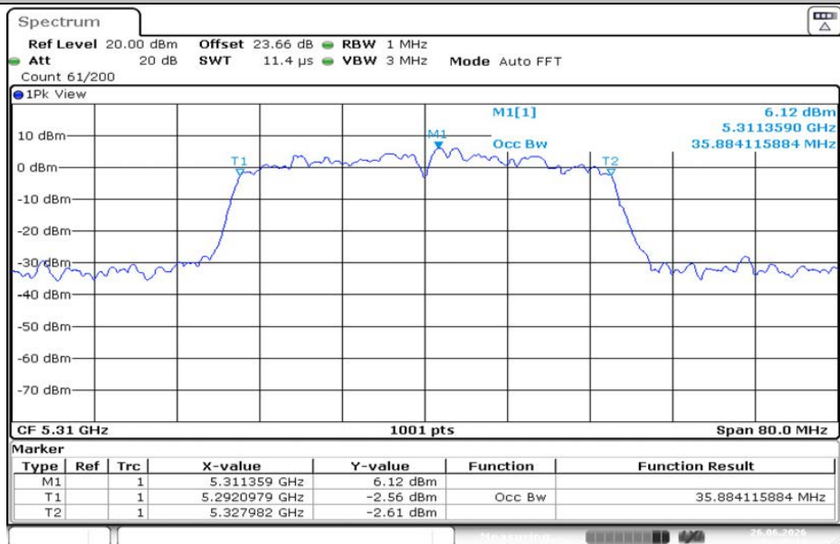
11N40MIMO-Ant2-5310
