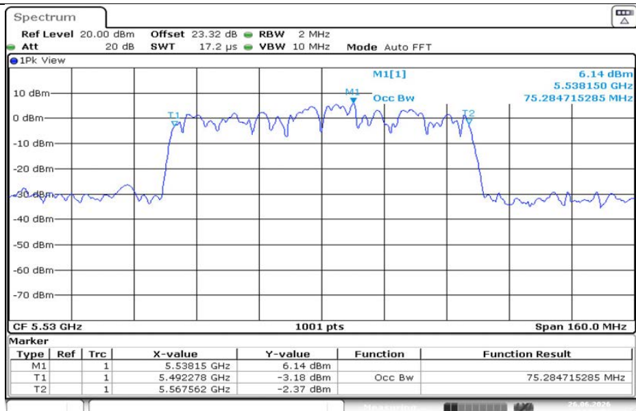
11AC80MIMO-Ant1-5530
