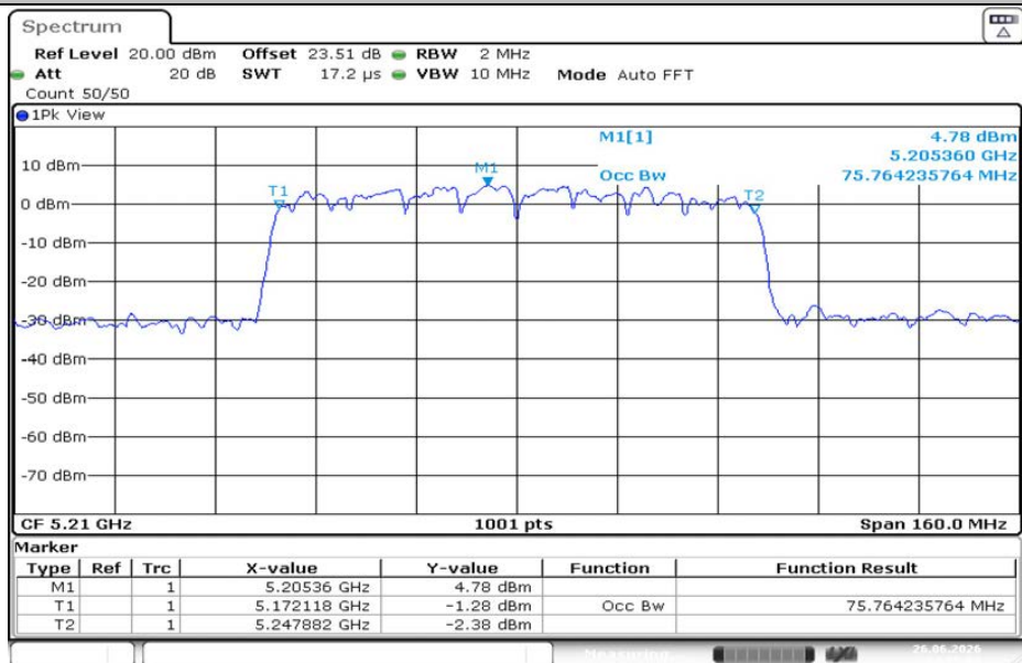
11AC80MIMO-Ant2-5210
