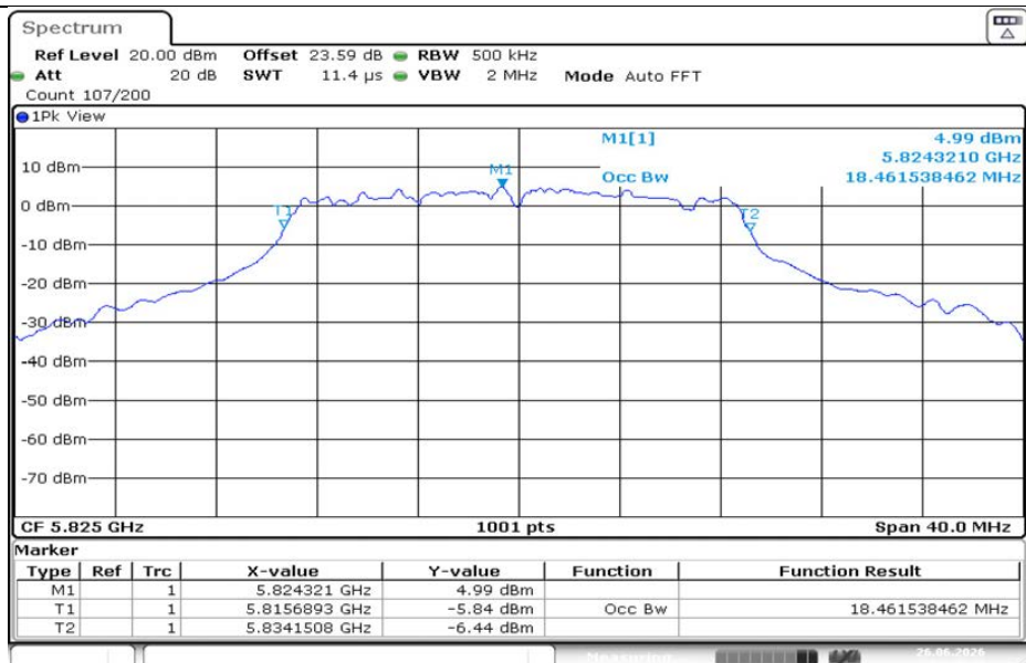
11AC20MIMO-Ant1-5825
