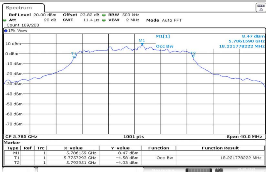
11N20MIMO-Ant1-5785
