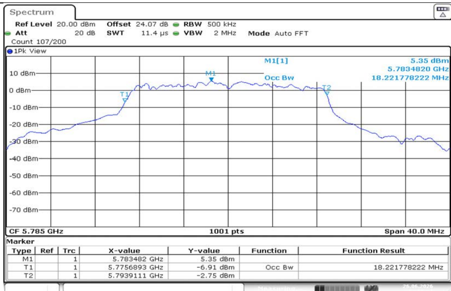
11AC20MIMO-Ant1-5785
