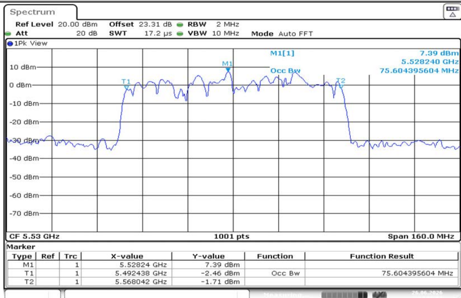
11AC80MIMO-Ant2-5530
