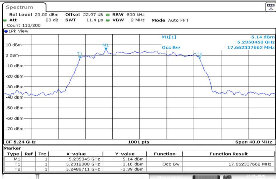
11AC20MIMO-Ant2-5240
