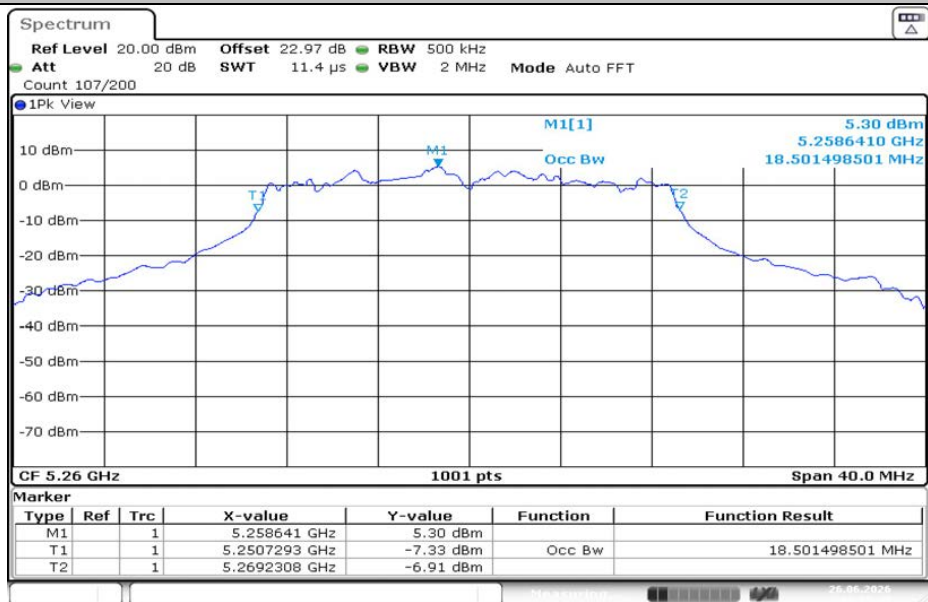
11N20MIMO-Ant2-5260
