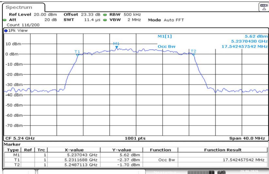
11AC20MIMO-Ant1-5240
