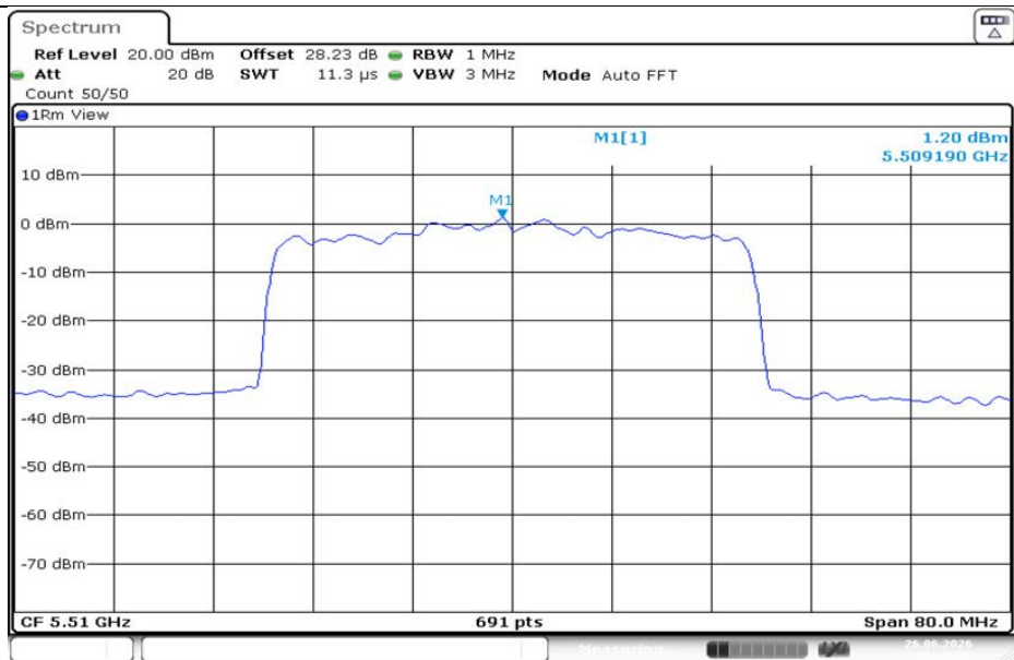
11AX40MIMO-Ant1-5510-PASS
