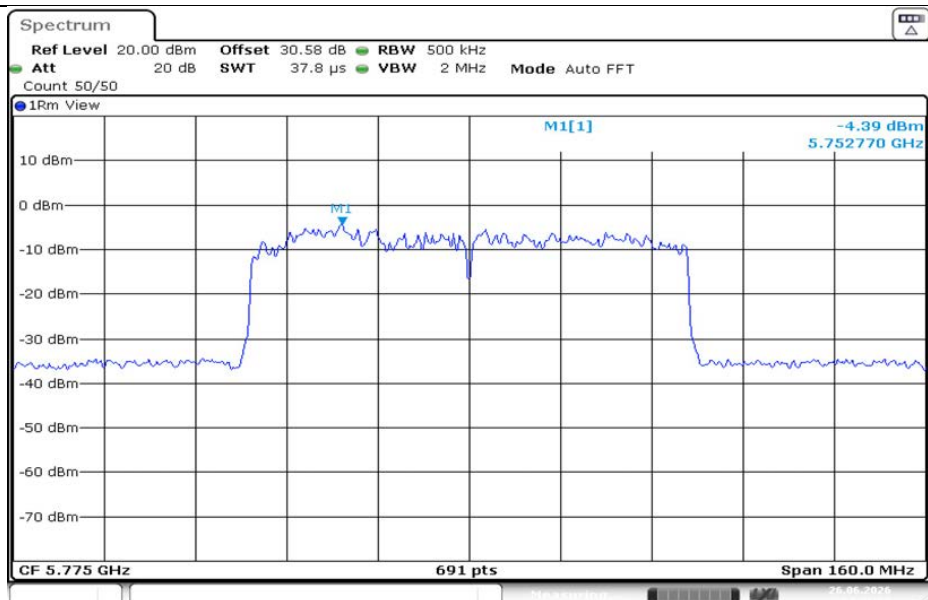
11AC80MIMO-Ant1-5775-PASS
