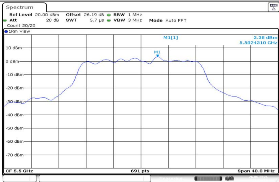
11AC20MIMO-Ant2-5500-PASS
