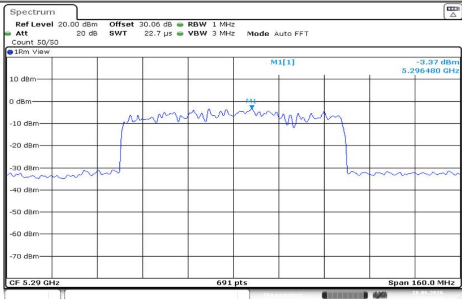
11AX80MIMO-Ant2-5290-PASS
