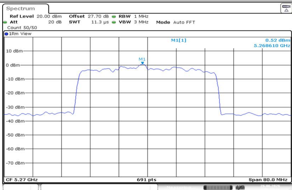
11AX40MIMO-Ant2-5270-PASS
