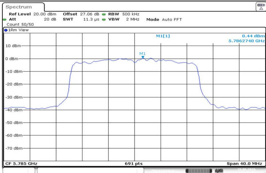
11AX20MIMO-Ant2-5785-PASS
