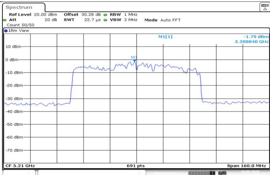
11AC80MIMO-Ant1-5210-PASS
