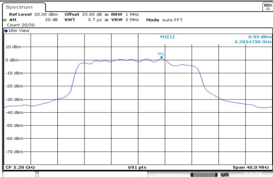
11AC20MIMO-Ant2-5280-PASS
