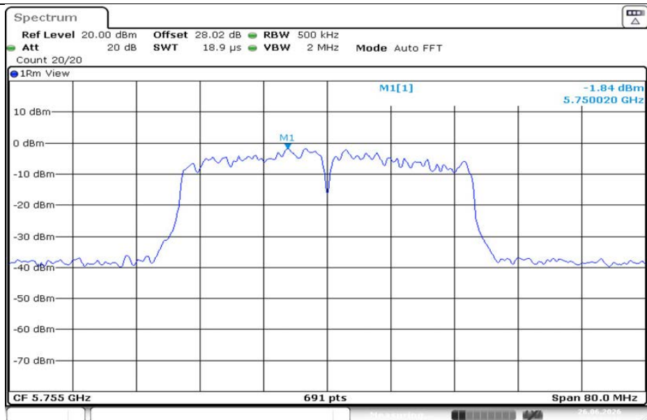
11AC40MIMO-Ant1-5755-PASS
