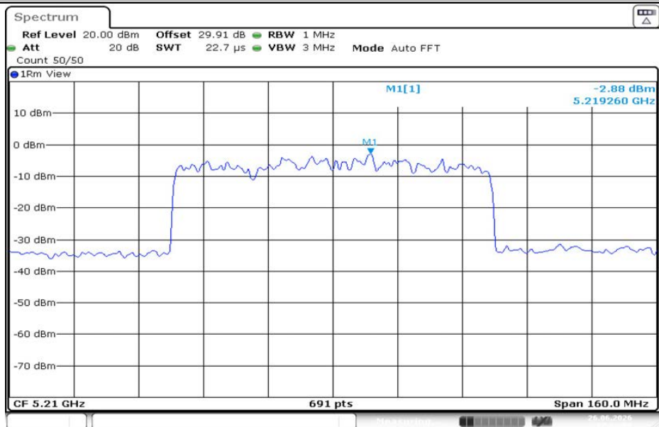
11AX80MIMO-Ant2-5210-PASS
