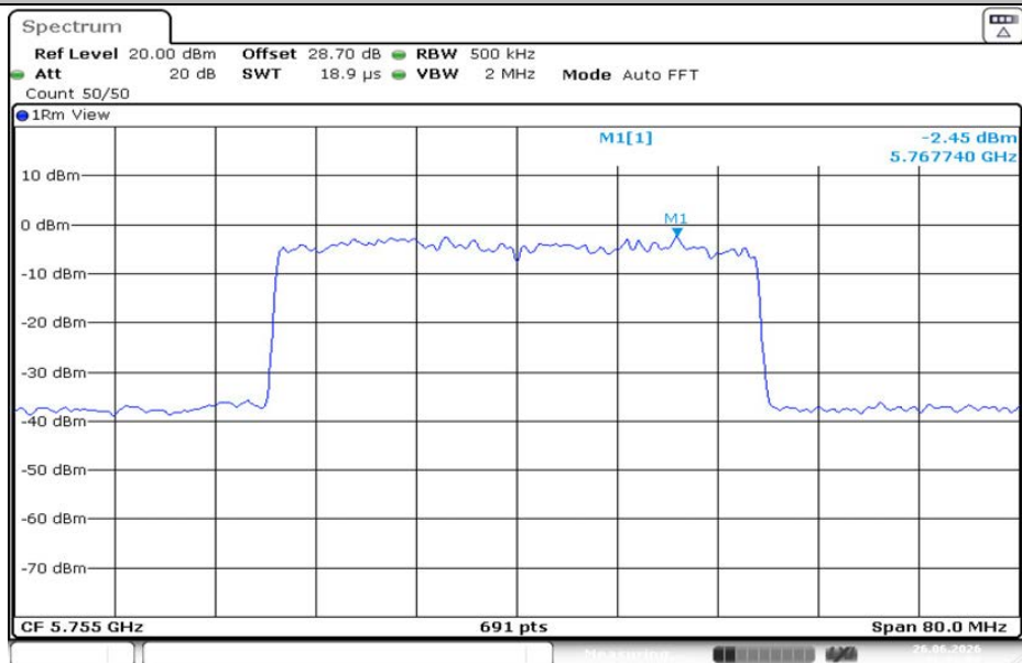
11AX40MIMO-Ant2-5755-PASS
