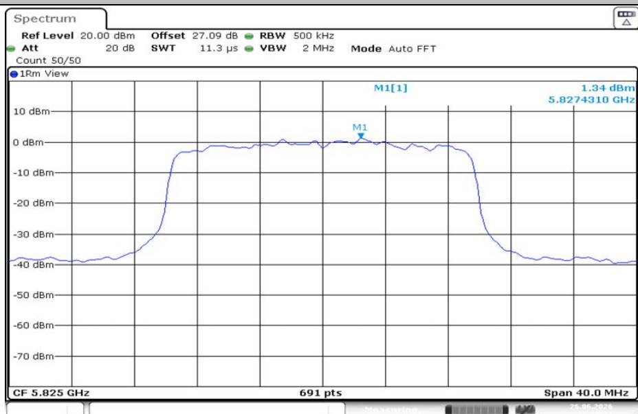
11AX20MIMO-Ant1-5825-PASS
