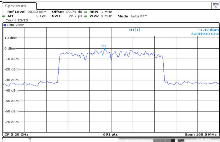
11AC80MIMO-Ant1-5290-PASS
