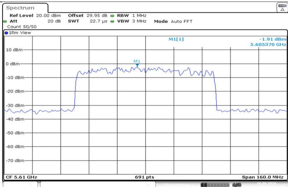
11AX80MIMO-Ant1-5610-PASS
