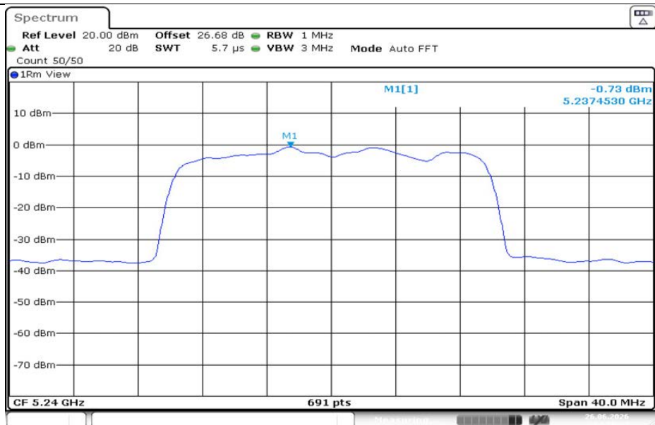
11AX20MIMO-Ant1-5240-PASS
