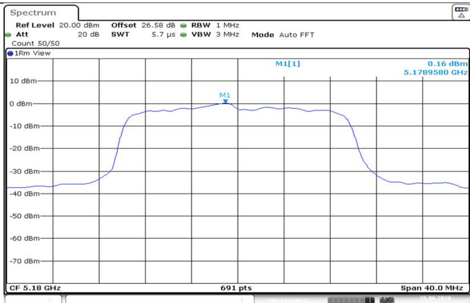
11AX20MIMO-Ant1-5180-PASS
