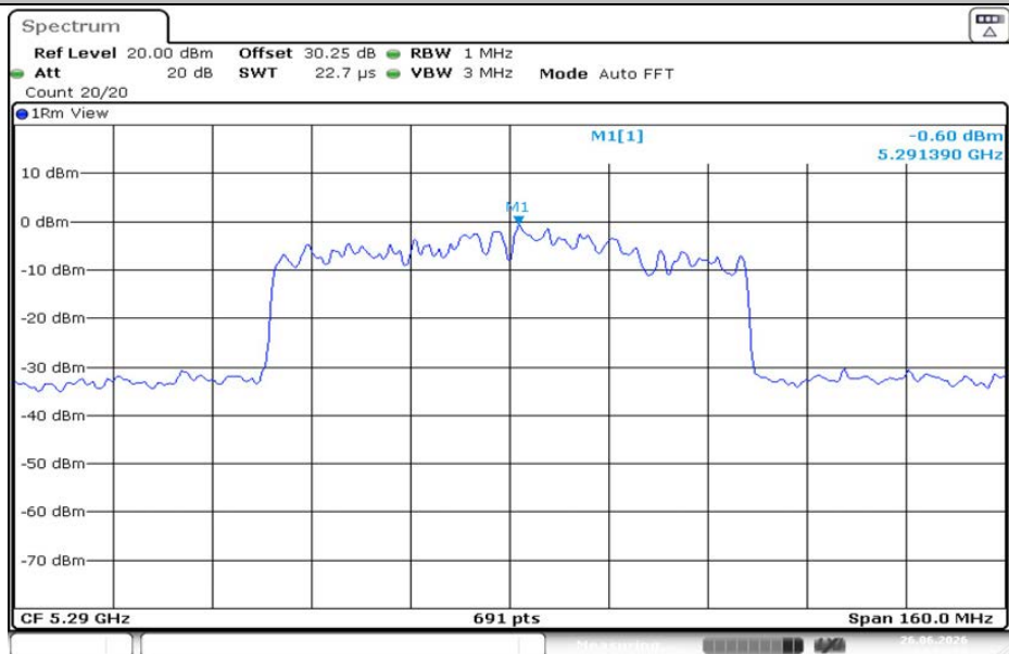
11AC80MIMO-Ant2-5290-PASS
