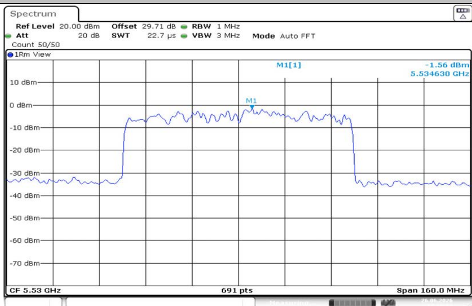
11AX80MIMO-Ant1-5530-PASS
