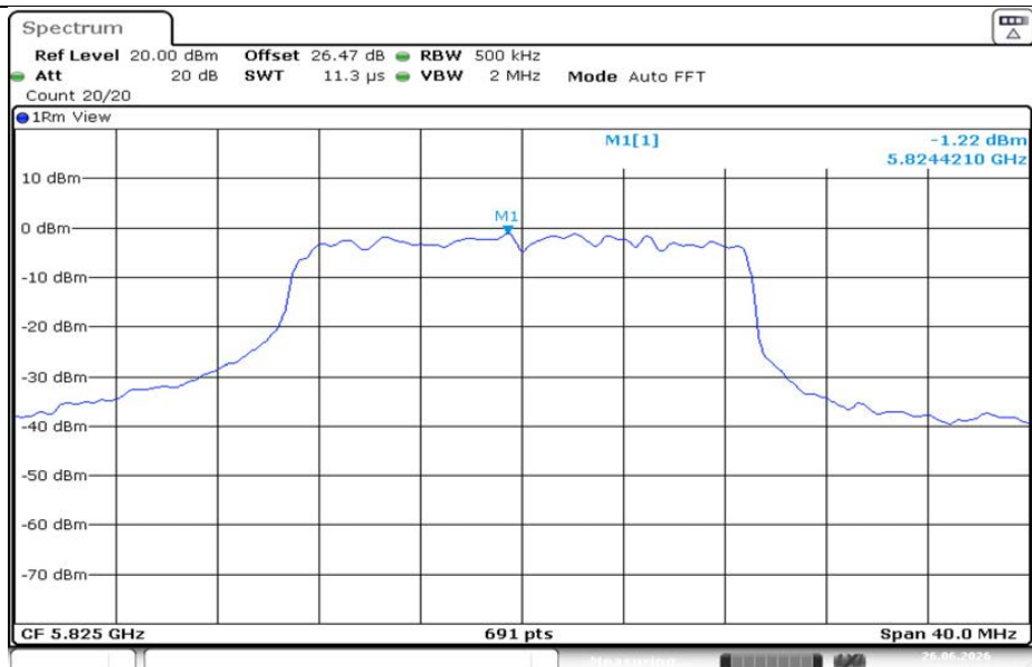
11AC20MIMO-Ant1-5825-PASS
