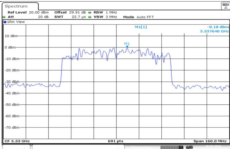
11AC80MIMO-Ant1-5530-PASS
