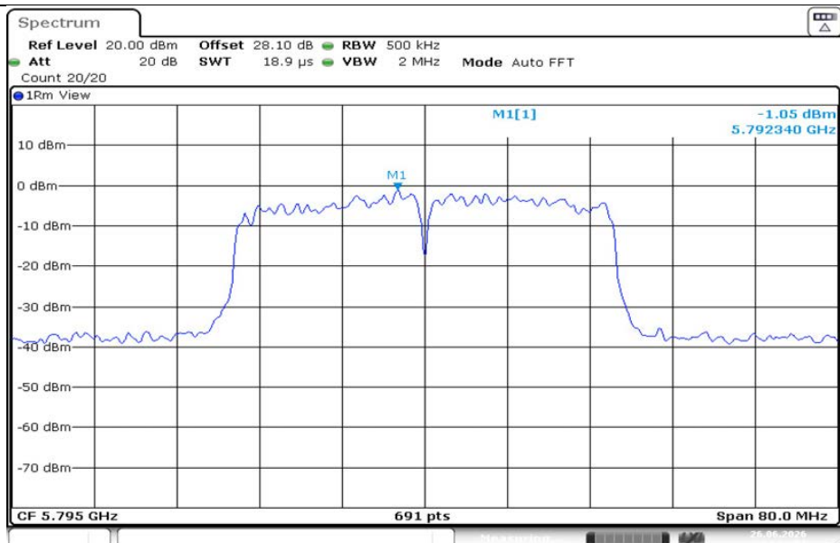
11AC40MIMO-Ant1-5795-PASS
