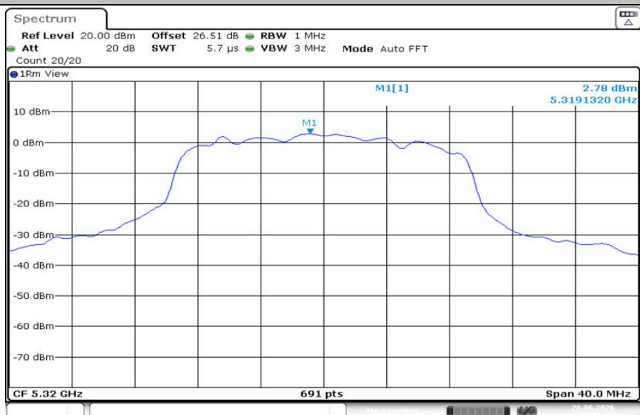
11AC20MIMO-Ant1-5320-PASS
