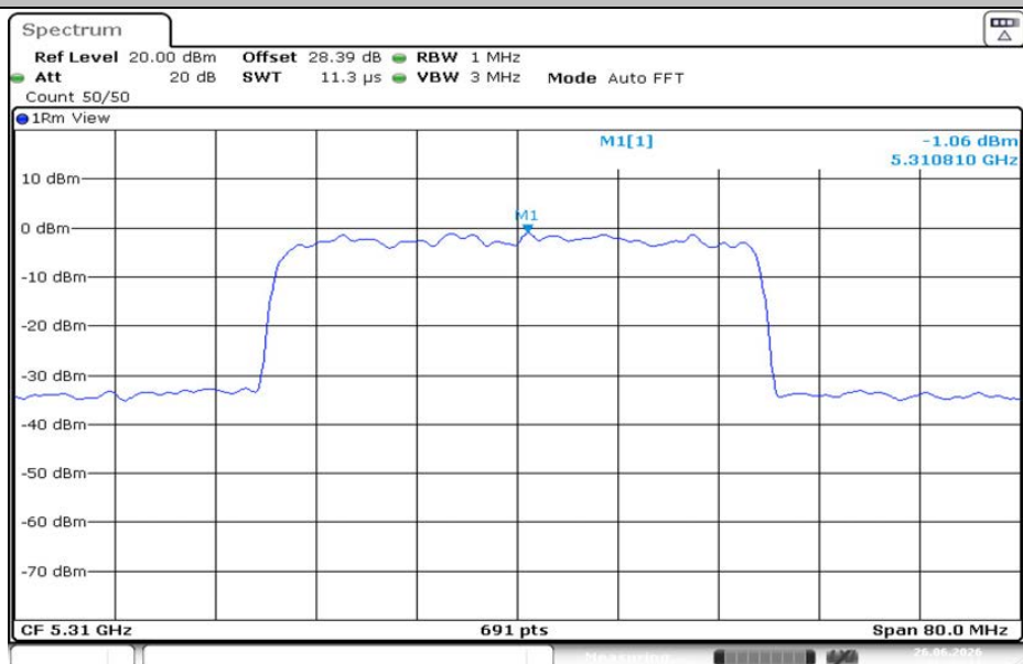
11AX40MIMO-Ant1-5310-PASS
