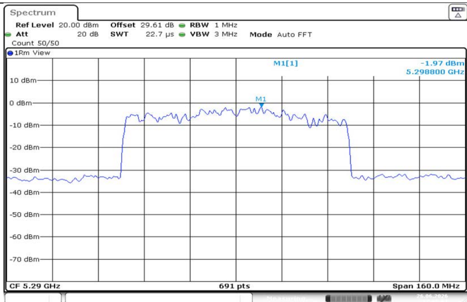
11AX80MIMO-Ant1-5290-PASS
