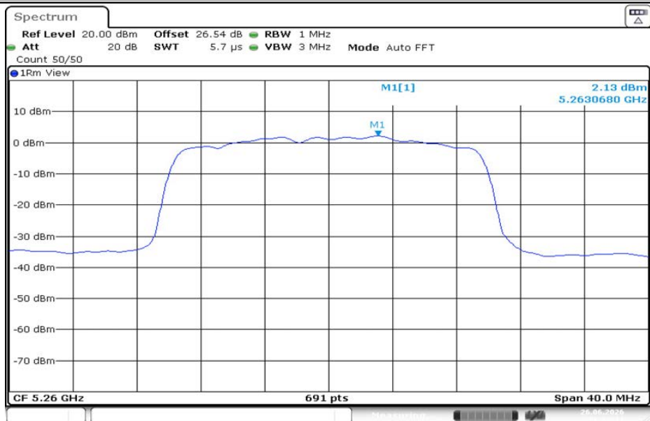
11AX20MIMO-Ant2-5260-PASS
