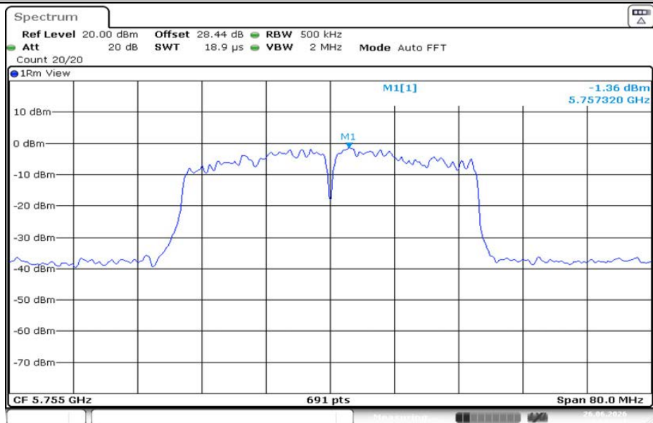
11AC40MIMO-Ant2-5755-PASS
