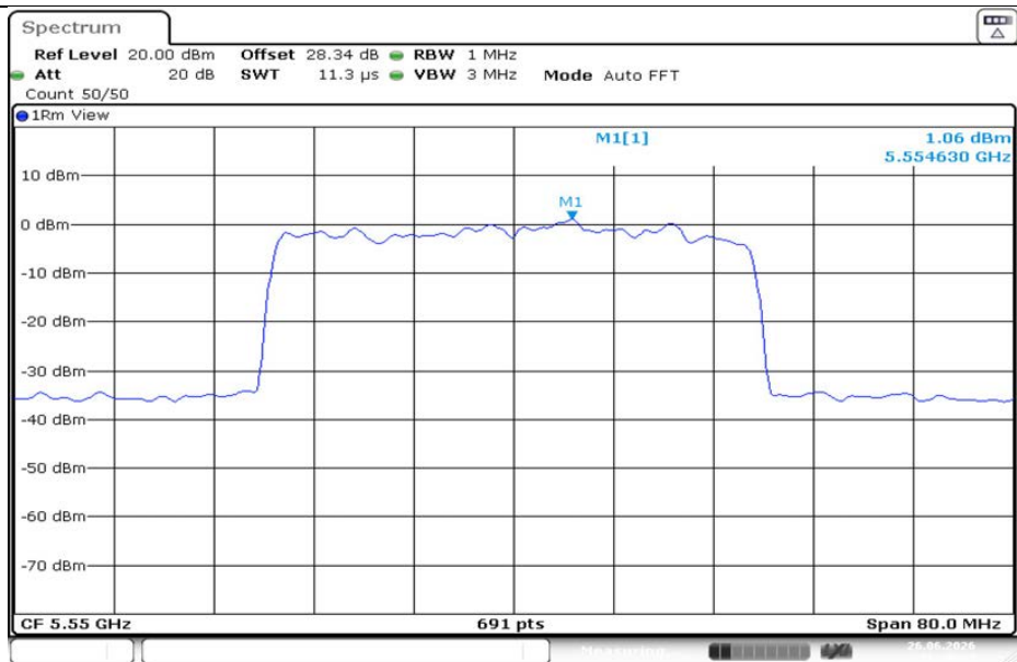
11AX40MIMO-Ant1-5550-PASS
