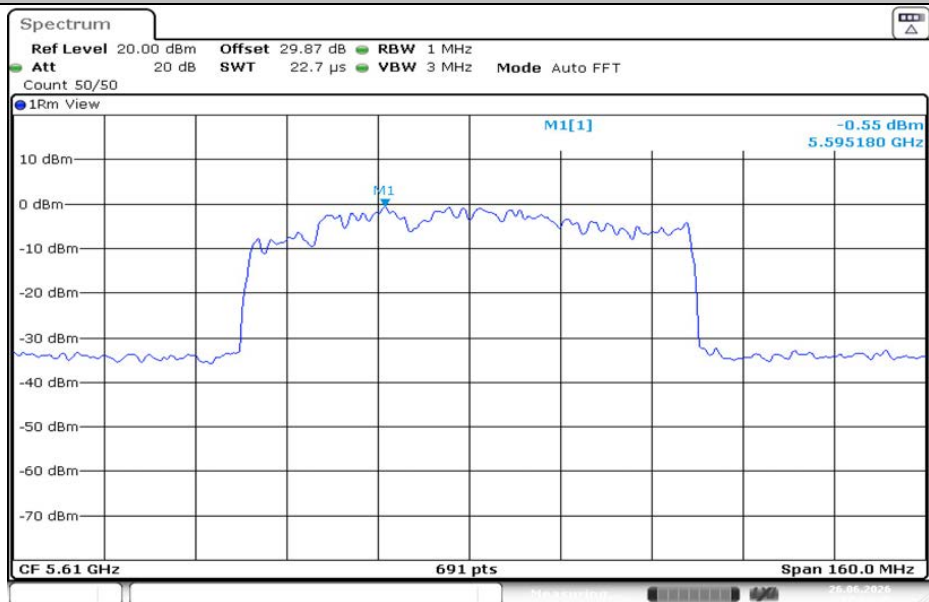
11AX80MIMO-Ant2-5610-PASS
