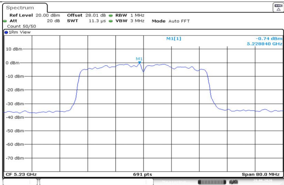
11AC40MIMO-Ant1-5230-PASS
