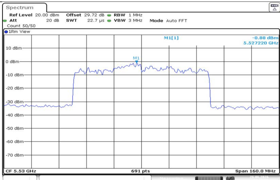
11AX80MIMO-Ant1-5530-PASS
