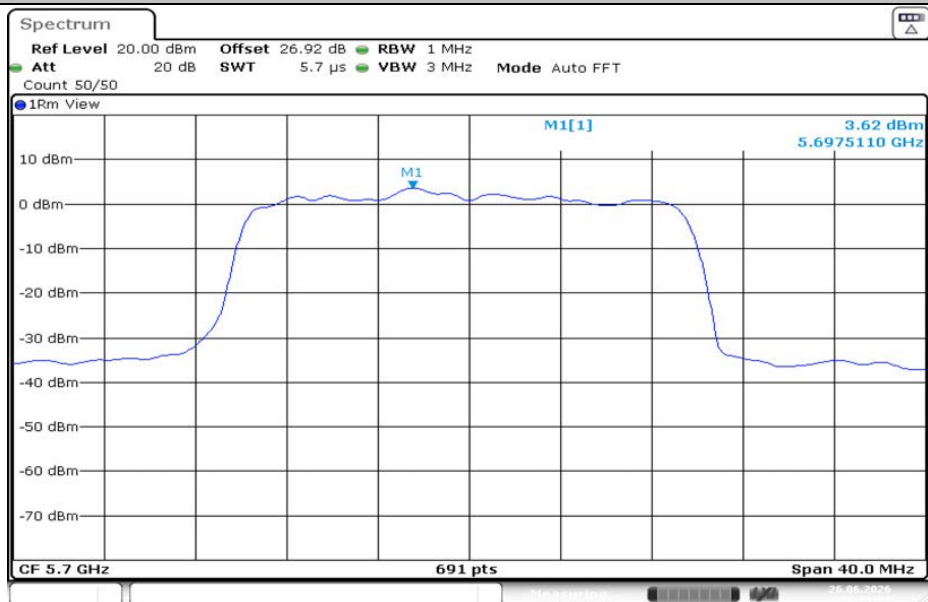
11AX20MIMO-Ant2-5700-PASS
