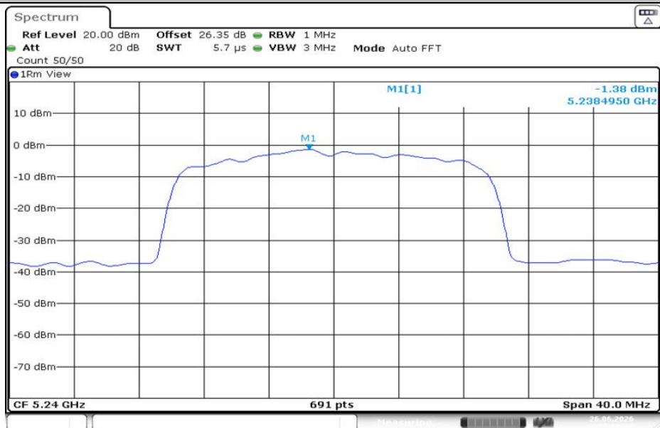
11AX20MIMO-Ant2-5240-PASS
