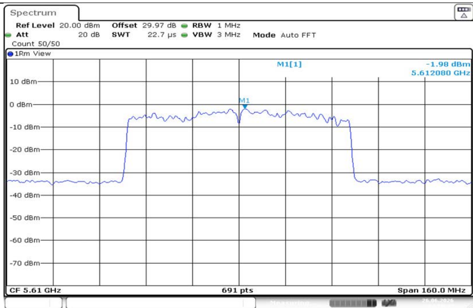
11AC80MIMO-Ant1-5610-PASS
