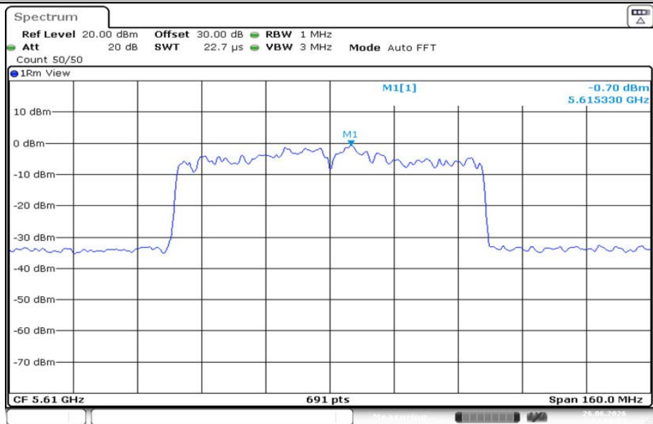
11AC80MIMO-Ant2-5610-PASS
