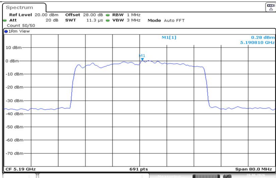
11AX40MIMO-Ant1-5190-PASS
