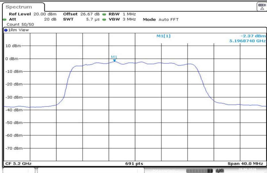
11AX20MIMO-Ant2-5200-PASS
