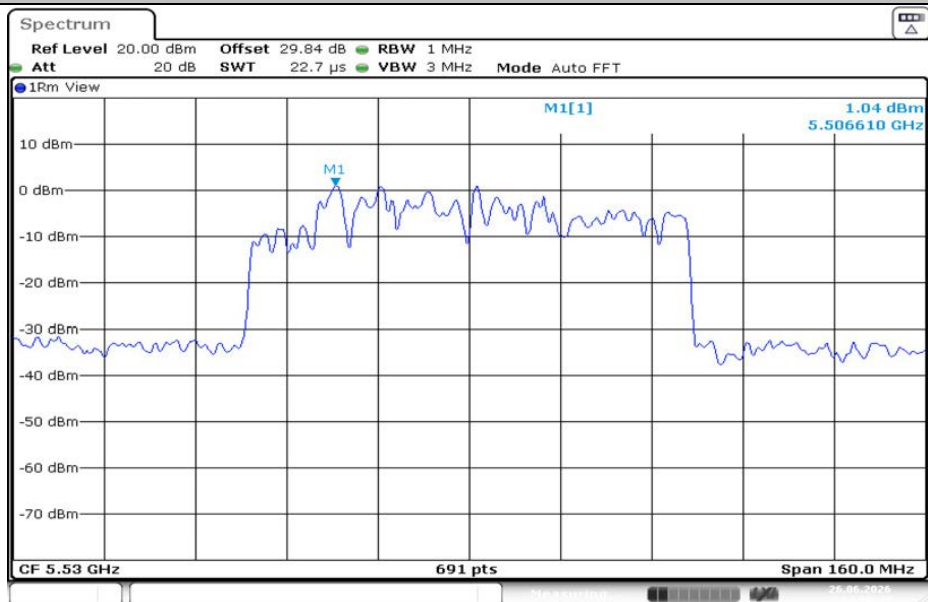
11AC80MIMO-Ant2-5530-PASS
