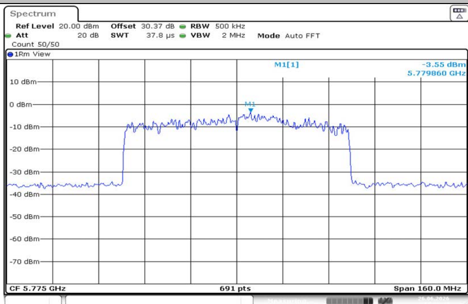
11AX80MIMO-Ant1-5775-PASS
