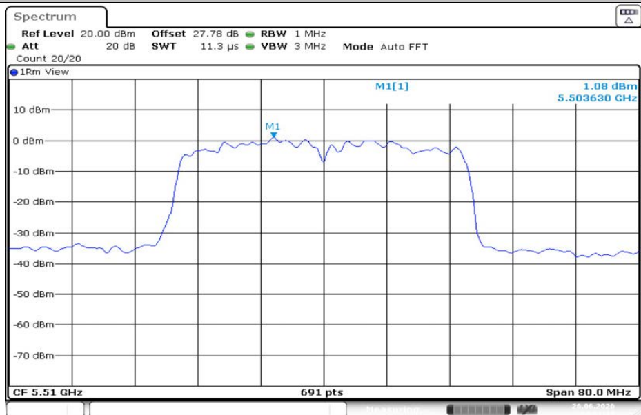
11AC40MIMO-Ant2-5510-PASS
