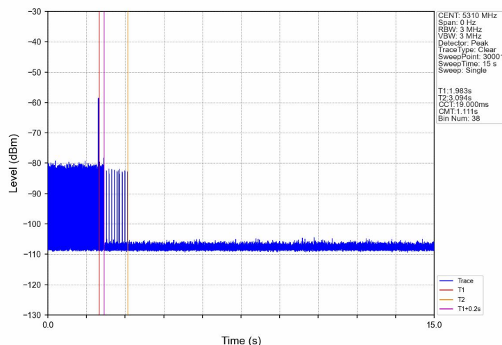
Channel Move Time and Closing Transmission Time_802.11ax(HEW40)_5310MHz
