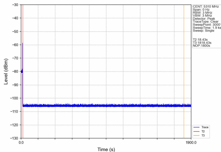
Non-Occupancy Period_802.11ax(HEW40)_5310MHz
