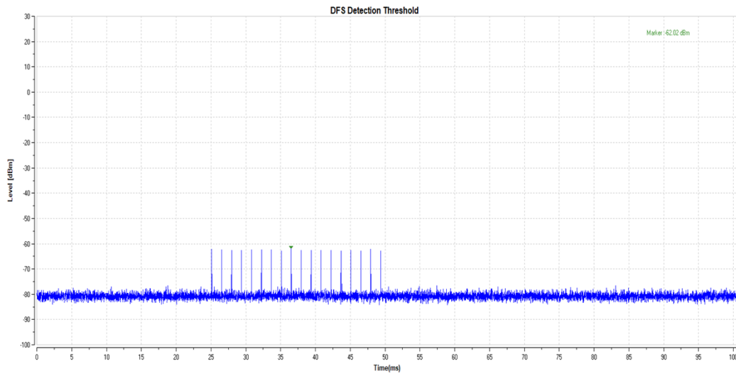
Radar Burst Level at -62dBm: Radar Type 0
