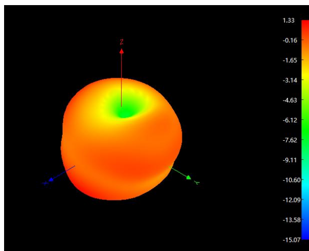
Pictrue 1 Antenna gain and radiation pattern measurement
