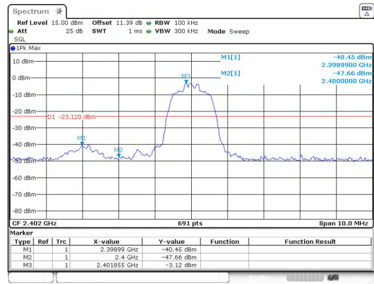
Out Of Band Emission π/4DQPSK_2-DH5_Channel 0
