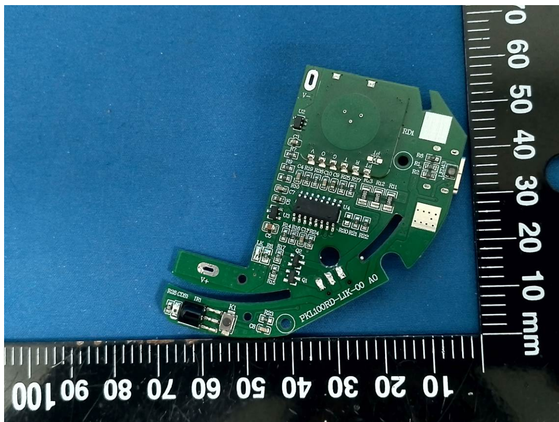
5.8G Radar Antenna
