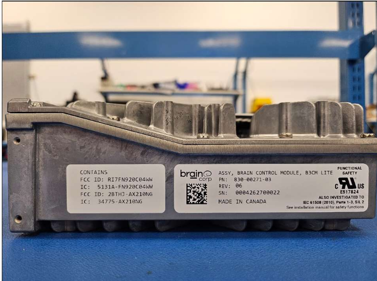
• Figure A.2: Physical Label Photograph – Model B3CM-L (P/N 830-00271-03)
