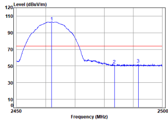
11b_TX_CH_11_Horizontal-Peak
