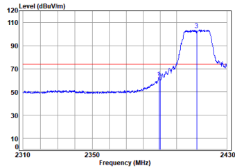
11g_TX_CH_01_Vertical-Peak
