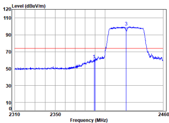
11n_HT(40M)_TX_CH_03_Vertical-Peak
