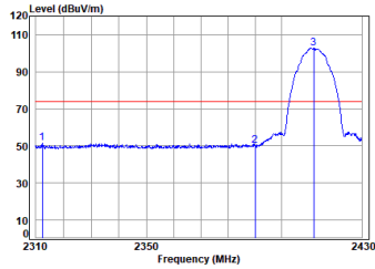
11b_TX_CH_01_Horizontal-Peak
