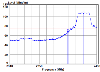
11g_TX_CH_01_Horizontal-Peak
