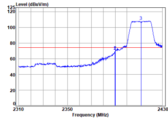
11n_HT(20M)_TX_CH_01_Horizontal-Peak
