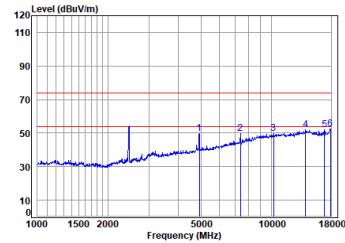
11g_TX_CH_11_Vertical
