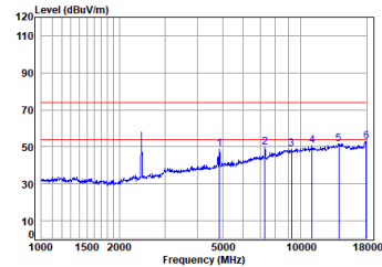
11g_TX_CH_06_Vertical
