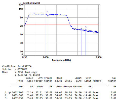
11n_HT(40M)_TX_CH_09_Vertical-Peak
