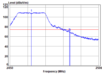
11g_TX_CH_11_Horizontal-Peak
