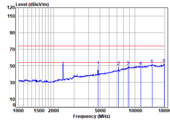
11g_TX_CH_01_Vertical
