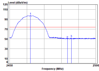
11b_TX_CH_11_Vertical-Peak
