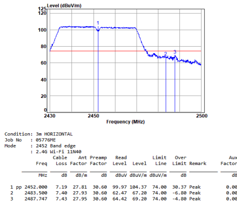
11n_HT(40M)_TX_CH_09_Horizontal-Peak
