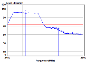
11n_HT(20M)_TX_CH_11_Vertical-Peak
