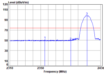
11b_TX_CH_01_Vertical-Peak
