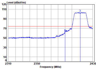
11n_HT(20M)_TX_CH_01_Vertical-Peak
