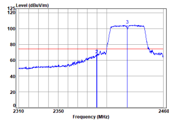
11n_HT(40M)_TX_CH_03_Horizontal-Peak
