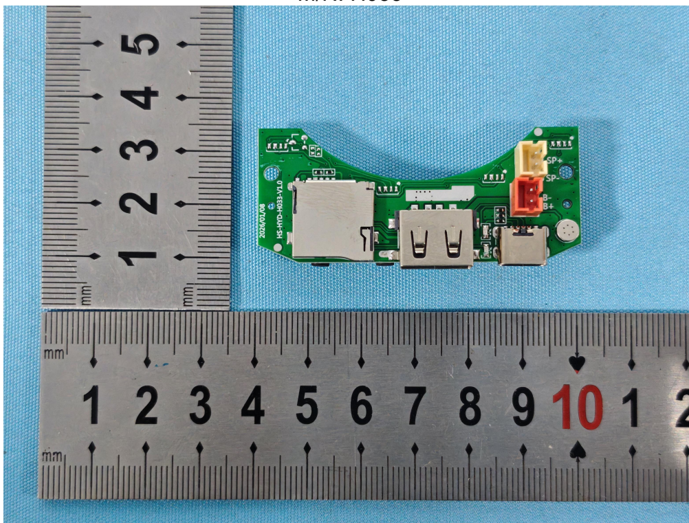
Photo 3 Internal photos of EUT M/N: H033
