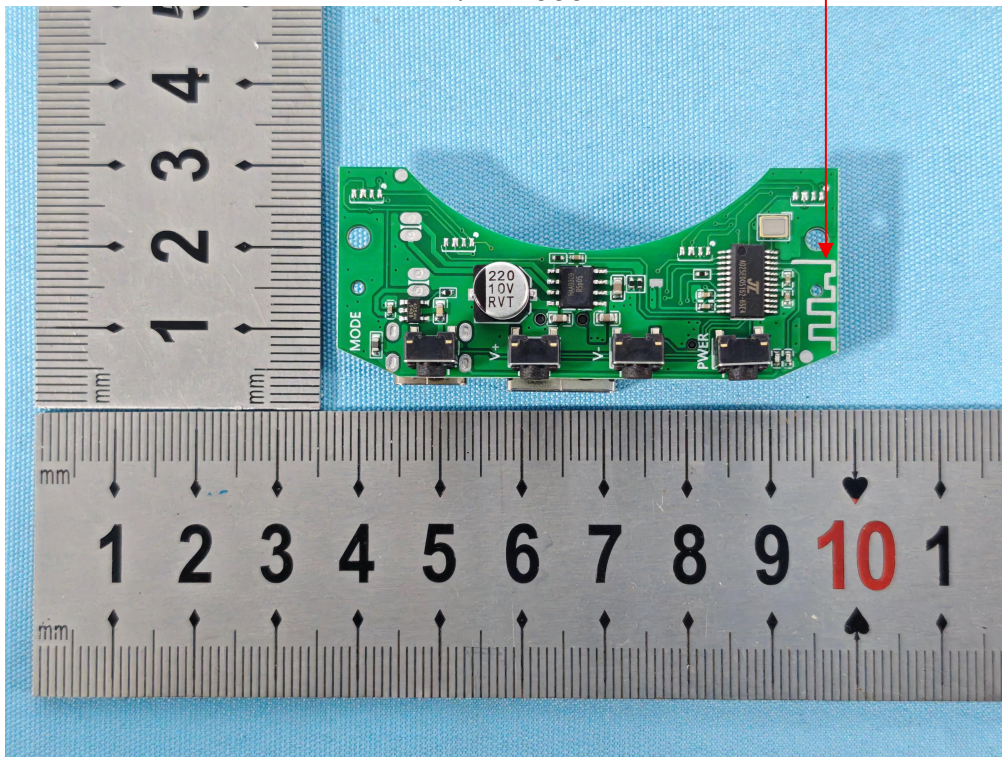
Photo 4 Internal photos of EUT M/N: H033
