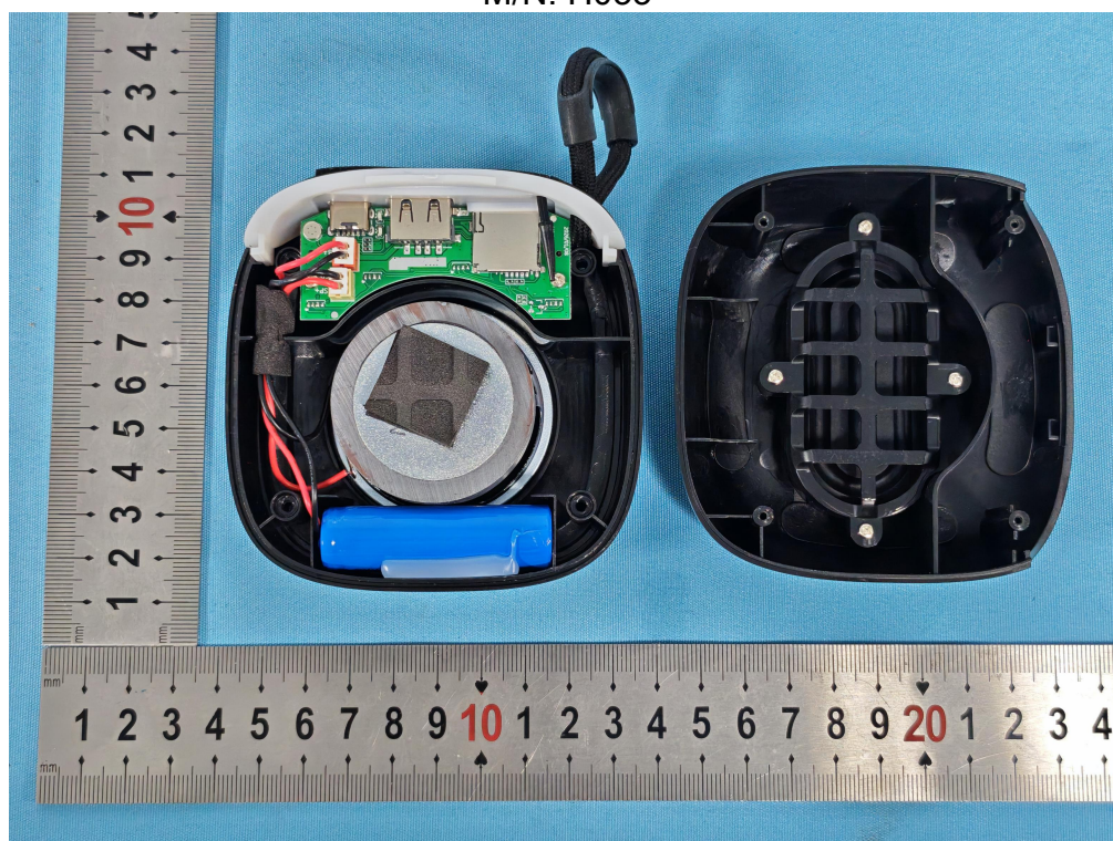
Photo 2 Internal photos of EUT M/N: H033
