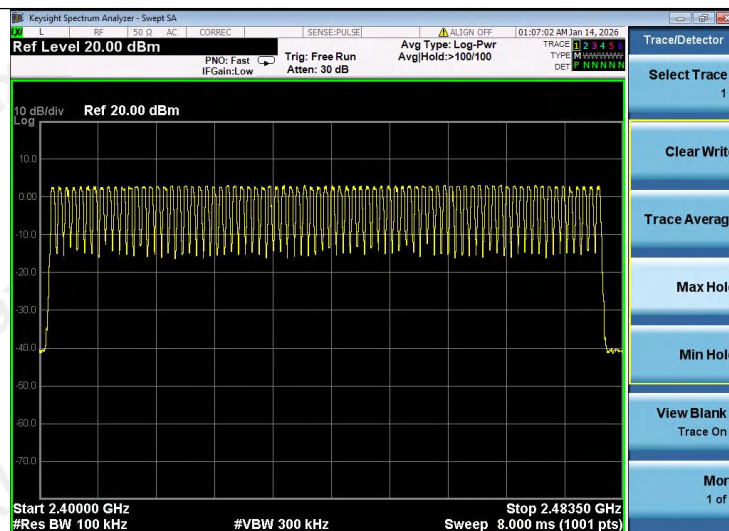
GFSK Modulation
