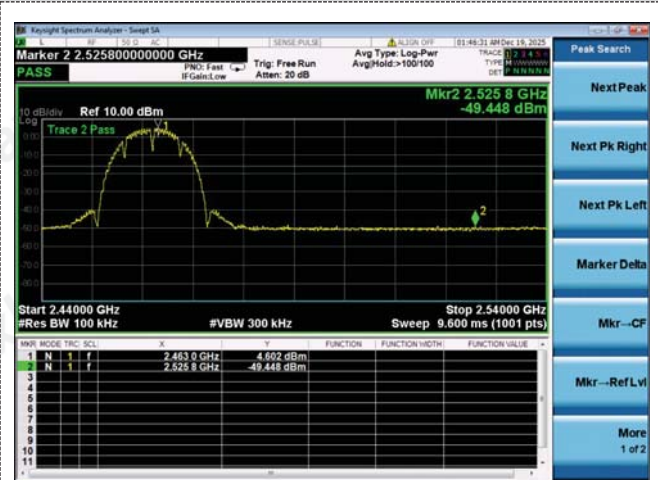
Right bandedge
