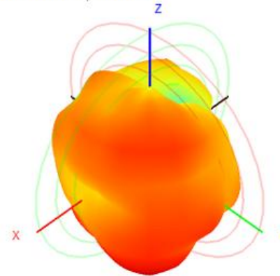
2450.0MHz H+V, Eff: 47.9%
