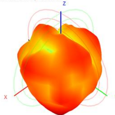
5550.0MHz H+V, Eff: 52.0%
