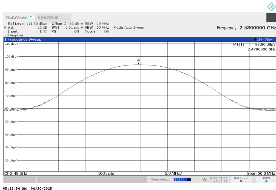
EIRP, Ch 26
