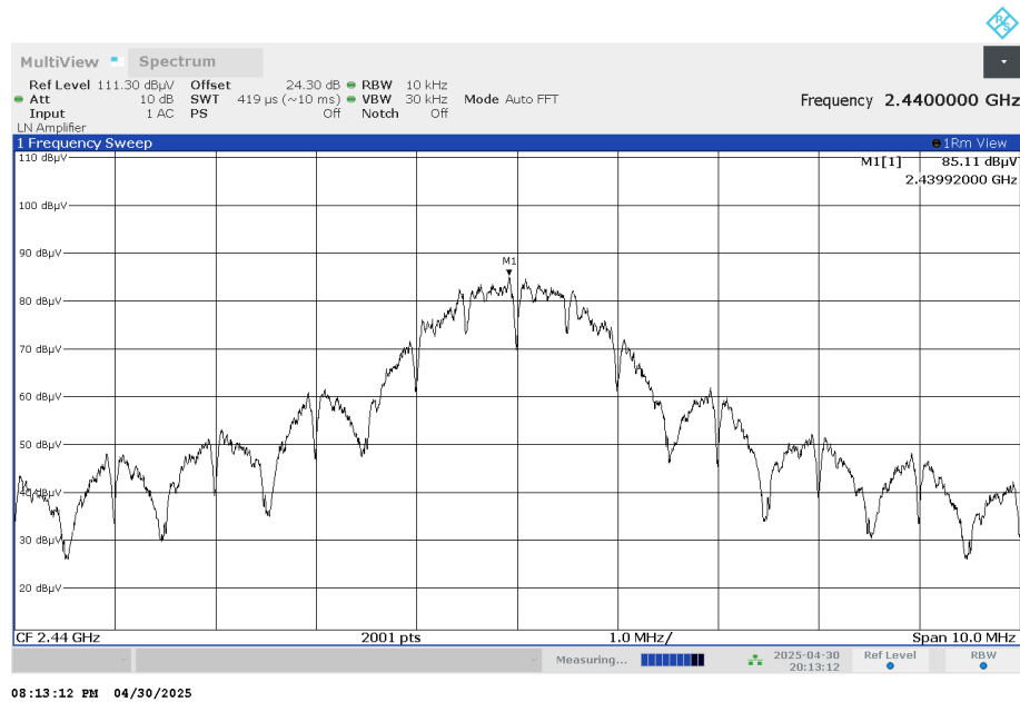
Power Spectral Density, Ch 18
