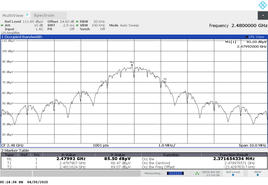
99% Bandwidth, Ch 26
