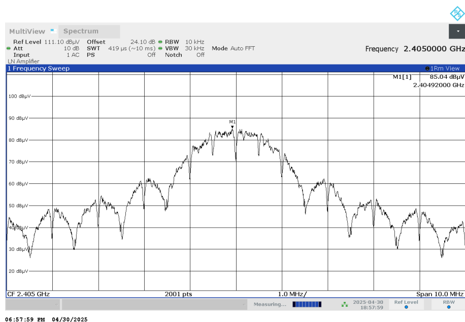
Power Spectral Density, Ch 11
