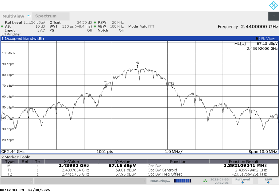
99% Bandwidth, Ch 18
