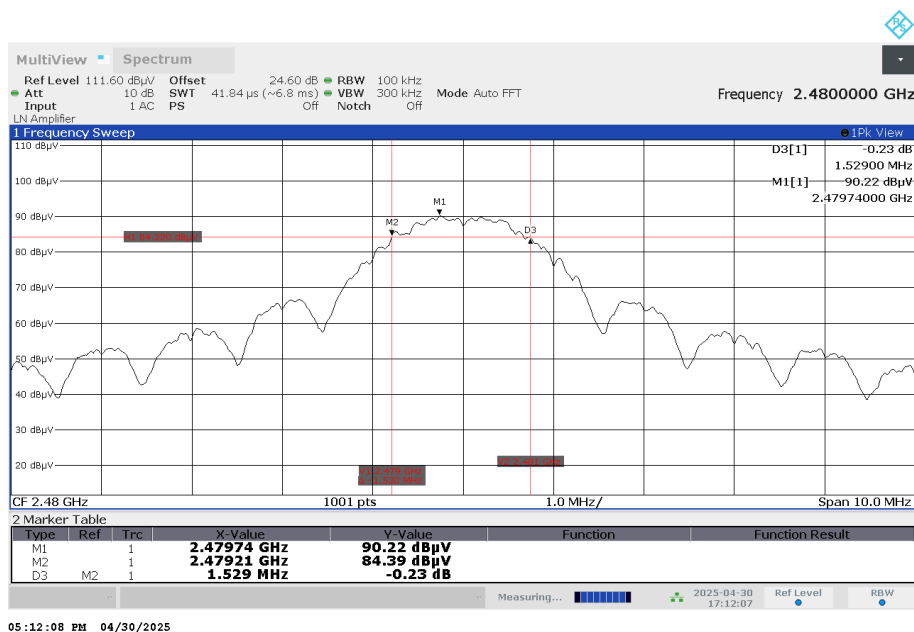
6 dB Bandwidth, Ch 26
