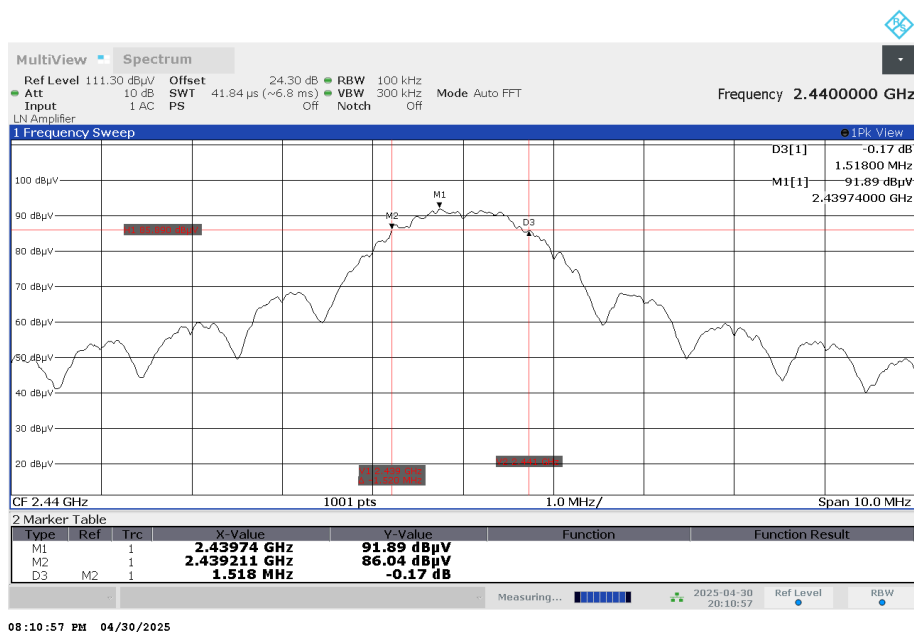
6 dB Bandwidth, Ch 18
