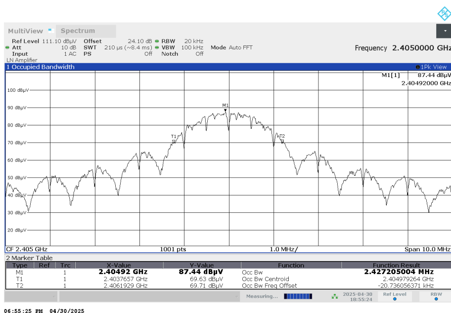
99% Bandwidth, Ch 11
