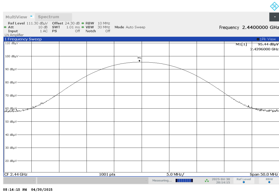
EIRP, Ch 18
