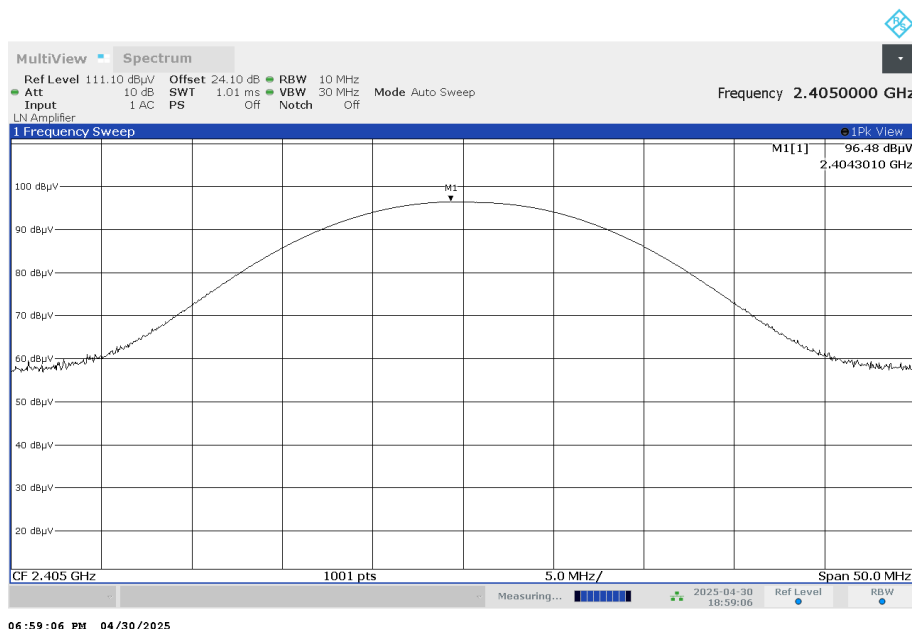
EIRP, Ch 11
