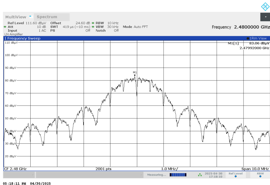
Power Spectral Density, Ch 26
