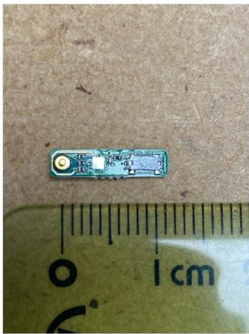
Buffer PCBA front
