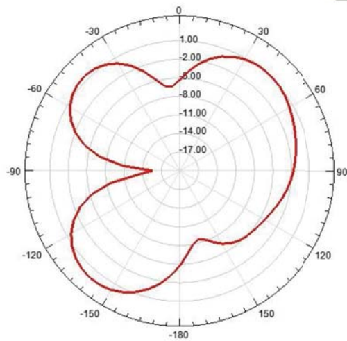
Radiation Pattern 2
