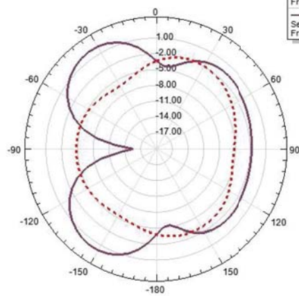
Radiation Pattern 2
