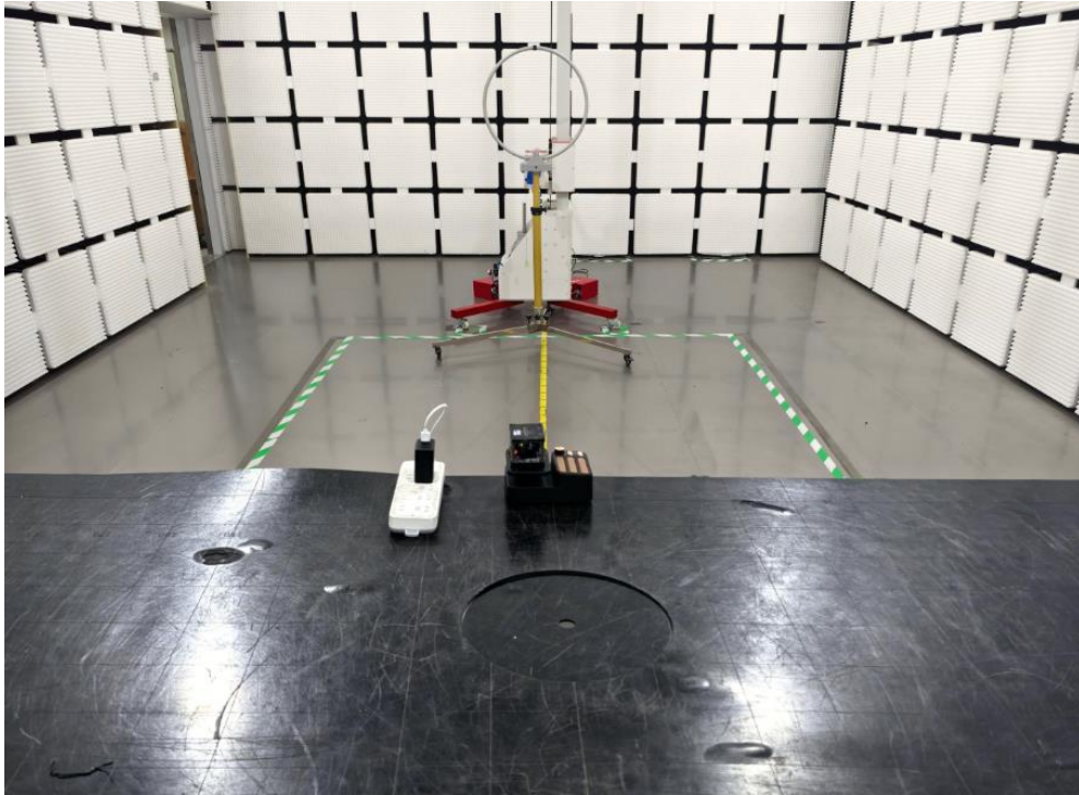
Spurious Radiation Emissions Test (9KHz-30MHz)
