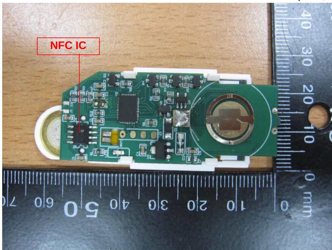
Figure 10 Internal View (PCB, Front View)
