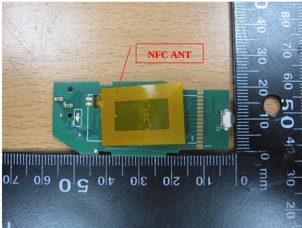
Figure 11 Internal View (PCB, Back View)
