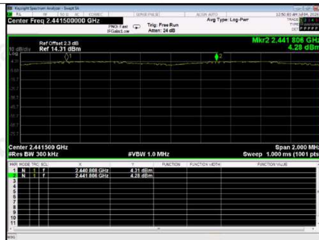
8-DPSK
