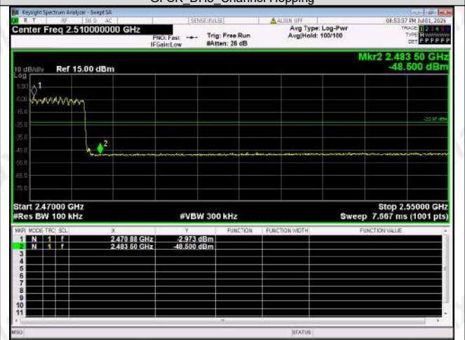
Out Of Band Emission(Right) π/4DQPSK_2-DH5_Channel Hopping
