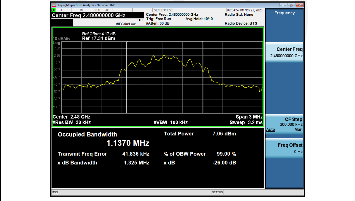
99%_Occupied_Bandwidth_NVNT_ANT1_2-DH1_2480_00
