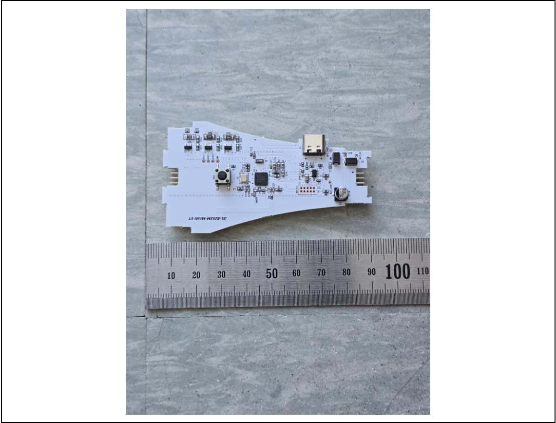
Board 1 Front
