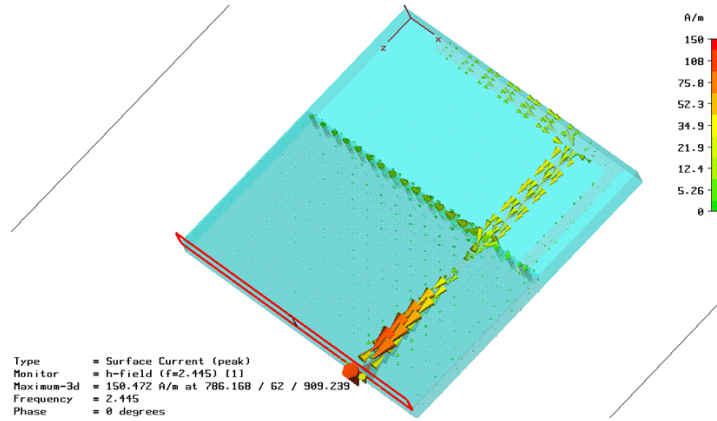
Figure 3.1. Surface Current
