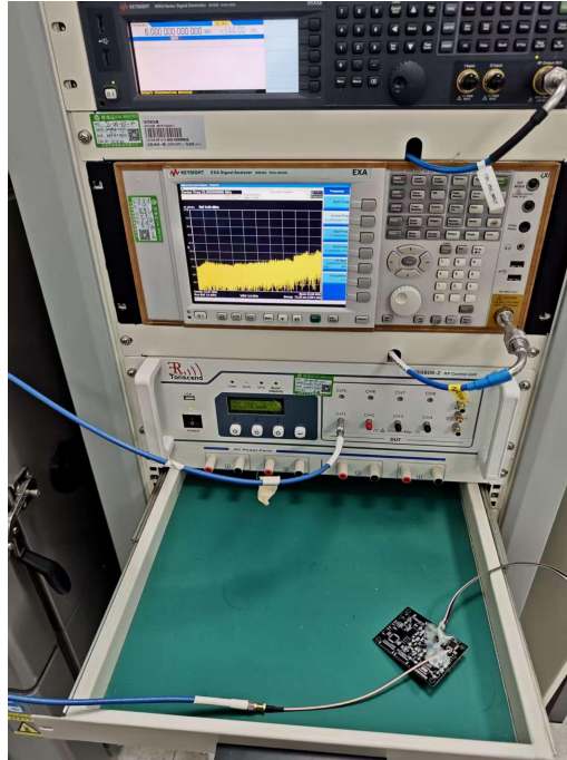
Conducted Emission View(BT Mode)
