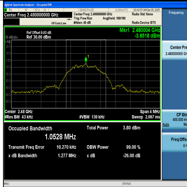
BLE_1M-Ant1-2480
