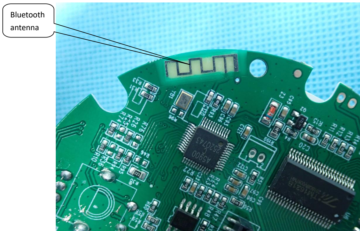
Internal Photo 6
