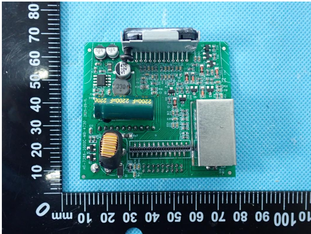
Internal Photo 9
