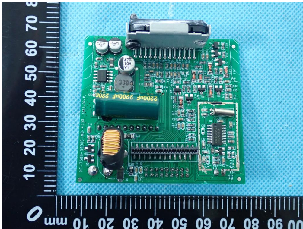
Internal Photo 11
