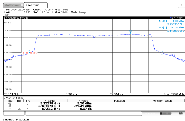
UNII 1 / 802.11ac VHT80 / Mid ch.
