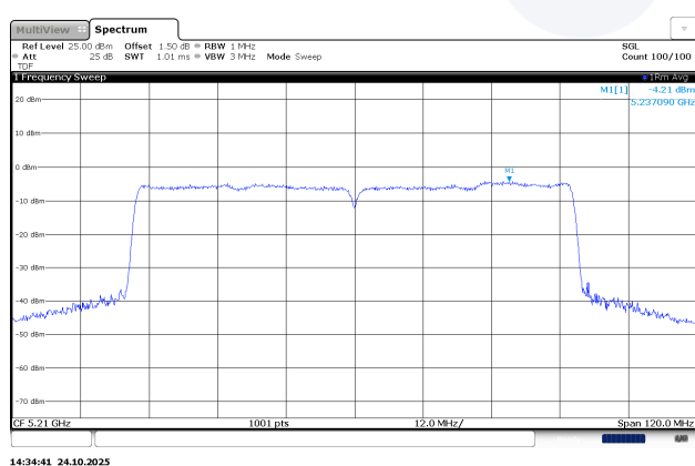
UNII 1 / 802.11ac VHT80 / Mid ch.
