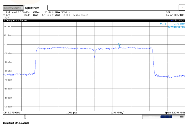
UNII 3 / 802.11ac VHT80 / Mid ch.
