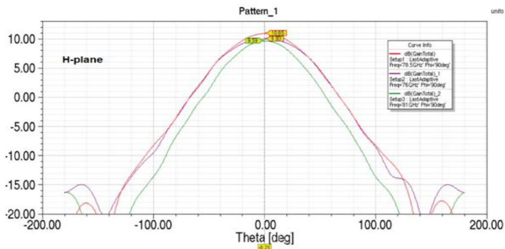
Figure 11. Antenna Pattern in H-Plane
