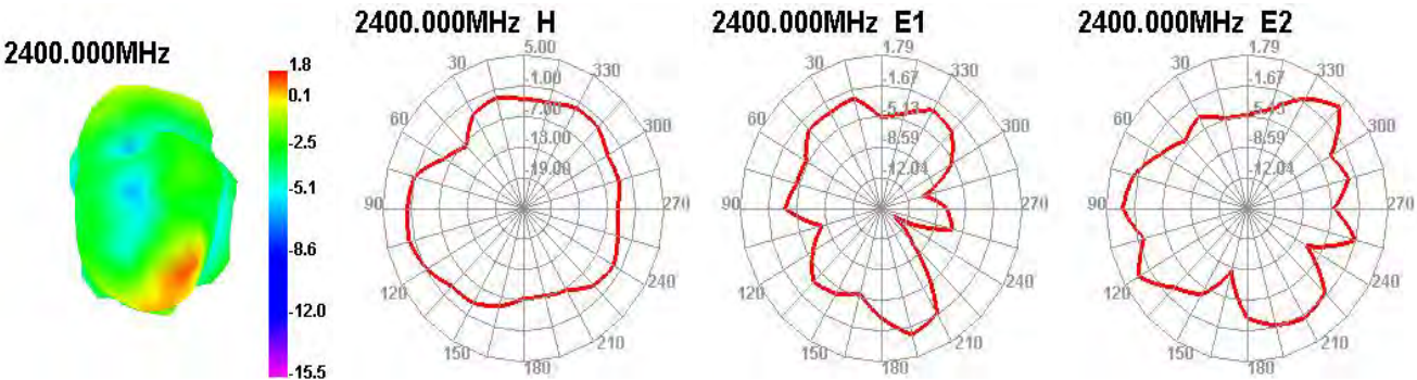
Radiation pattern.
