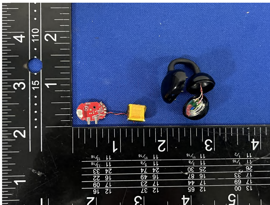
Right Earphones
