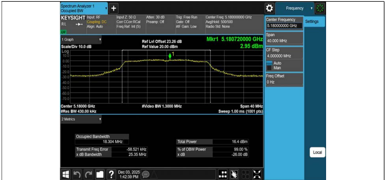
11N20MIMO-Ant1-5180
