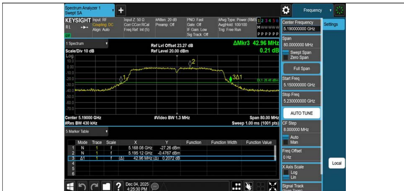
11AC40MIMO-Ant1-5190
