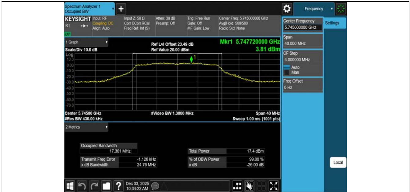
11A-CDD-Ant1-5745
