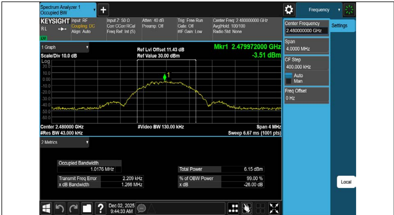
BLE_1M-Ant1-2480
