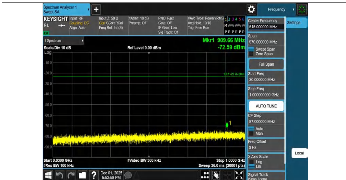
2DH5-Ant1-2480-30~1000-PASS
