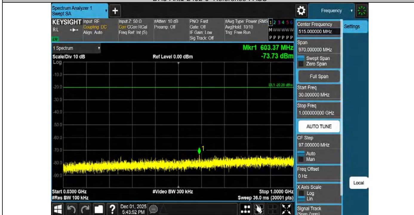
DH5-Ant1-2402-30~1000-PASS
