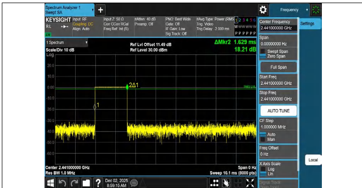
DH3-Ant1-Hop-PASS
