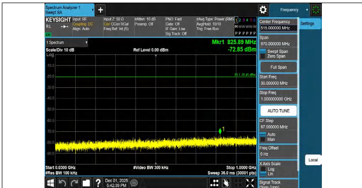
DH5-Ant1-2441-30~1000-PASS
