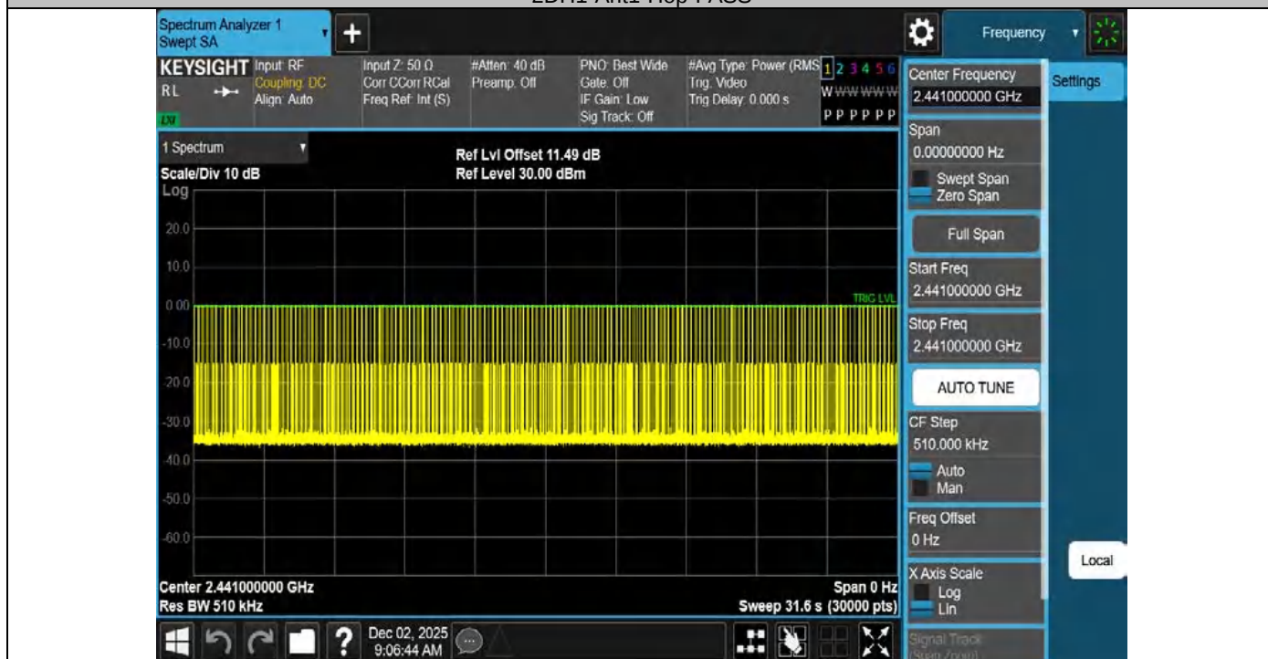
2DH1-Ant1-Hop-PASS
