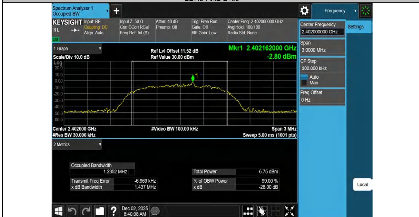
3DH5-Ant1-2402
