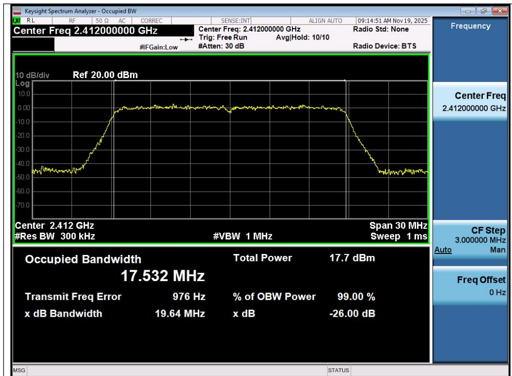
Test_Graph_802.11n20_Chain A_2412_MCS0_OBW
