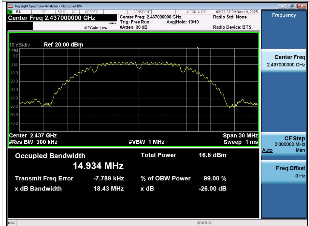
Test_Graph_802.11b_Chain B_2437_1Mbps_OBW
