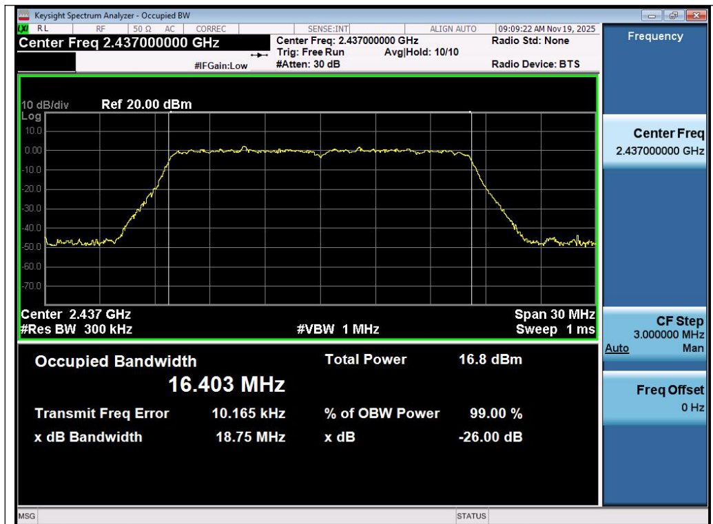
Test_Graph_802.11g_Chain A_2437_6Mbps_OBW
