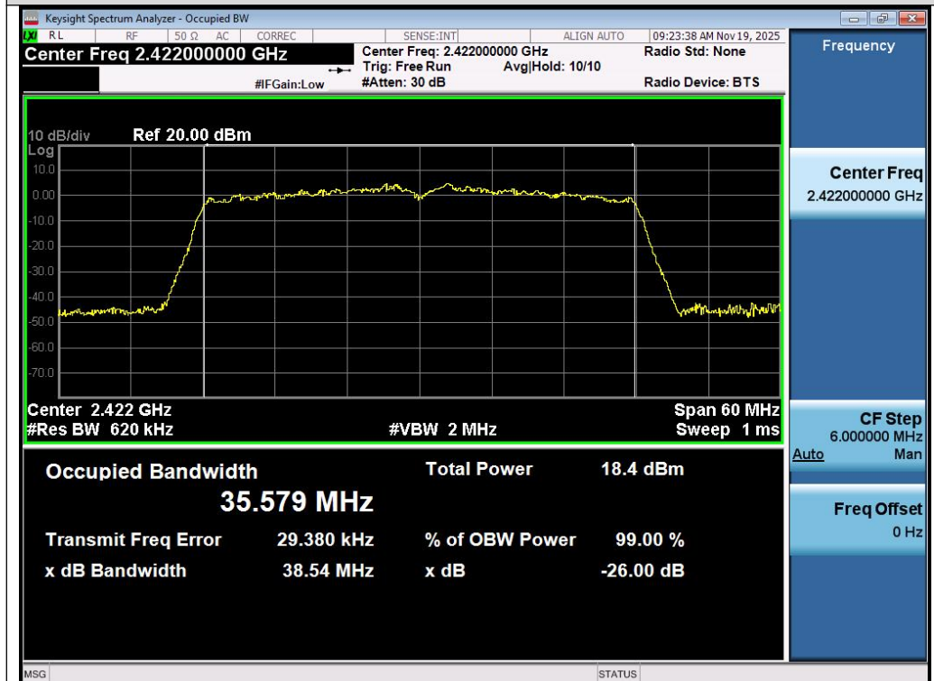
Test_Graph_802.11n40_Chain A_2422_MCS0_OBW
