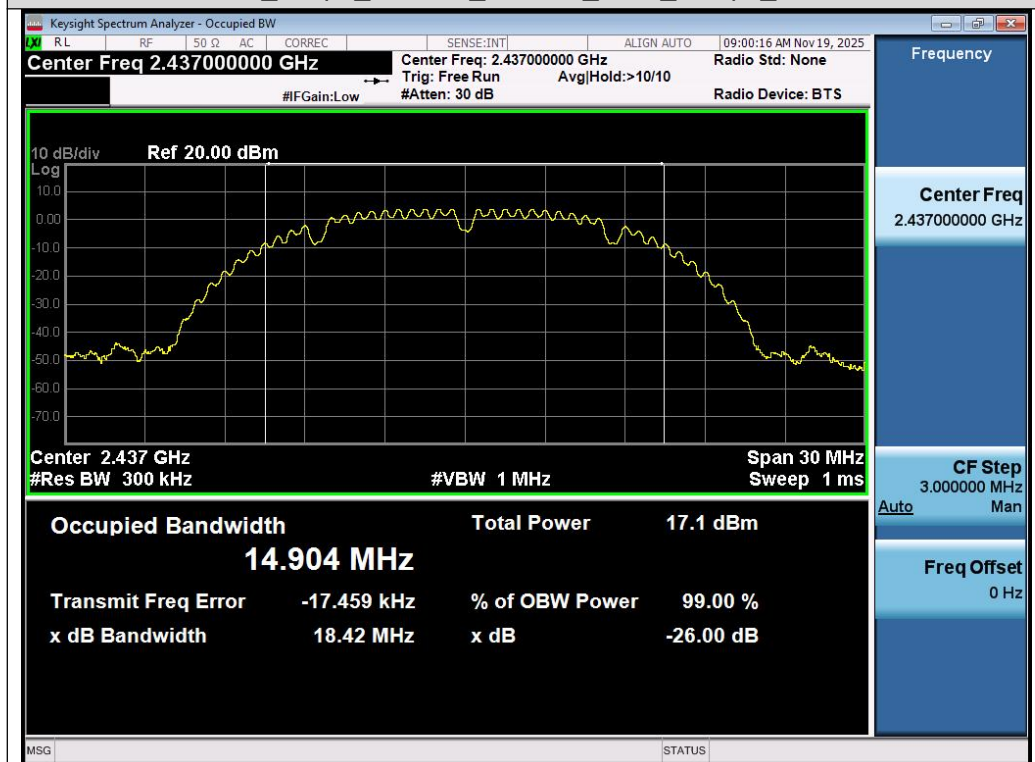
Test_Graph_802.11b_Chain A_2437_1Mbps_OBW
