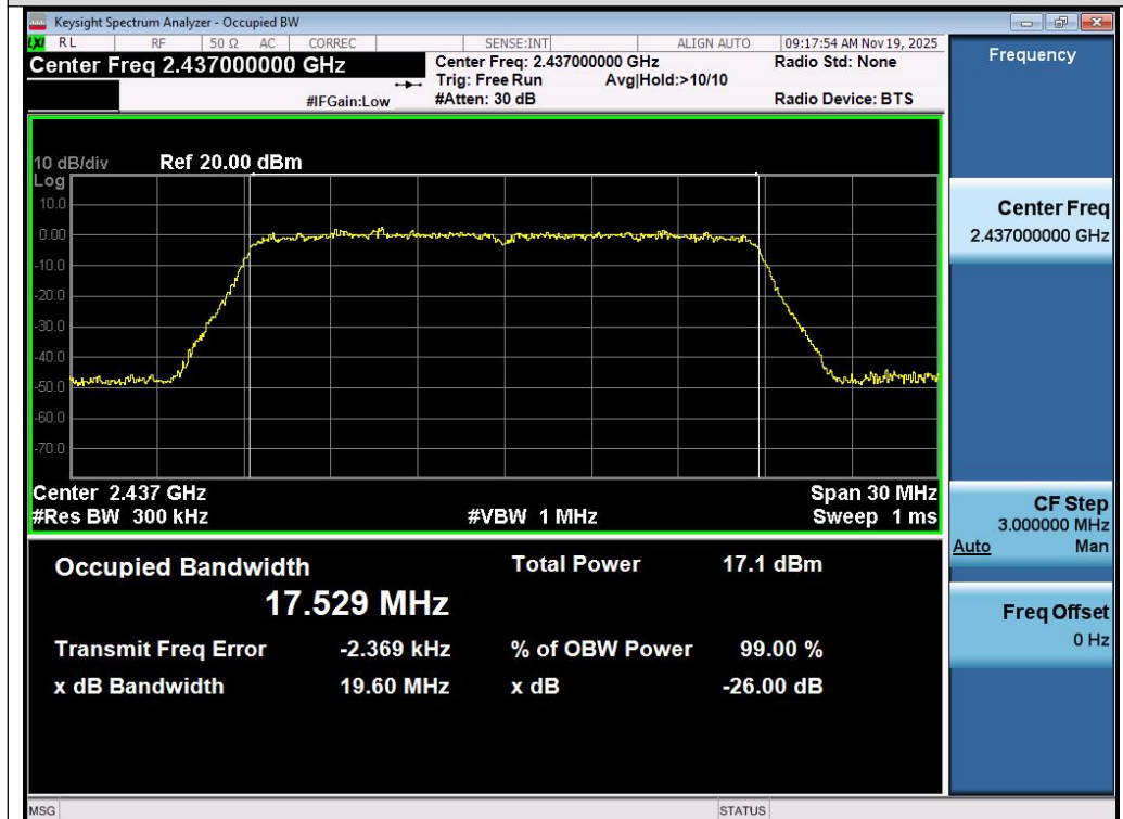
Test_Graph_802.11n20_Chain A_2437_MCS0_OBW
